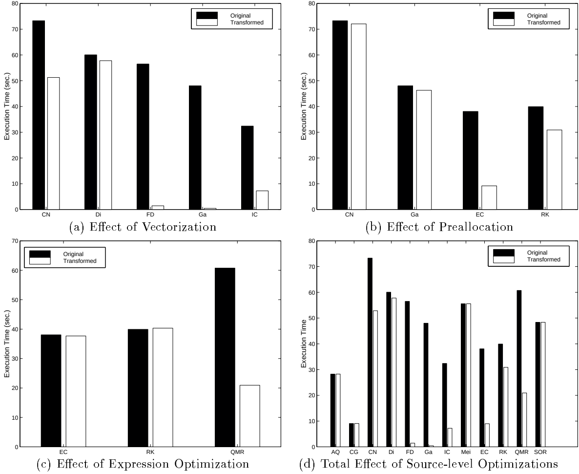
Figure 2: Source-to-Source Optimizations
