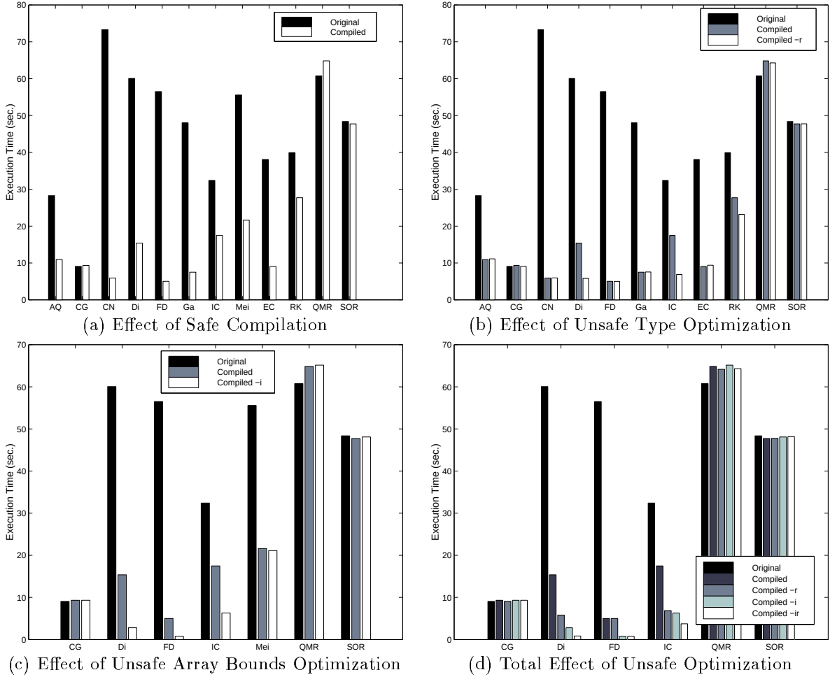
Figure 1: MCC Compilation
