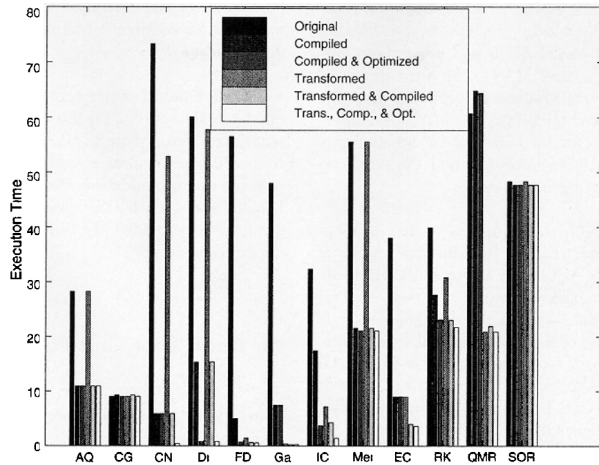
Figure 7: Source-Level Transformations and Compilation
