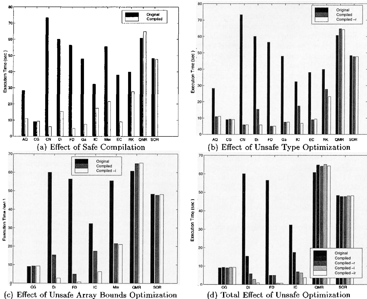
Figure 1: MCC Compilation
