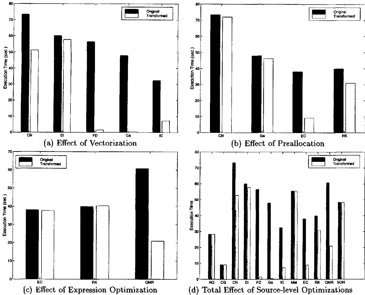
Figure 2: Source-to-Source Optimizations
