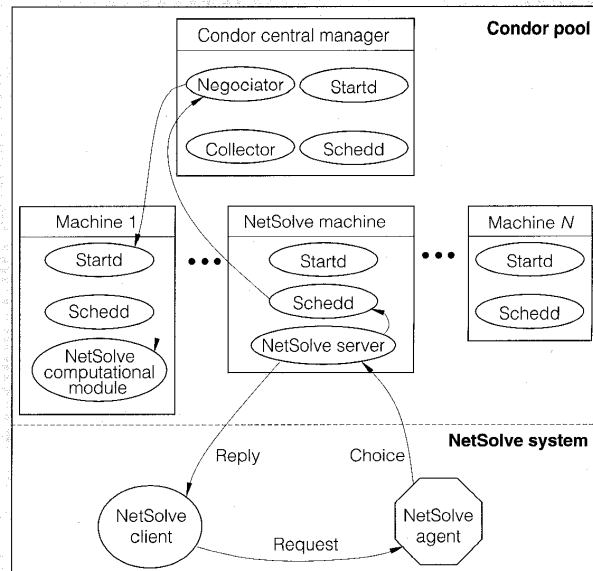
Figure A. NetSolve and Condor.
