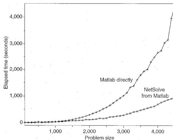
Figure 5. Using ScaLapack transparently from Matlab via NetSolve.
