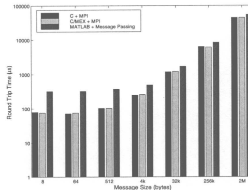
Figure 3: MultiMATLAB Round Trip Latencies on the IBM SP-2
