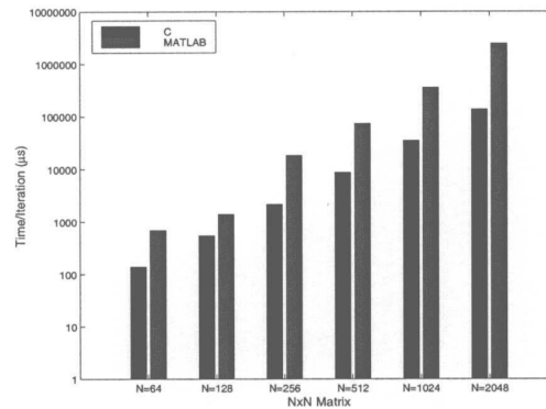
Figure 5: Sequential Conjugate Gradients on the IBM SP-2
