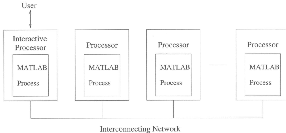
Figure 1: MultiMATLAB Architecture
