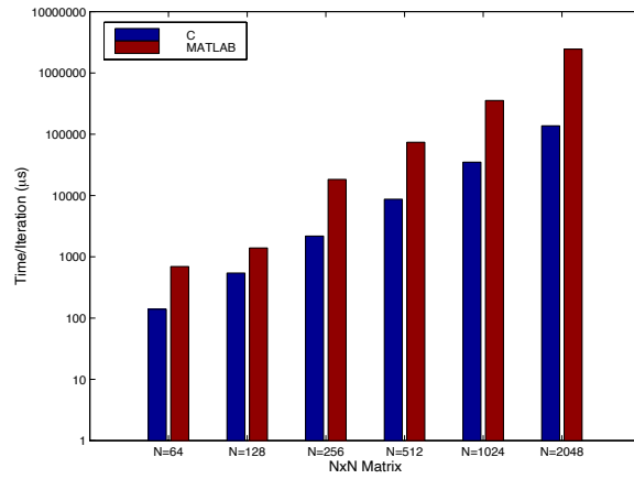
Figure 5: Sequential Conjugate Gradients on the IBM SP-2
