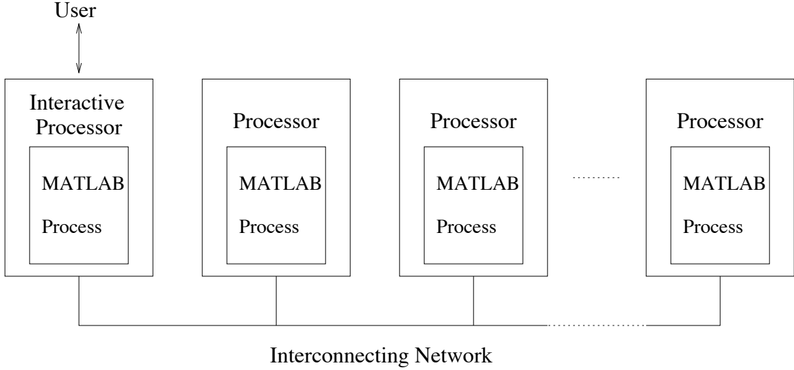
Figure 1: MultiMATLAB Architecture
