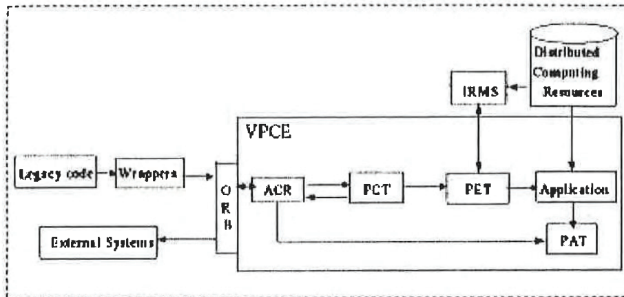
Fig. 1. The CB-PSE Architecture
