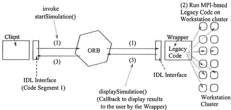
Fig. 4. The invocation sequences of the MDS-PSE
