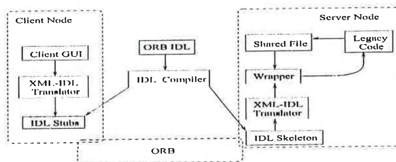
Fig. 2. The MDS-PSE Architecture
