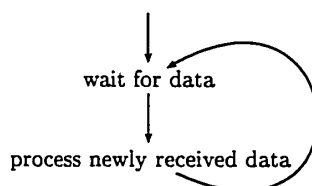
Figure 1.1: “Reader” Procedure
