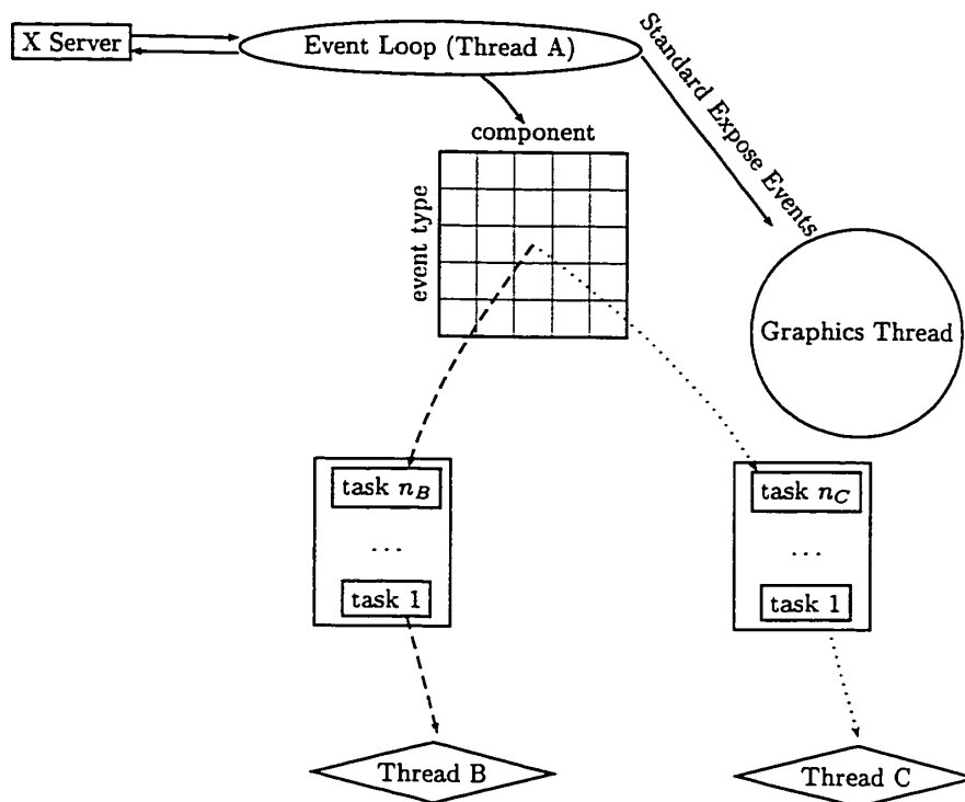
Figure 4.1: GUI Application Control Structure.
