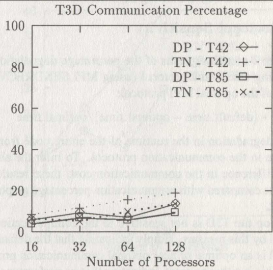
Figure 2. Communication percentages for fastest implementations
