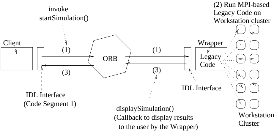
Fig. 4. The invocation sequences of the MDS-PSE
