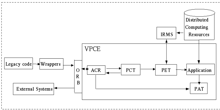
Fig. 1. The CB-PSE Architecture
