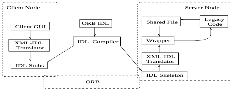
Fig. 2. The MDS-PSE Architecture
