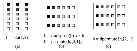
Figure 6. Permute and dpermute.
