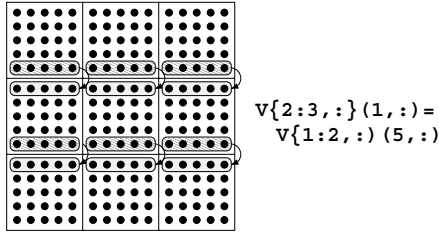
Figure 5. Assignment of all the elements in the last row of each one of the tiles located in the rows of tiles 1 and 2 to the first row of the corresponding tiles in the rows of tiles 2 and 3.
