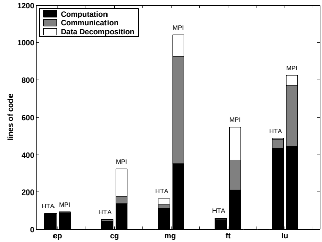
Figure 16. Linecount of key sections of HTA and MPI programs.
