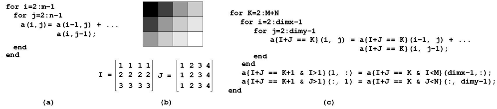
Figure 8: 2-D wavefront computation.(a) Fortran code. (b) Pictorial view. (c) HTA code.
