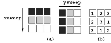
Figure 7: BT Benchmark. (a) Flow of Computation. (b) Processor Mapping.
