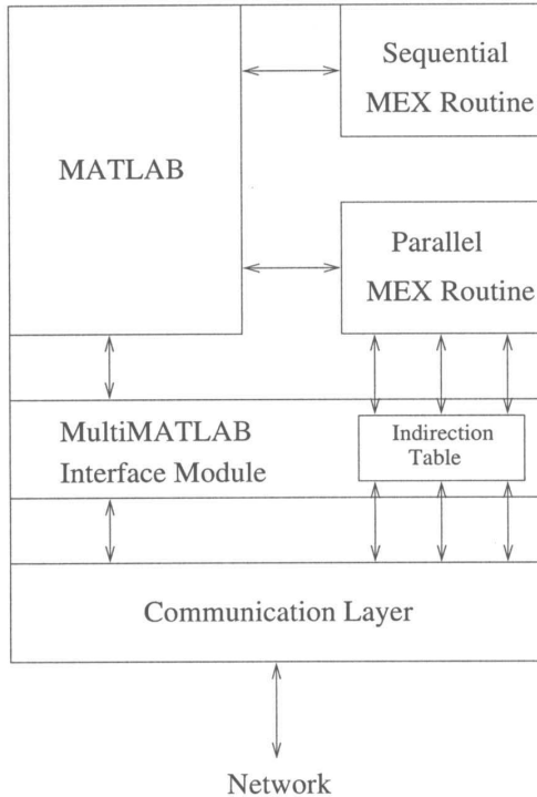
Figure 2: MATLAB Process Address Space
