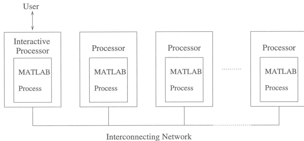
Figure 1: MultiMATLAB Architecture
