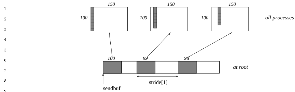
Figure 4.9: The root scatters blocks of 100-i ints into column i of a 100×150 C array. At the sending side, the blocks are stride[i] ints apart.
