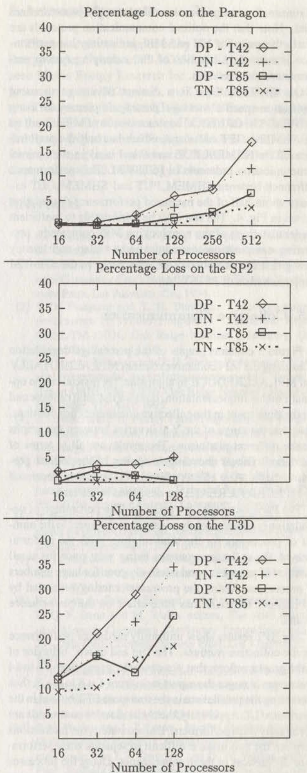
Figure 4. Performance Degradation from Using MPI Implementation
