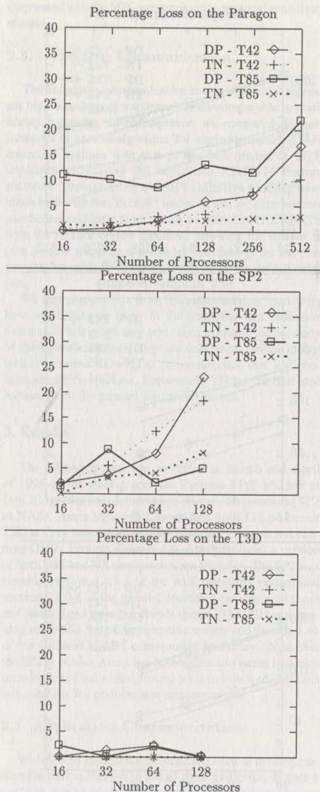
Figure 3. Performance Degradation from Using Default Protocol
