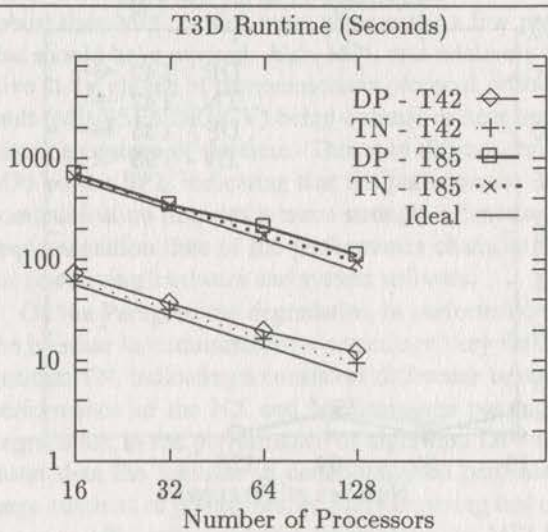
Figure 1. Runtimes for fastest implementations of PSTSWM.
