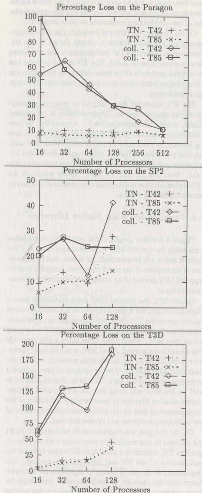
Figure 5. Performance Degradation from Using MPI Collective Communication Routines
