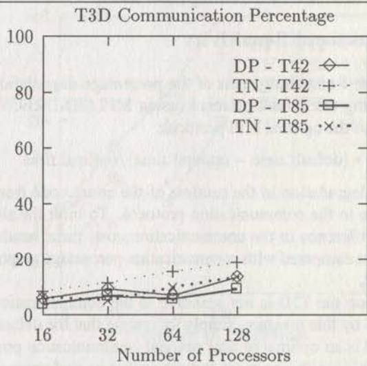
Figure 2. Communication percentages for fastest implementations
