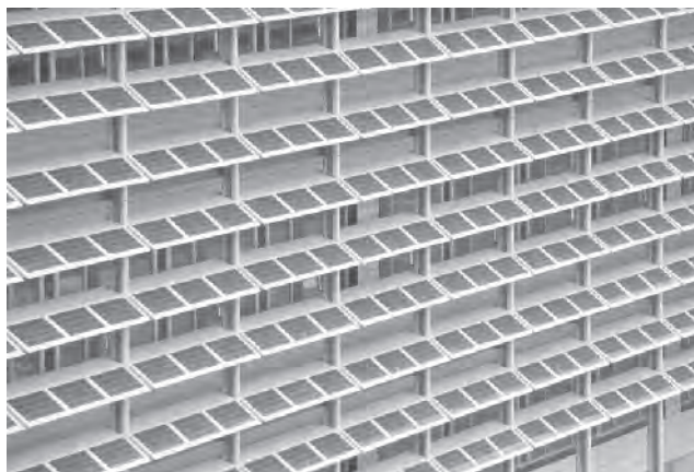
Figure 22.11 South facade of ECN Building 31 in Petten (NL). The shading structure supports the 35 kWp Shell Solar modules. Reproduced with permission by BEAR Architecten T. Reijenga
