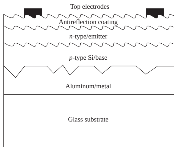
Figure 8.12 A sketch of the generic device structure used for cell design discussion
