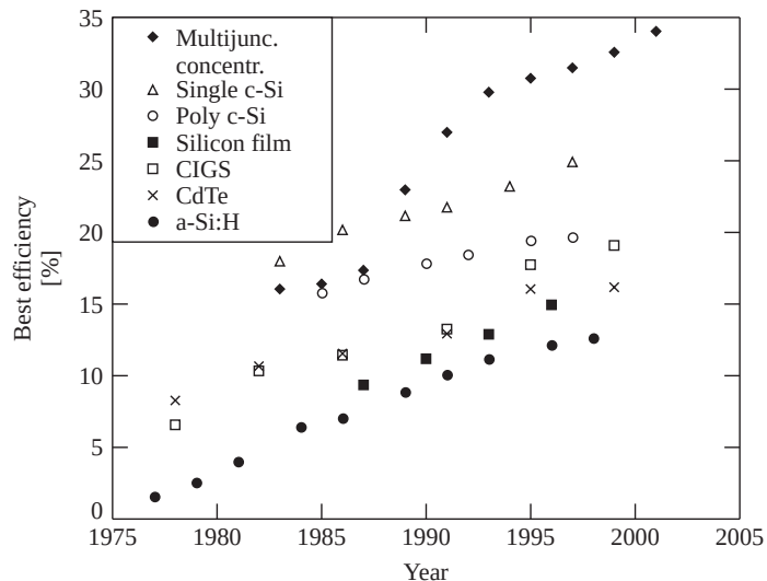
Figure 1.8 Best small area ( 0.5\text{--}5\text{ cm}^2 ) efficiency for various cell technologies measured under standard laboratory test conditions. MJ concentrators are double junctions before 1995, and triple junctions after. a-Si represents stabilized efficiency after extended light soaking and are MJ after 1990 (see Chapter 12)
