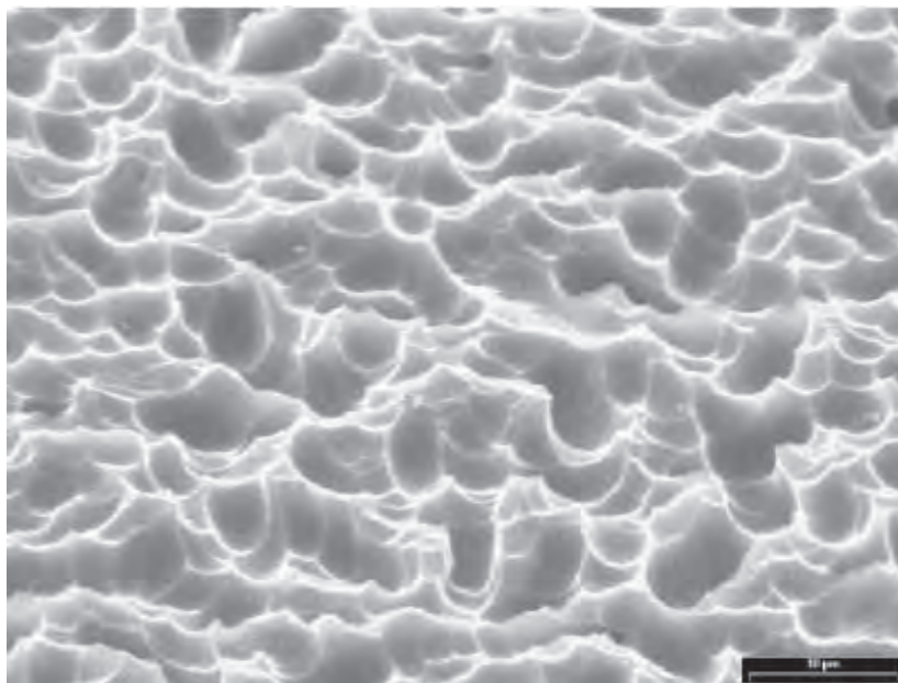
Figure 7.12 Mc-Si surface after acid etching. (Reprinted from Solar Energy Materials and Solar Cells , 74, Szulc J, Duerinckx F, Horzel J, Van Kerschaver E, Dekkers H, De Wolf S, Choulat P, Allebe C and Nijs J, “High-efficiency low-cost integral screen-printing multicrystalline silicon solar cells”, 155–164, (2002), with permission from Elsevier Science)
