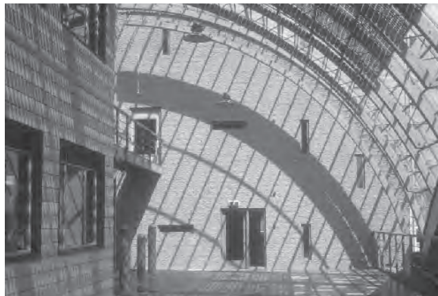
Figure 22.5 Interior view of the conservatory with integrated 43 kWp transparent BP solar modules in ECN Building 42 in Petten (NL). Reproduced with permission by BEAR Architecten T. Reijenga
