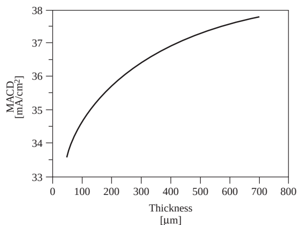
Figure 8.1 Maximum achievable current density (MACD) from a planar, AR-coated Si solar cell as a function of cell thickness. These calculations assume an optimized AR coating and AM1.5 incident spectrum. These results are obtained with PV Optics
