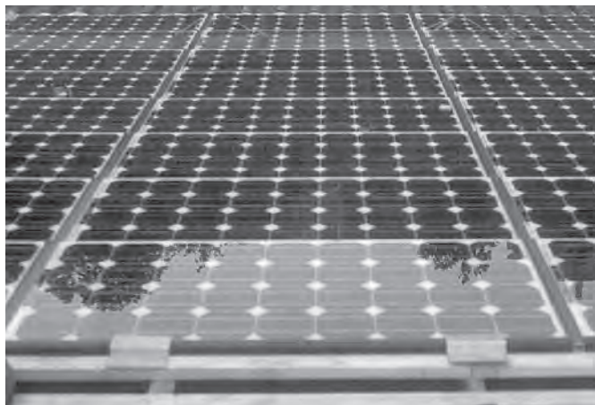
Figure 22.35 Solrif Solar profile system in a roof renovation in Zurich (CH). Capacity of the system is 53 kWp. Reproduced with permission by BEAR Architecten T. Reijenga
