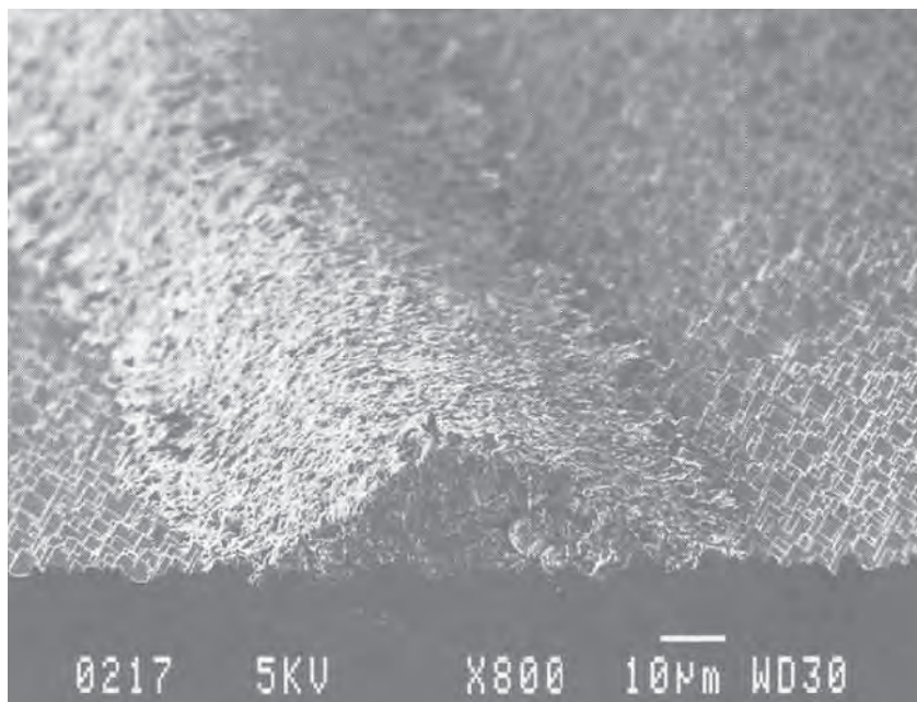
Figure 7.10 Screen-printed contact finger; texture pyramids are also visible. (Reprinted from Solar Energy Materials and Solar Cells , 41/42, Nijs J, Demesmaeker E, Szulc J, Poortmans J, Frisson L, De Clerq K, Ghannam M, Mertens R, Van Overstraeten R, “Recent improvements in the screen-printing technology and comparison with the buried contact technology by 2D-simulation”, 101–107, (1997), with permission from Elsevier Science)
