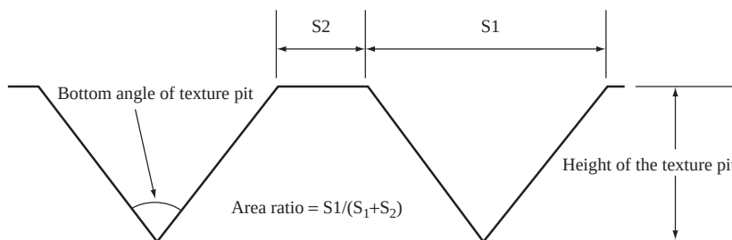
Figure 8.17 The geometry and the terminology used in the texture shape study [19]
