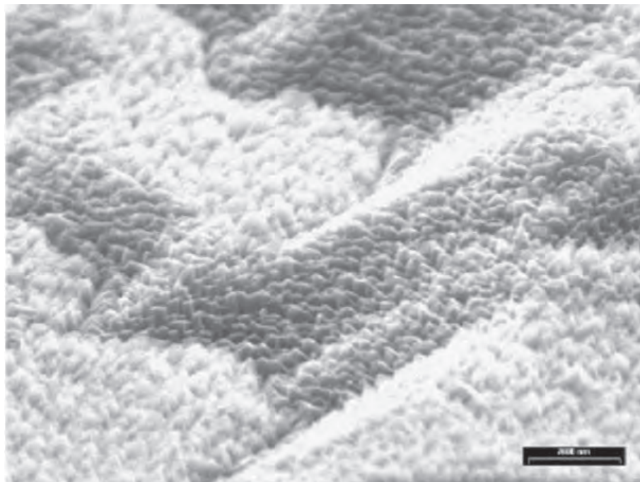
Figure 7.13 mc-Si surface after RIE. (Reprinted from Solar Energy Materials and Solar Cells , 74, Szulfcik J, Duerinckx F, Horzel J, Van Kerschaver E, Dekkers H, De Wolf S, Choulal P, Allebe C and Nijis J, “High-efficiency low-cost integral screen-printing multicrystalline silicon solar cells”, 155–164, (2002), with permission from Elsevier Science)
