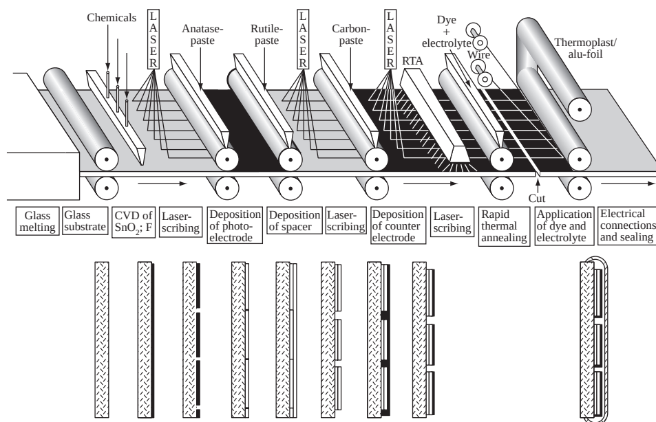
Figure 15.16 Continuous process for the fabrication of monolithic series-connected DSSC modules. Reprinted from Sol. Energy Mater. Sol. Cells , 44, Kay A, Gratzel M, 99–117, © (2002), with permission from Elsevier Science
