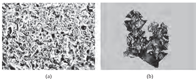
Figure 6.17 Optical micrograph of the surface of an as-cut silicon wafer (a) and several micro-indentations on a polished silicon surface (b)
