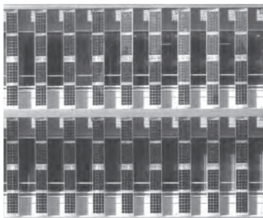
Figure 22.6 Solar shading (PV modules as part of a vertical louver system) on the west facade of the SBIC office building in Tokyo (JA). The transparent vertical louvers, with a total capacity of 20.1 kWp, were manufactured by Atlantis Switzerland. Reproduced with permission by Jiro Ono
