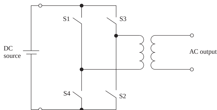
Figure 19.22 H-bridge-type inverter
