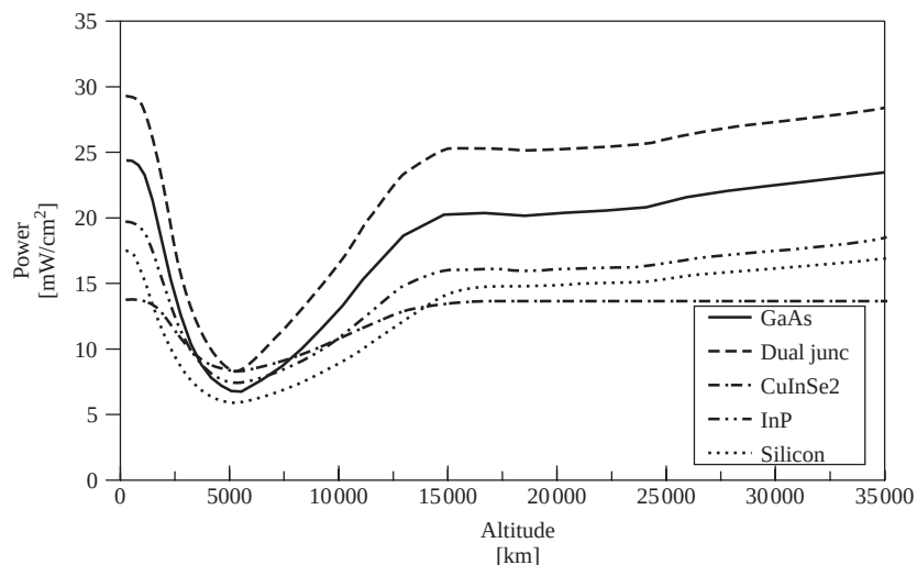
Figure 10.4 Solar cell power density as a function of altitude after 10 years in a 60° orbit with a cover glass thickness of 300 \mu\text{m} (GaAs: BOL 24.4 (mW/cm 2 ) [27]; Dual Junc – GaInP/GaAs/Ge [28]: BOL 29.3 (mW/cm 2 ); CuInSe2: BOL 14.4 (mW/cm 2 ) [29]; InP: BOL 19.7 (mW/cm 2 ) [30]; Si: BOL 17.5 (mW/cm 2 ) [31]). (Graph courtesy of Tom Morton, Ohio Aerospace Institute)
