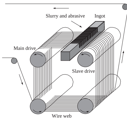
Figure 6.15 Schematic diagram depicting the principle of the multi-wire sawing technique
