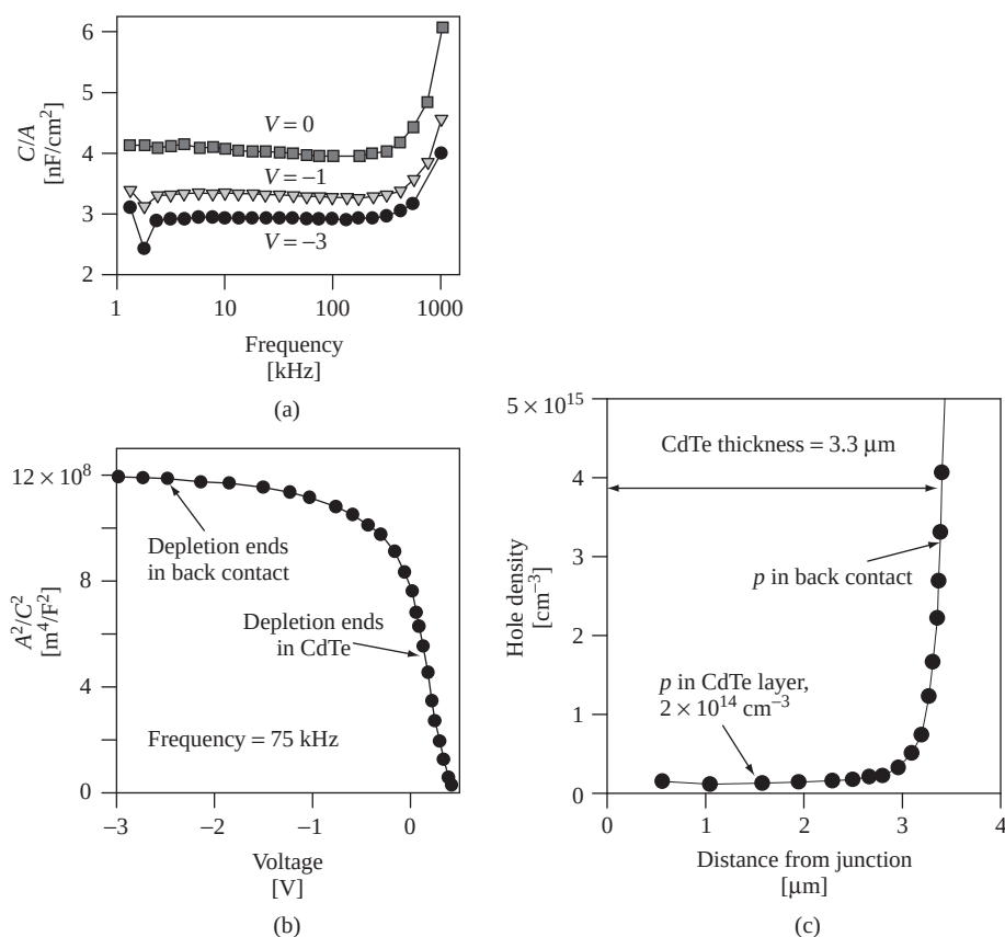
Figure 14.25 Capacitance measurements and hole-density determination for a CdTe solar cell
