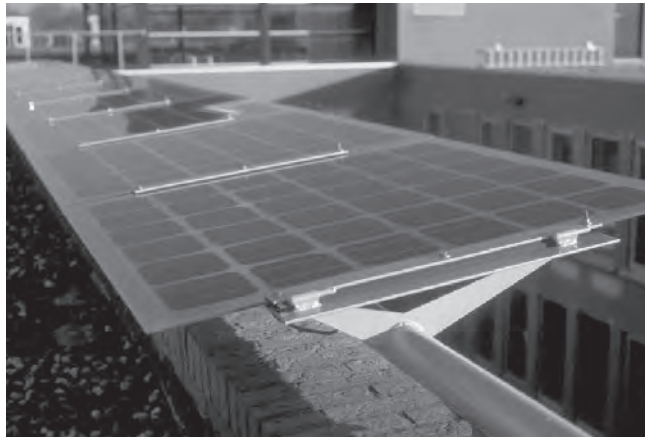
Figure 22.42 Canopy at the eaves of a roof. 6.2 kWp PV system at an office building in Gouda (NL). Reproduced with permission by BEAR Architecten T. Reijenga
