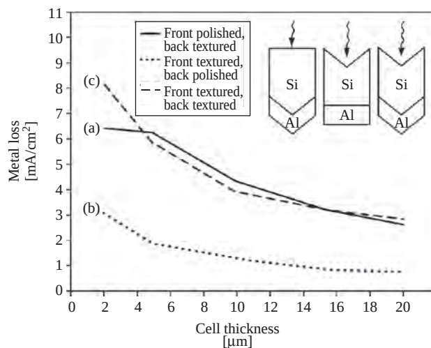
Figure 8.14 Metal loss due to absorption by an Al back-reflector as a function of thickness for three different cell structures. Texture height was 1.0 µm
