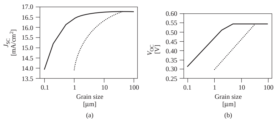
Figure 8.24 Calculated dependence of (a) J_{SC} ; and (b) V_{OC} on the grain size of the 10-μm-thick cell for two values of interface recombination velocity, 100 cm/s (solid lines) and 1000 cm/s (dotted lines)
