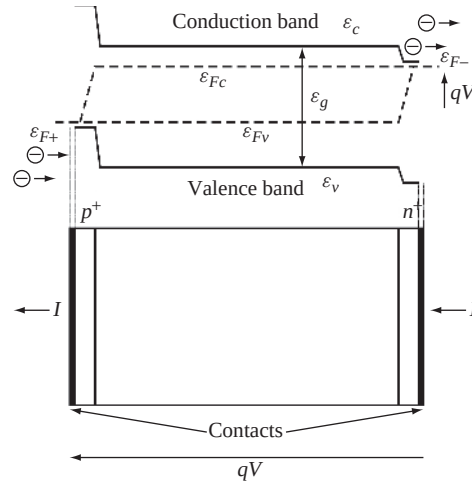
Figure 4.2 Band diagram of a solar cell with its contacts
