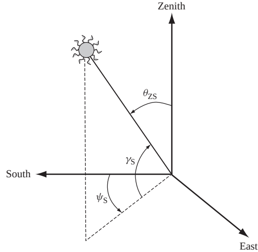
Figure 20.5 Position of the sun relative to a fixed point on the Earth
