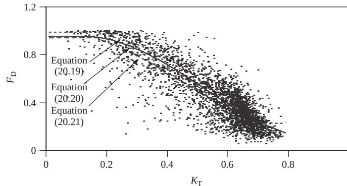
Figure 20.12 The diffuse fraction of the individual daily global irradiation F_{Dd} is plotted against the clearness index K_{Td} . The cluster of points refers to measured values in Madrid from 1977 to 1988
