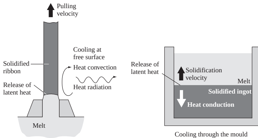
Figure 6.28 Scheme of thermal effects during ribbon growth and ingot crystallisation
