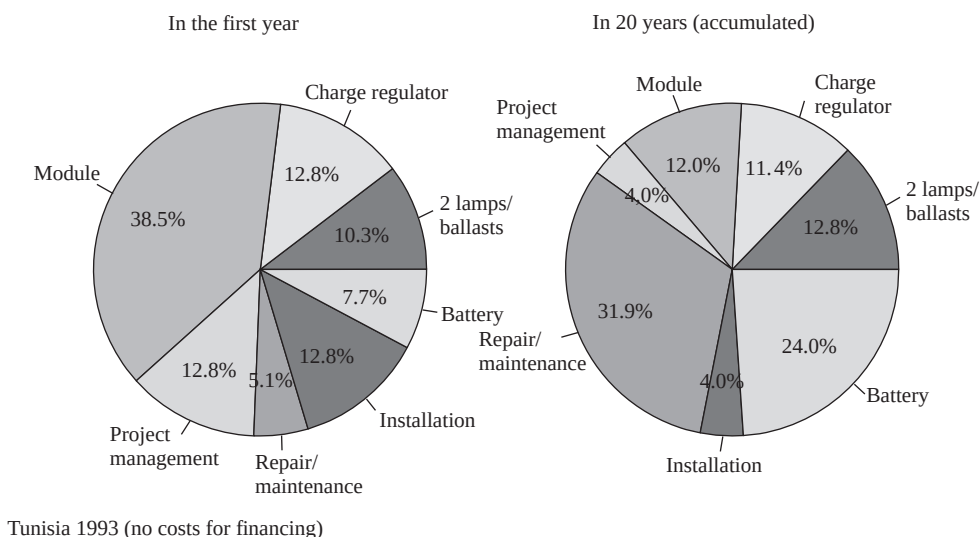
Figure 17.19 Cost breakdown for Solar Home Systems [7]: (a) year of installation; (b) cumulative costs after 20 years of lifetime
