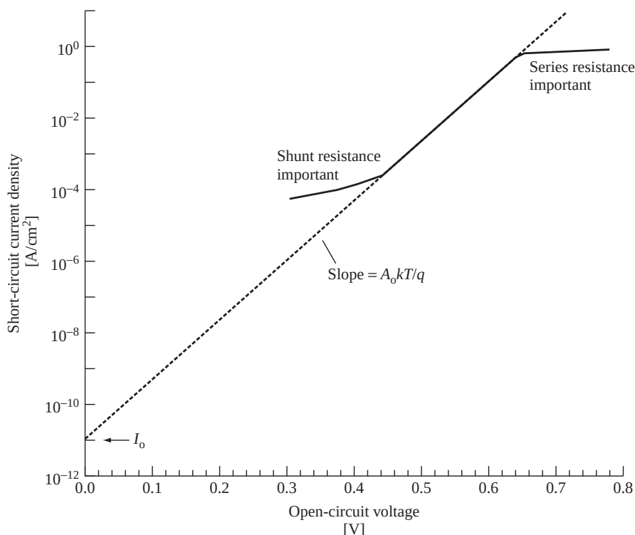
Figure 3.24 Short-circuit current versus open-circuit voltage plot illustrating parameter extraction
