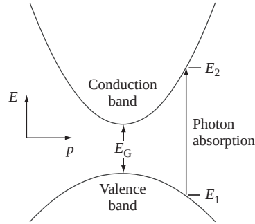
Figure 3.6 Photon absorption in a direct band gap semiconductor for an incident photon with energy h\nu = E_2 - E_1 > E_G
