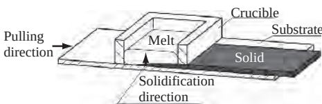
Figure 6.32 Scheme of the RGS process. The latent heat is removed through the substrate. By this, solidification is propagated vertical to the substrate and is de-coupled from substrates' pulling direction
