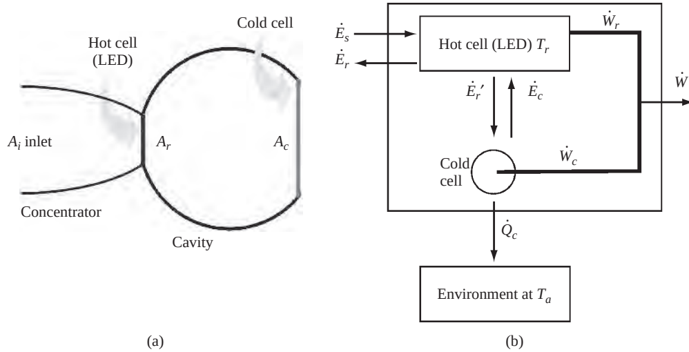
Figure 4.9 Diagram of the TPH converter with cavity. In (b), the energy fluxes are given by \dot{E}_s \equiv E(T_s, 0, 0, \infty, H_{rs}) , \dot{E}_r \equiv E(T_r, qV_r, 0, \infty, H_{rs}) , \dot{Q}_r = \dot{E}_s - \dot{E}_r , \dot{E}_r' \equiv E(T_r, qV_r, 0, \infty, H_{rc}) , \dot{E}_c' \equiv E(T_a, qV_c, \varepsilon_g, \infty, H_{rc})
