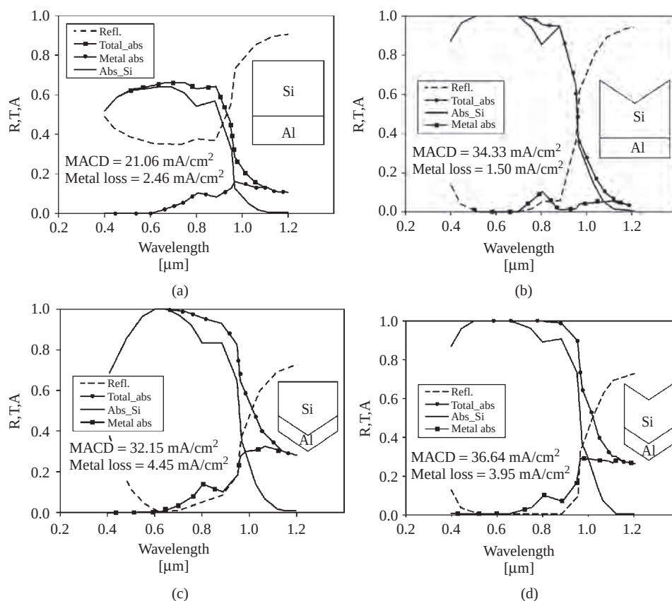
Figure 8.13 a–d Calculated reflectance (R), transmittance (T), and absorbance (A) of a single-junction cell under different surface configurations. The cell structures are shown in the inset of the figures. Absorber thickness = 10 \mu\text{m} . (a) Planar, (b) FTBP, (c) FPBT, and (d) DT
