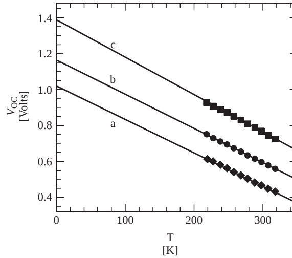
Figure 13.18 Temperature dependence of V_{OC} for the devices shown in Figure 13.16
