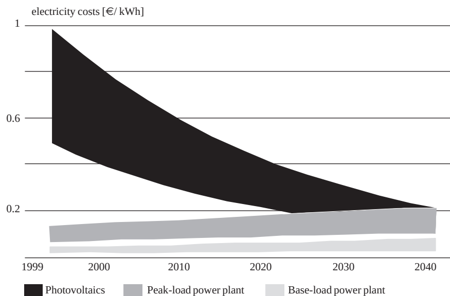
Figure 2.5 Cost projections for photovoltaic electricity. The upper boundary of photovoltaic costs reflects the meteorological situation of Germany, the lower boundary that of Southern Europe [8]
