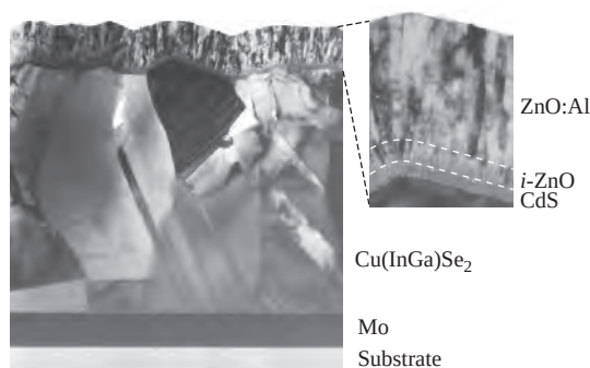
Figure 13.2 TEM cross section of a Cu(InGa)Se 2 solar cell
