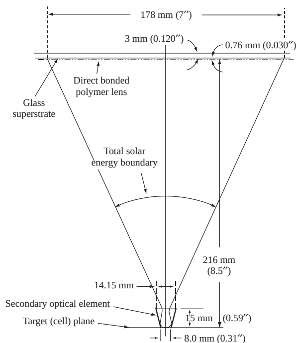
Figure 11.31 Lens cell configuration for a Fresnel lens with v-trough secondary [30]. Copyright © 1984, Electric Power Research Institute. AP-3263. Conceptual Design for a High-Concentration 500X Photovoltaic Array . Reprinted with permission
