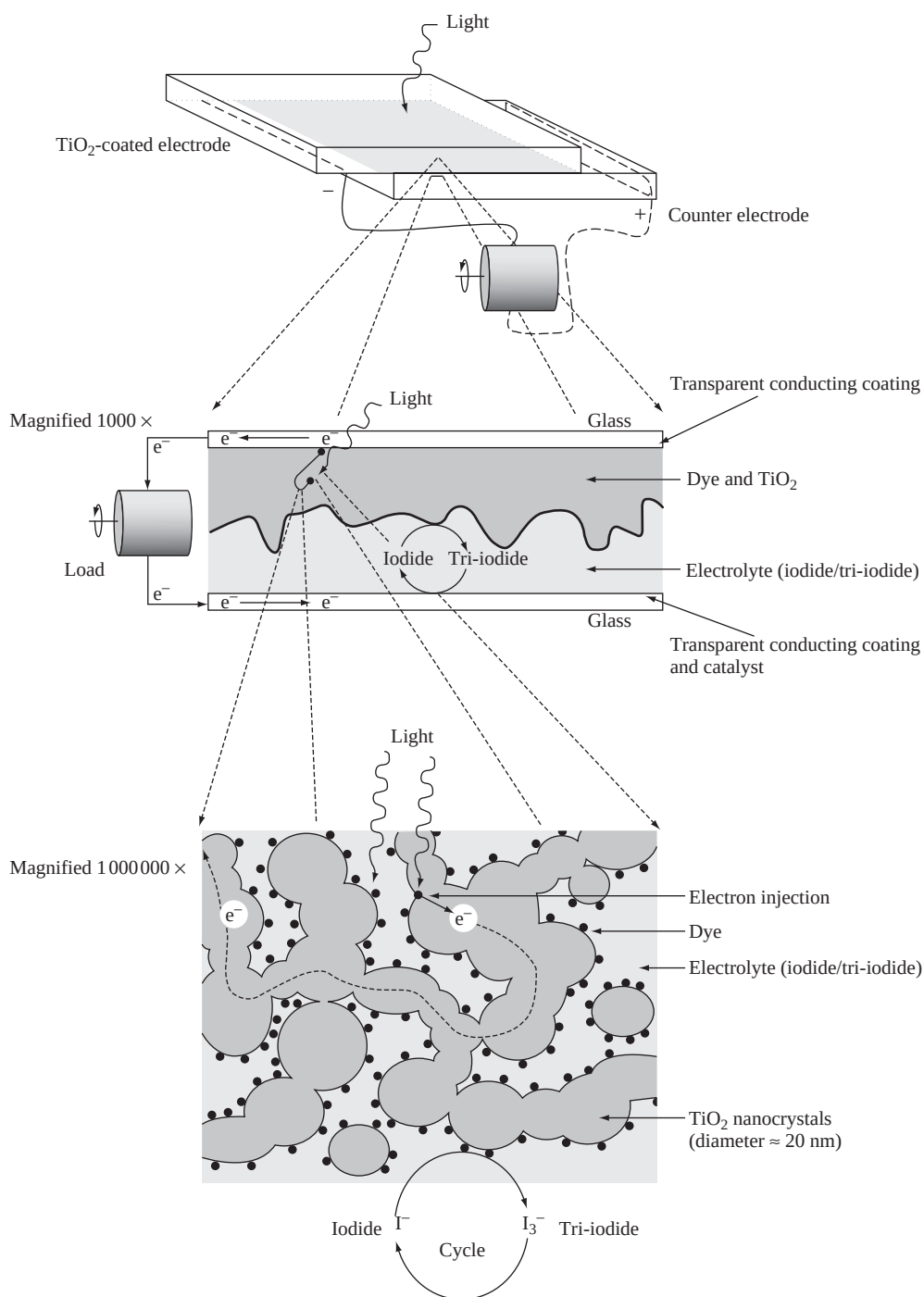
Figure 15.1 Schematic structure of the nanocrystalline dye-sensitized solar cell (DSSC). Reprinted from Sol. Energy Mater. Sol. Cells , 55, Smestad G, 157–178, © 2002, with permission from Elsevier Science [15]
