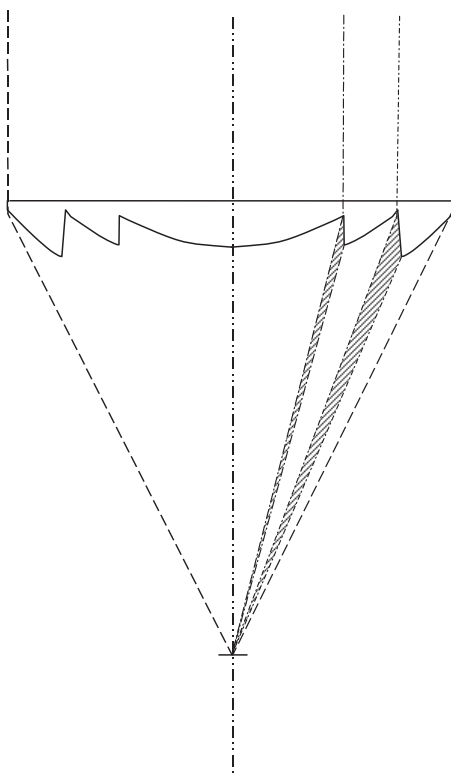
Figure 11.29 Cross section of a Fresnel lens
