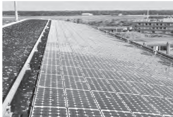
Figure 22.33 BP Sunflower system at the bent roof at ECN building 31, Petten (NL). Capacity 35 kWp. Reproduced with permission by BEAR Architecten H. Lieveerse
