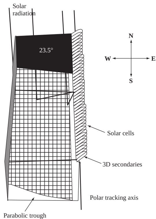
Figure 11.17 A two-stage concentrator permitting 300X concentration with one-axis tracking. Reprinted from Sol. Energy , 56, Brunotte M, Goetzberger A, Blieske U, 285–300, © (2002), with permission from Elsevier Science
