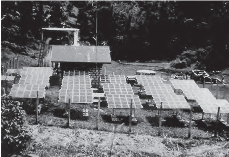
Figure 17.16 Photovoltaically powered system to provide drinking water for 4000 people (Source: TUV Rheinland, Cologne)
