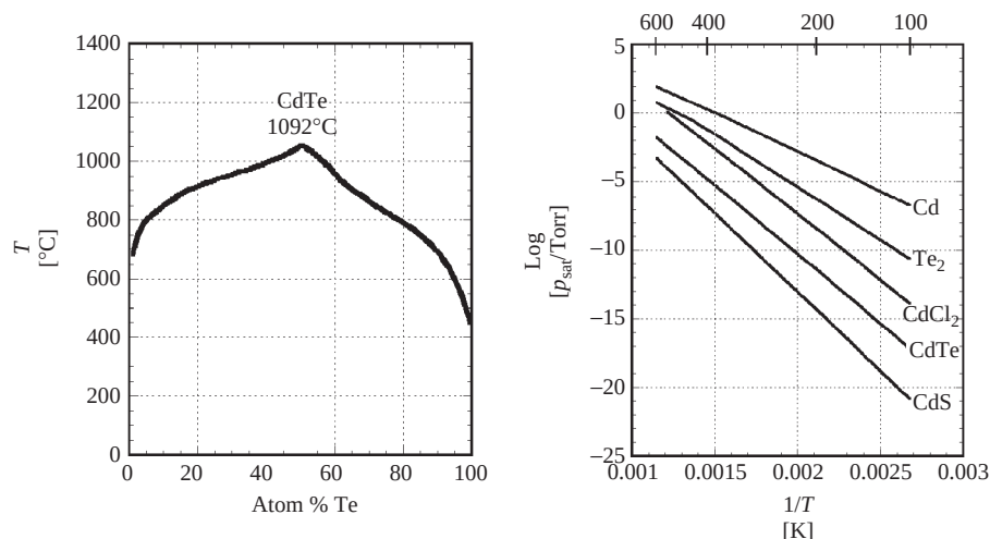
Figure 14.3 (a) CdTe T \times phase diagram (1 atm) [47] and (b) vapor–solid p_{\text{sat}} versus 1/T diagram for CdTe, CdS, \text{CdCl}_2 , Cd, and Te [48]
