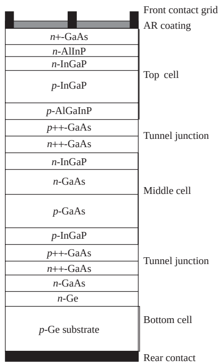
Figure 10.8 Commercially available 26.9% GaInP/GaAs/Ge triple-junction cell
