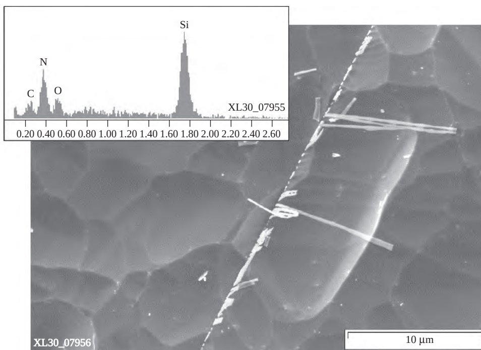
Figure 6.12 SEM (Scanning Electron Microscope) image of a heavily shunted solar cell region. The microscopic investigations reveal needle-shaped structures containing silicon, nitrogen, oxygen and carbon. The shunting mechanism is assumed to be due to electrically conductive SiC that short-circuits the solar cell pn -junction
