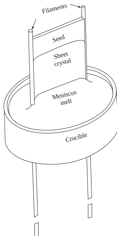
Figure 6.24 Schematic of String Ribbon (STR) growth system
