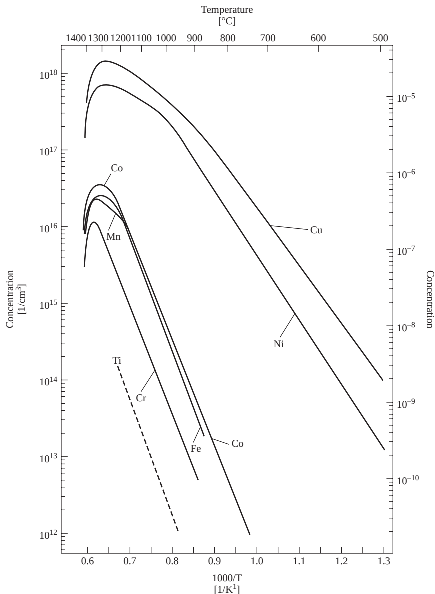
Figure 5.10 Solid solubility of 3d transition elements in silicon. Sc is still missing, but is assumed to be a little below the values of Ti. Adapted from J. Appl. Phys. Weber E, A30, 1–22 1983, © Springer-Verlag GmbH & Co. KG. The values for Ti are taken from [37]
