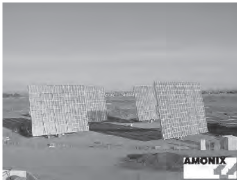
Figure 11.38 Amonix 100-kW high-concentration Fresnel lens array at the Glendale, California Airport
