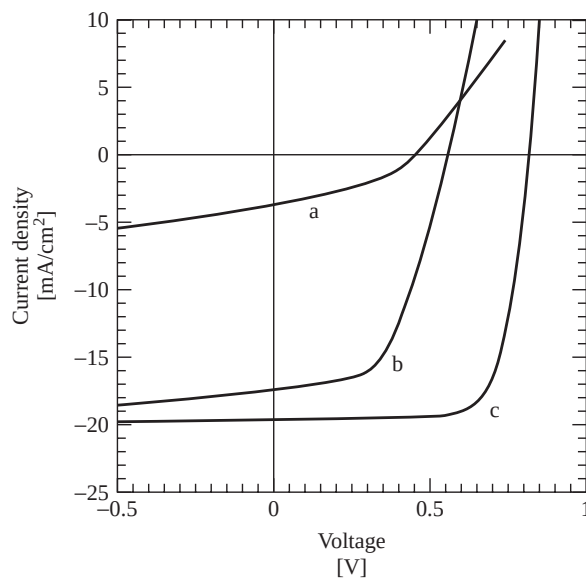
Figure 14.11 Light AM1.5 J-V curves of PVD devices with \text{Cu}_2\text{Te}/\text{C} contacts and different post-deposition processing: (a) no heat treatment; (b) treatment at 550^\circ\text{C} for 5 min in air; (c) treatment in \text{CdCl}_2 vapor at 420^\circ\text{C} for 20 min in air [105]
