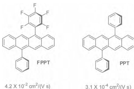
Scheme 2. Chemical structures of FPPT and PPT and corresponding hole mobilities.
