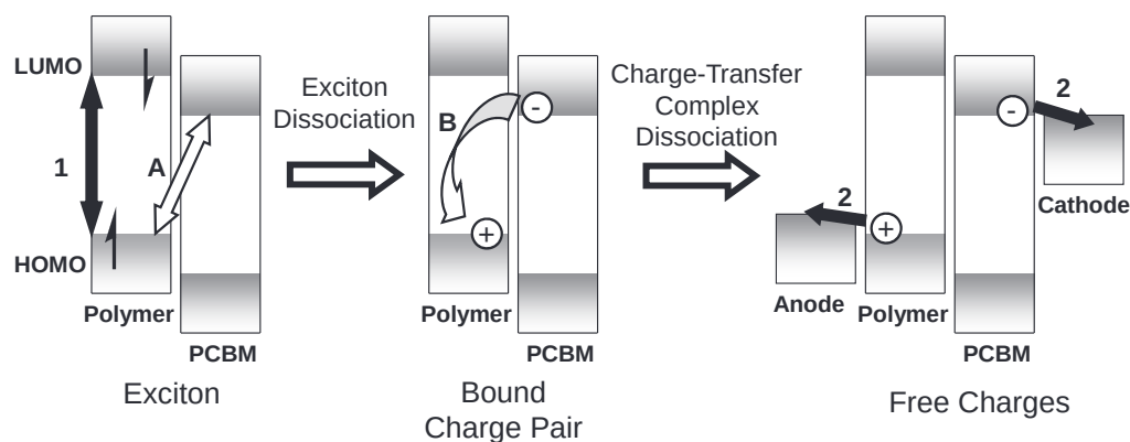
■ Figure 2. The process of exciton dissociation to charge separation. Parameters that affect the open circuit voltage ( V_{oc} ) are shown with white arrows and letters, parameters that affect the short circuit current ( I_{sc} ) are shown with black arrows and numbers.
