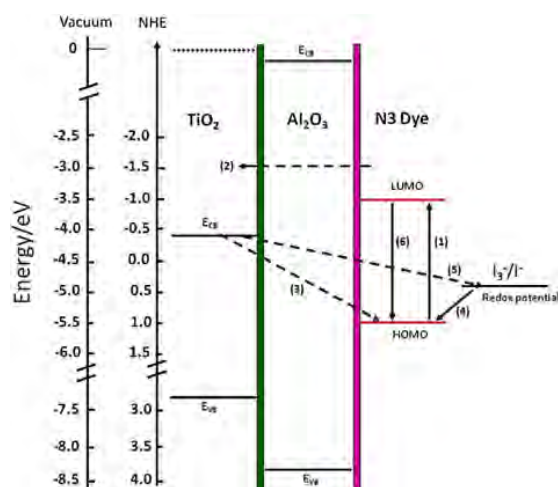
Fig. 7. Schematic diagram of band structure including interfacial charge-transfer processes occurring at \text{TiO}_2 /dye/electrolyte interface in DSSCs. Reprinted with permission from S.-W. Rhee et al. [27]. Copyright 2010, Elsevier.
