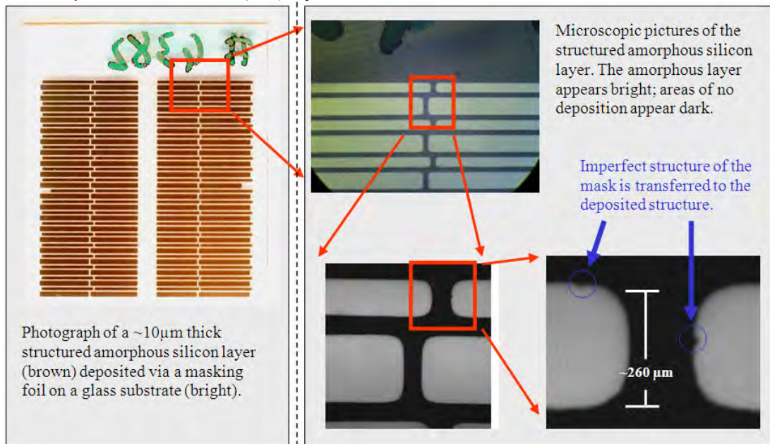
Figure 2: Structured a -Si:H layer deposited through a flexible mask according to the novel method.
