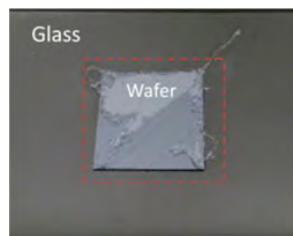
Fig. 5. Silicone degradation after dip in HF: HNO 3 mixture. The red dotted line indicates approximately the perimeter of the silicone area before dip.
