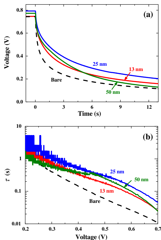
Fig. 2. (a) Experimental decay results of V_{oc} for the bare and compact-layer coated DSSCs. (b) Electron lifetimes as a function of voltage. Reprinted with permission from B. Park et al. [41]. Copyright 2012, Elsevier.
