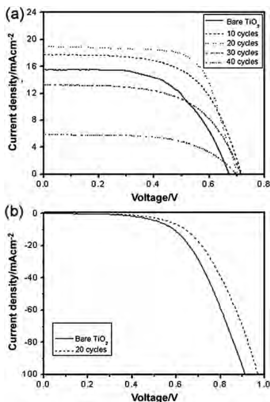
Fig. 10. (a) J - V characteristics of solar cell with bare and alumina-coated \text{TiO}_2 samples measured under one sun illumination. (b) J - V curves of bare \text{TiO}_2 and 20 cycles alumina-coated sample measured in dark. Reprinted with permission from S.-W. Rhee et al. [27]. Copyright 2010, Elsevier.
