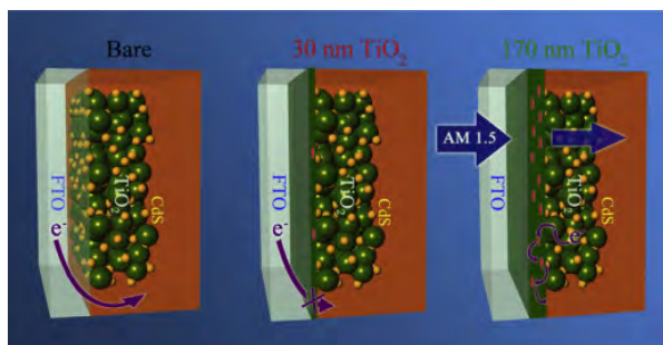
Fig. 4. Schematic figures of the \text{TiO}_2 blocking-layer effects on the performance of CdS-sensitized solar cells. Reprinted with permission from B. Park et al. [53]. Copyright 2011, Elsevier.
