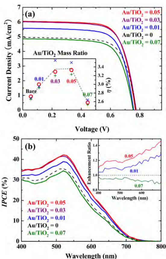
Fig. 19. (a) J–V characteristics of DSSCs at various Au/TiO 2 mass ratios. The inset shows the power-conversion efficiency of DSSCs with respect to the Au/TiO 2 mass ratio. (b) Incident photon-to-current conversion efficiency spectra of DSSCs at various Au/TiO 2 mass ratios. The IPCE enhancement ratios are also shown compared with the bare DSSC (Au/TiO 2 = 0) in the inset. Reprinted with permission from B. Park et al. [111]. Copyright 2011, American Institute of Physics.
