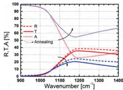
Fig. 4. Infrared carrier reflectance, transmittance, and absorbance of the sample cSi(n)/aSi(i/p + )/ITO (80 nm) before and after annealing at 200 °C for 1 h.
