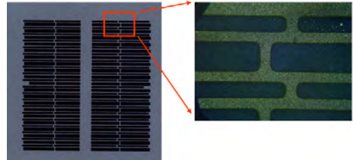
Figure 4: Photograph (left) and microscopic picture (right) of a \sim 80\text{nm} thick structured indium tin oxide (ITO) layer (dark/blue) deposited via a masking foil on a silicon wafer (grey).
