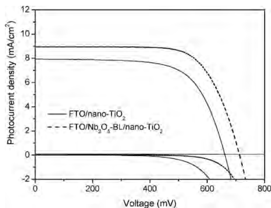
Fig. 6. J – V curves of cells employing Z-907 sensitized \text{FTO}/\text{TiO}_2 (solid line) and \text{FTO}/\text{Nb}_2\text{O}_5\text{-BL}/\text{nano-TiO}_2 (dashed line) under AM 1.5 illumination. Reprinted with permission from S. Yanagida et al. [48]. Copyright 2007, Royal Society of Chemistry.
