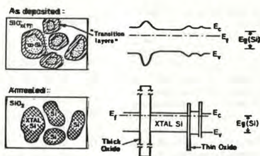
Fig. 3: (A) postulated structure of as-deposited SIPOS (B) and after annealing; the "oxide-like" regions become more \text{SiO}_2 -like, accompanied by crystallization of the silicon crystallites.
