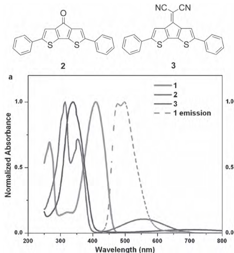
Figure 7. Molecules 2 and 3 have electrochemical band gaps of 2.1 and 1.7 eV, respectively, yet the absorption coefficients below 3.0 eV (413 nm) for these compounds are exceptionally poor. Adapted with permission. [62] Copyright 2011, American Chemical Society.
