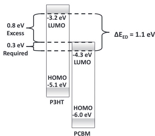
Figure 4. One of the key limitations of the P3HT:PCBM system is the 1.1 eV LUMO P3HT - LUMO PCBM gap ( \Delta E_{ED} ) where only 0.3 eV is required.
