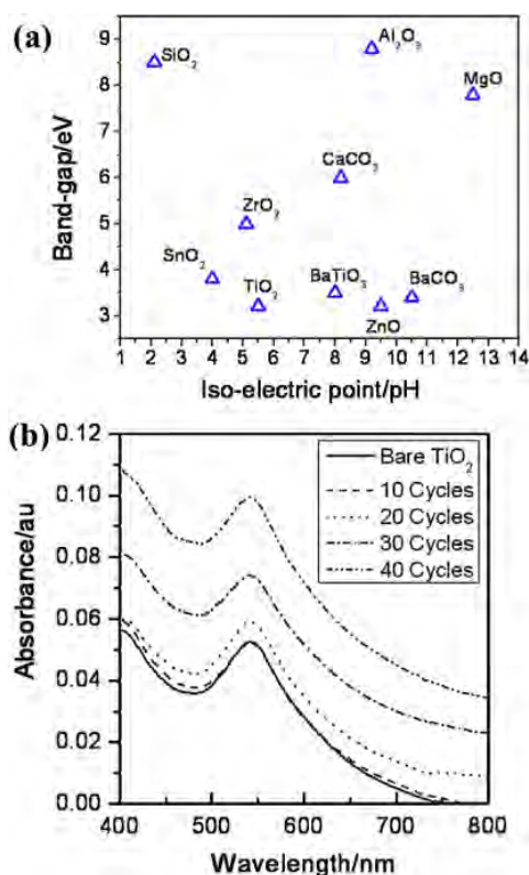
Fig. 8. (a) Graphical representation of isoelectric point and bandgap of various oxide materials. (b) Absorbance spectra of dye desorbed from bare and alumina-coated \text{TiO}_2 samples using 0.1 M NaOH. Alumina was deposited by ALD process with deposition cycles between 10 and 40. Reprinted with permission from S.-W. Rhee et al. [27]. Copyright 2010, Elsevier.
