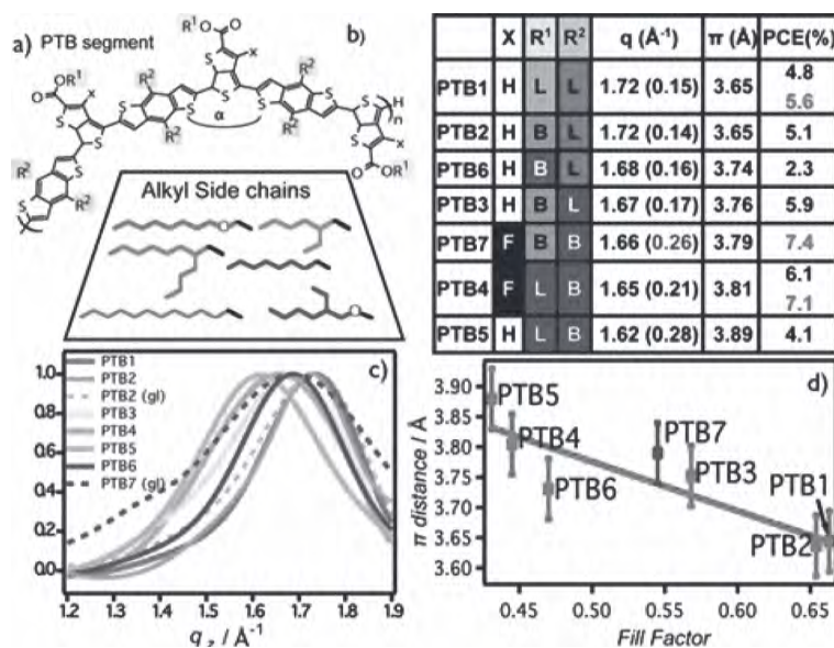
Figure 11. Photovoltaic properties and XRD values of PTB polymers. Reproduced with permission. [74]
