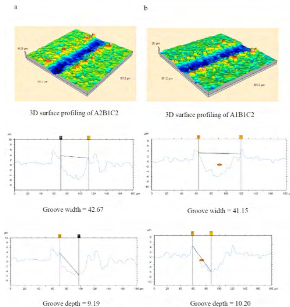
Fig. 3 Comparisons of the measured surface profiling. (a) Experiment 4 for order 1: A2B1C2; (b) confirmation experiment for optimal combination: A1B1C2.
