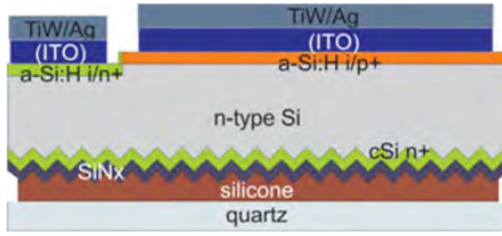
Fig. 1. Scheme of the devices obtained with the designed flow. The ITO layer is only present in the HJ ITO split, and the cell dimension is 2.5 \times 2.5 \text{ cm}^2 .
