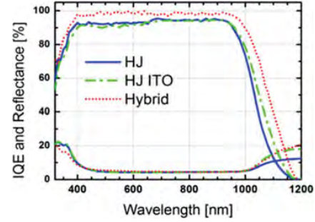
Fig. 2. Reflectance and IQE of the best cells of each split. For comparison, the IQE and reflectance of the Hybrid cells are also reported [19].
