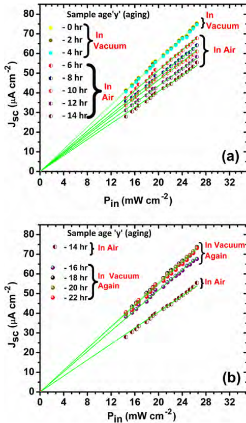
Fig. 1. J_{sc}-P_{in} characteristics of S-1 at 300 K for illumination with laser radiation of 789 nm wavelength from p^+ side for (a) initial 4 h aging under vacuum and next 10 h aging under air ambient; (b) after 14 h aging under air ambient and for next 8 h aging under vacuum again.
