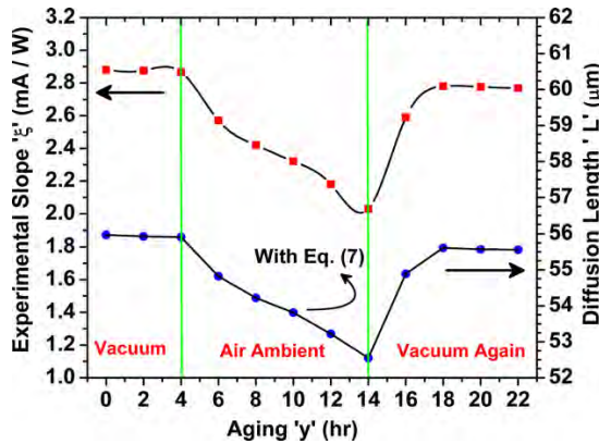
Fig. 2. Variations in the slope \xi of J_{sc} – P_m curve and in the diffusion length L as determined using Eq. (7) with the aging of specimen S-1 in vacuum–air–vacuum.
