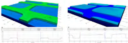
Figure 4: Topographies of the structured deposited a-Si:H layers shown in figure 1 (right) and etched a-Si:H layer after plasma etching from figure 2 (left) prepared by a confocal microscope.
