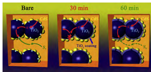
Fig. 12. Schematic figures of the \text{TiCl}_4 -treatment effects on the performance of CdS-sensitized solar cells. Reprinted with permission from B. Park et al. [32]. Copyright 2012, Elsevier.
