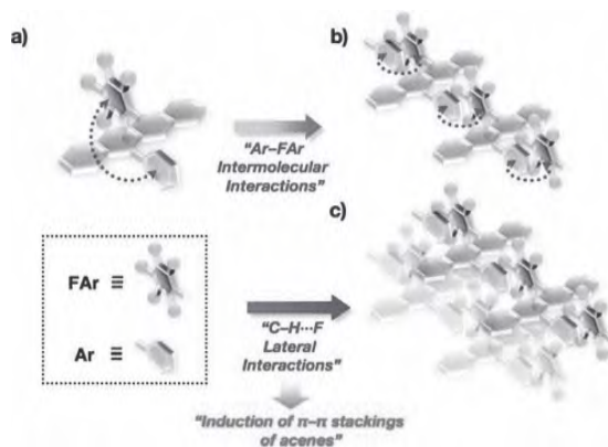
Figure 10. Molecular design and concept for the enhancement of \pi - \pi stacking between neighboring charge transporting units by the introduction of Ar and FAr substituents. Reproduced with permission. [82] Copyright 2011, American Chemical Society.
