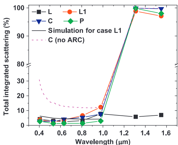
Fig. 3. Total integrated scattering as a function of wavelength at an incidence angle \theta_i of 8° for ultrafast laser textured silicon (L), ultrafast laser textured silicon that has been annealed (L1), chemically textured silicon with SiN x (C) and porous silicon surface (P).
