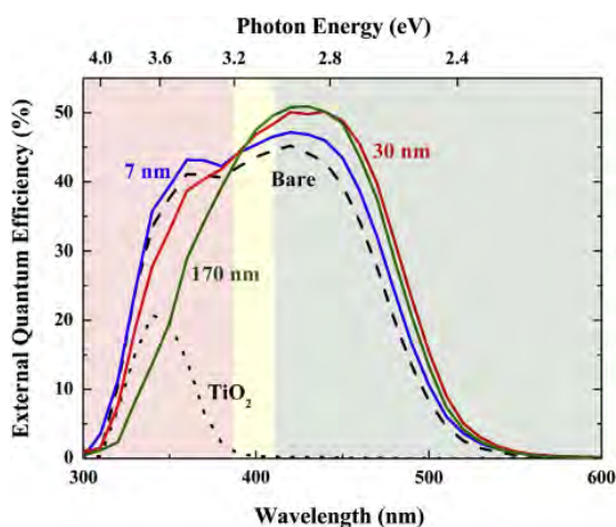
Fig. 3. Incident photon-to-current conversion efficiency (IPCE) spectra of QDSCs with various blocking-layer thicknesses. The IPCE of \text{TiO}_2 nanoparticles without CdS sensitizer is shown as a dotted line. Reprinted with permission from B. Park et al. [53]. Copyright 2011, Elsevier.
