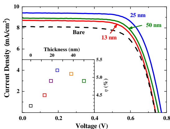
Fig. 1. Photocurrent–voltage curves of DSSCs with various \text{TiO}_2 compact-layer thicknesses. The inset shows power-conversion efficiency of DSSCs as a function of the compact-layer thickness. Reprinted with permission from B. Park et al. [41]. Copyright 2012, Elsevier.
