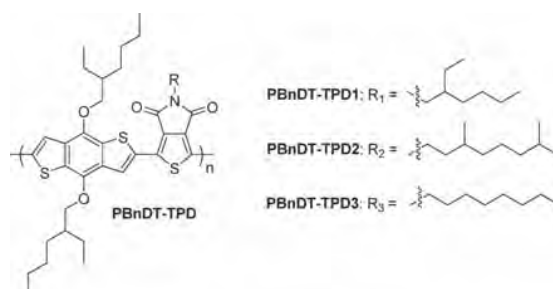
Scheme 3. Structures of PBnDT-TPD polymers.
