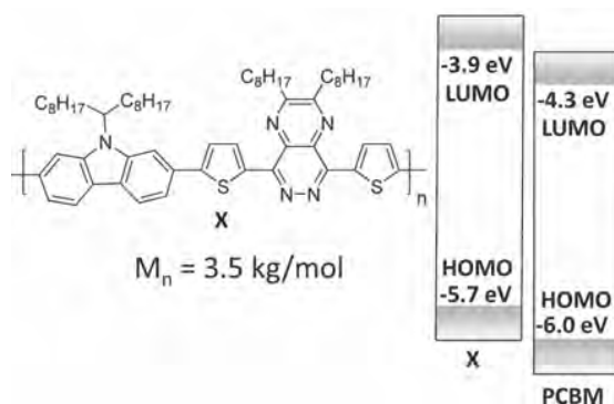
Figure 5. Pyridazine-based polymer with a near optimal LUMO.
