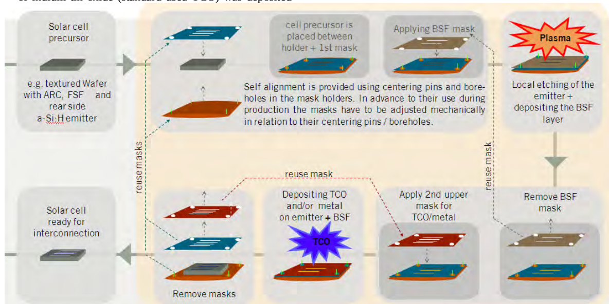
Figure 5: Example of one possible process flow using a BEHIND-like [5] procedure to prepare the structured a-Si:H layers.
