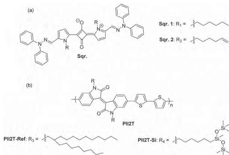
Scheme 4. Structures of (a) Sqr. and (b) PII2T derivatives.
