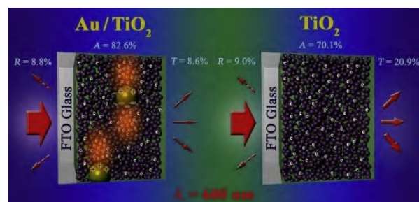
Fig. 20. Schematic figure representing the enhancement of Au/TiO 2 -DSSC. Field enhancement near the Au nanoparticles is depicted as orange-color regions. Reprinted with permission from B. Park et al. [111]. Copyright 2011, American Institute of Physics.
