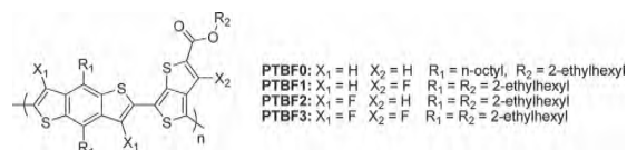
Scheme 1. Chemical structures of PTBF polymer series.
