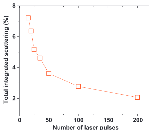
Fig. 4. Total integrated scattering as a function number of laser pulses for ultrafast laser textured silicon. Angle of incidence is 8° and wavelength of incident light is 633 nm.
