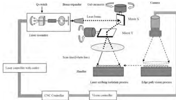
Fig. 2 Configuration of the laser scribing system for solar cell wafers.
