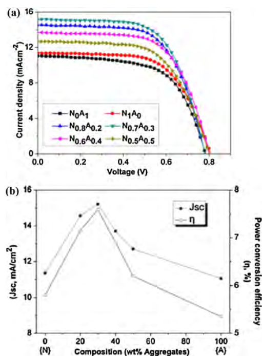
Fig. 17. (a) J–V curves of DSSCs with mixed photoelectrodes. (b) Comparison of the short-circuit current density and power-conversion efficiency as a function of TiO 2 nanoparticle (N) and aggregate (A) fraction. Reprinted with permission from G. Cao et al. [105]. Copyright 2011, Elsevier.
