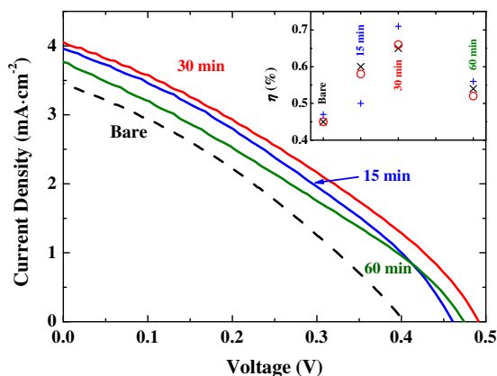
Fig. 11. Photocurrent-voltage curves of CdS quantum-dot-sensitized solar cells with various \text{TiO}_2 -coating times. The inset shows power-conversion efficiency of QDSCs as a function of the coating time. Reprinted with permission from B. Park et al. [32]. Copyright 2012, Elsevier.
