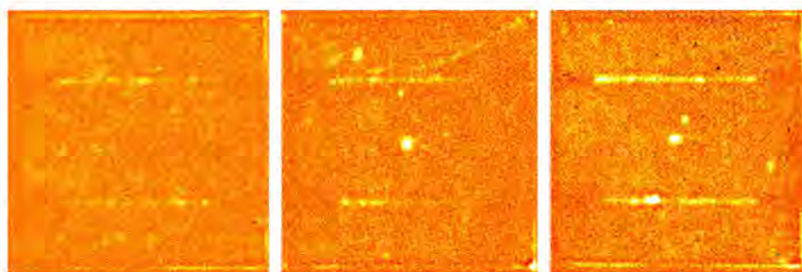
Fig. 4. Dark thermography maps at V_{\text{oc}} conditions of industrial solar cells of 156 × 156 mm 2 size. Left: reference industrial laser edge isolation, middle: edge isolation with waterjet-guided laser (variant 2, cf. Table 1), right: dry UV laser edge isolation.
