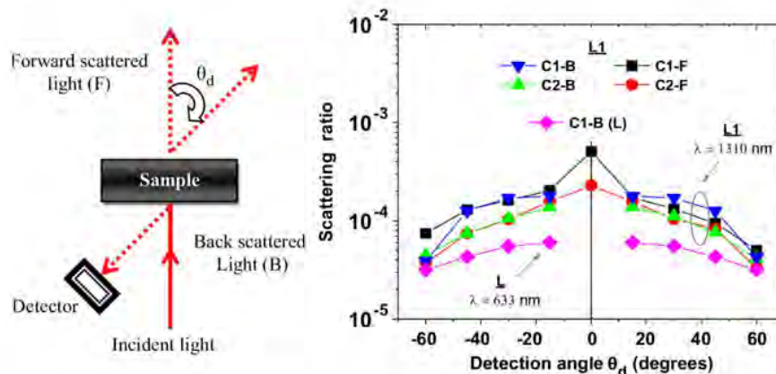
Fig. 5. (a) Experimental setup used to characterize light scattering for the ultrafast laser textured surface and (b) scattering as a function of detection angle for the ultrafast laser textured silicon (L) and annealed ultrafast laser textured silicon (L1) surfaces. L1 sample has been characterized by forward (F) as well as backward scatterings (B) at a wavelength of 1310 nm. The C1-B curve represents the backward scattering ratio and C1-F refers to forward scattering ratio for the configuration where light is normally incident on the textured surface. The C2-B curve represents the backward scattering ratio and C2-F refers to forward scattering ratio for the configuration where light is normally incident on the polished surface. The ultrafast laser textured silicon, C1-B (L), surface is only characterized for backward scattering for a wavelength of 633 nm.
