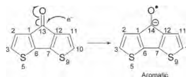
Figure 6. CPD monomer is an easily reduced, 13 electron species. Addition of 1 more electron causes the entire heterocyclic system to become aromatic because it has 14 electrons. The LUMO orbital resides almost exclusively on the carbonyl.
