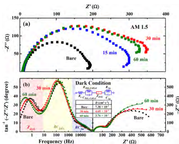
Fig. 13. (a) Electrochemical impedance spectra measured under AM 1.5 illumination, and (b) Bode and Nyquist plots measured under dark conditions with various \text{TiO}_2 -passivation conditions at V_{oc} . Reprinted with permission from B. Park et al. [32]. Copyright 2012, Elsevier.
