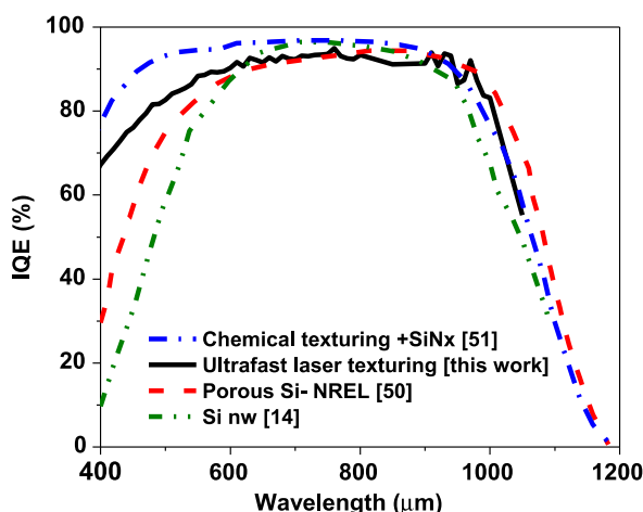
Fig. 6. Internal quantum efficiency of solar cells fabricated with different texturing schemes.
