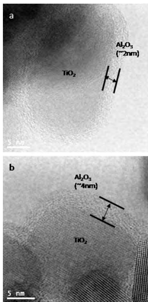
Fig. 9. High-resolution TEM images of \text{TiO}_2 porous layer covered with ALD alumina deposited with (a) 20 cycles and (b) 40 cycles. Reprinted with permission from S.-W. Rhee et al. [27]. Copyright 2010, Elsevier.
