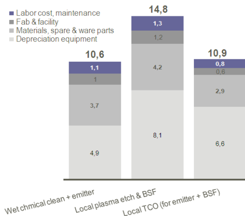
Figure 9: Cost distribution for the process flow of figure 5 excluding cost for preparing the cell precursor.
