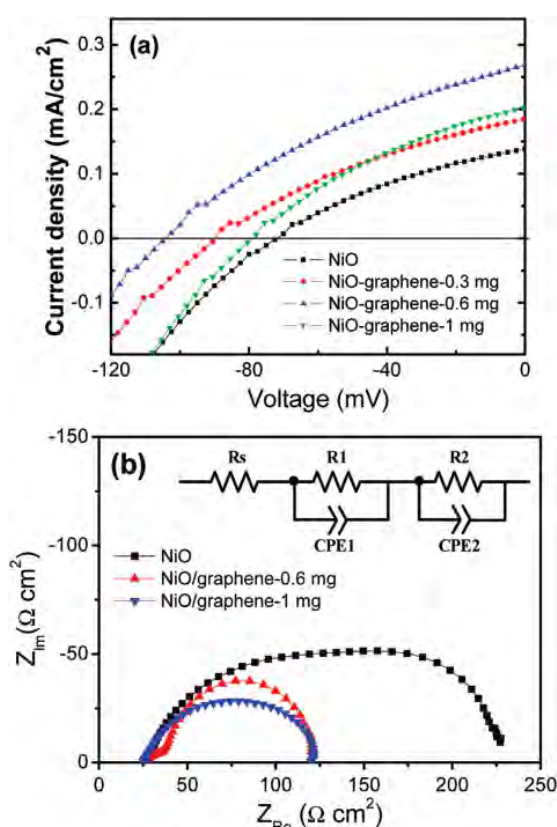
Fig. 23. (a) J - V characteristics of p -type DSSCs based on NiO and NiO/graphene composite films. (b) Nyquist plots of p -type DSSCs based on NiO and NiO/graphene composite electrodes. The inset displays the equivalent circuit of the devices. From Ref. [118].
