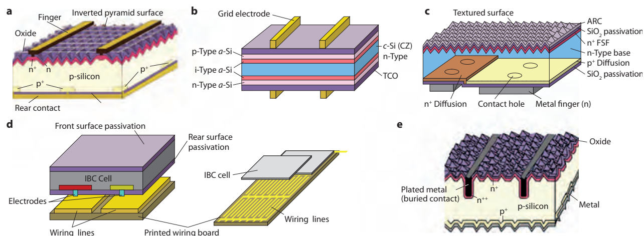
Figure 4. Schematics of various crystalline solar cell structures. (a) PERC. Adapted from Ref. 5 (© 1999 Wiley-VCH Verlag GmbH & Co. KGaA). (b) HIT. Adapted from Ref. 48 (© 2008 WIP Munich). (c) BC-BJ. Adapted from Ref. 49. (d) interdigitated back-contact (IBC) cell using surface mount technology. Adapted from Ref. 17 (© 1976 IEEE). (e) Buried-contact cell structure by BP Solar. Adapted from Ref. 40 (© 2008 IEEE). All figures reproduced with permission.
