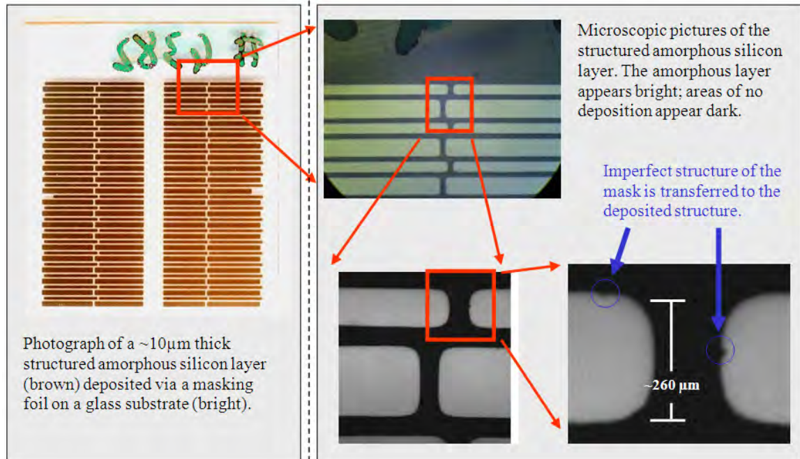
Figure 2: Structured \alpha -Si:H layer deposited through a flexible mask according to the novel method.
