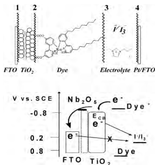
Fig. 5. Schematic views of interfaces in the DSSC device and the electron transfer of the \text{FTO}/\text{Nb}_2\text{O}_5/\text{TiO}_2 electrode. Reprinted with permission from S. Yanagida et al. [48]. Copyright 2007, Royal Society of Chemistry.
