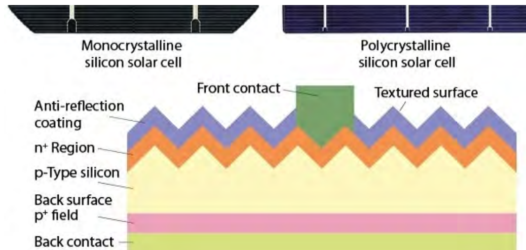
Typical mono- and polycrystalline silicon solar cells (upper), and simplified cross-section of a commercial monocrystalline silicon solar cell (lower) (© 2010 Sharp).
