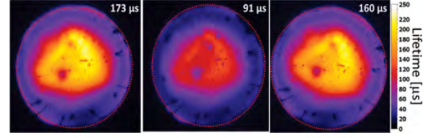
Fig. 3. PL pictures of monitor wafers for the evaluation of the a-Si:H passivation. The measurements are taken after: a-Si:H(i/p + ) passivation (left); ITO deposition and etching (middle); 1 h annealing at 200 °C (right). The lifetimes measured at an injection level of 10^{15} \text{ cm}^{-3} are indicated.
