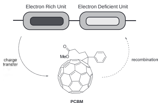
Figure 12. Possible interaction between polymer and PCBM, charge transfer, and recombination pathway are shown by arrows. Outer gray borders represent alkyl side chains. Reproduced with permission. [89] Copyright 2011 American Chemical Society.
