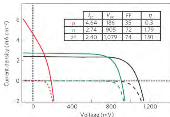
Fig. 22. J - V characteristics of a tandem solar cell (black) as well as p -type DSSCs (red) and n -type DSSCs (green) under illumination (solid lines) and in the dark (dashed lines). (For interpretation of the references to colour in this figure legend, the reader is referred to the web version of this article.) Reprinted with permission from U. Bach et al. [116]. Copyright 2010, Nature Publishing Group.
