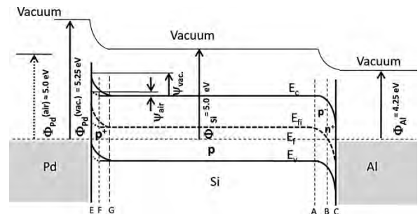
Fig. 4. A schematic energy band diagram for n + –p–p + induced structure under thermal equilibrium for specimen S-1 stored in vacuum and the air ambient. EF and FG indicate the thickness of p + accumulation layer under air and vacuum respectively, AB is p − depletion layer and BC is the n + inversion layer. \Psi_{\text{vac}} and \Psi_{\text{air}} stand for \Psi_{\text{p-p}^+} for storage of S-1 in vacuum and air respectively.
