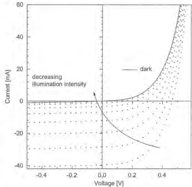
Fig. 2. Illumination-level-dependent current–voltage characteristics for the analyzed solar cell performed at room temperature.
