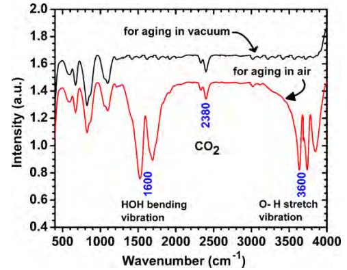
Fig. 3. FTIR spectra of Pd covered silicon wafer after taking it out from vacuum and after 10 h aging in air ambient.
