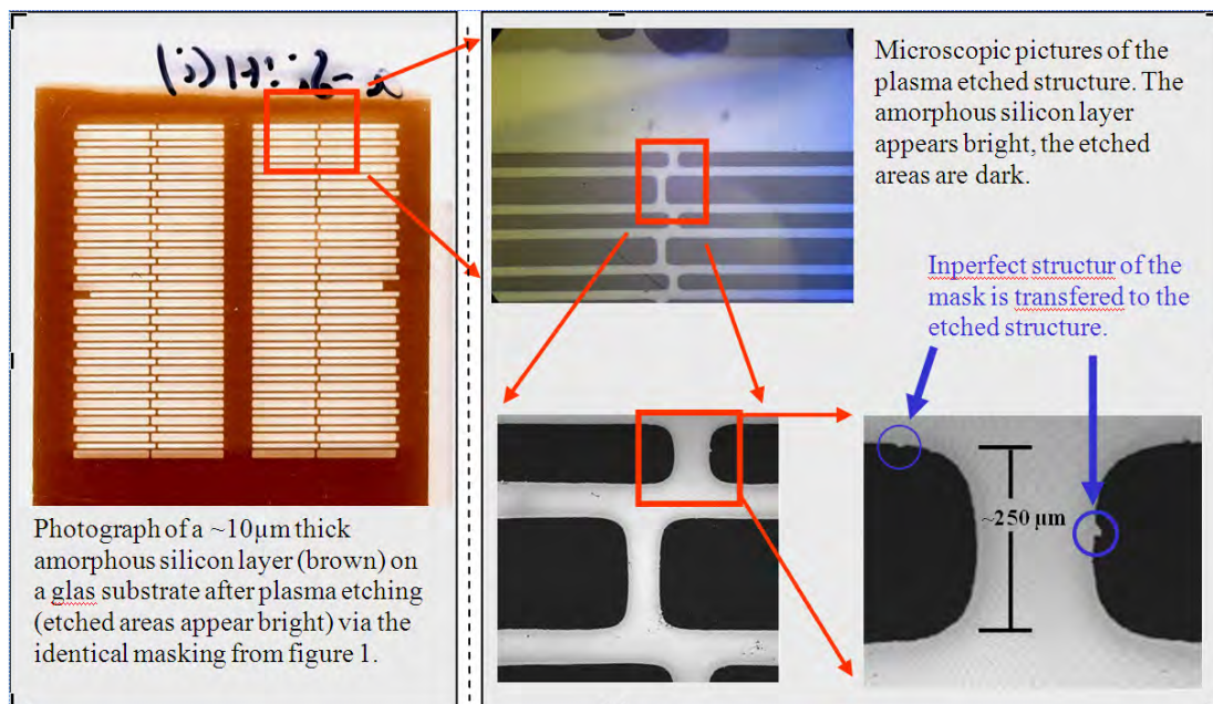
Figure 3: Structured a -Si:H layer after plasma etching through a flexible mask according to the novel method.
