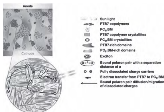
Figure 8. Diagrammatic hypothesis of the hierarchical nanomorphologies in the PTB7/PCBM active layer. Reproduced with permission. [75] Copyright 2011, American Chemical Society.
