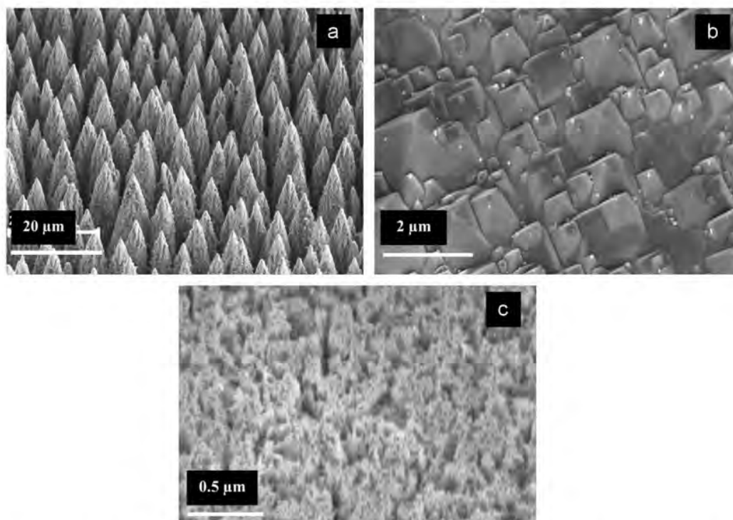
Fig. 1. SEM images of (a) ultrafast laser textured silicon surface in \text{SF}_6 gas ambient, (b) chemically textured silicon surface and (c) porous silicon surface.
