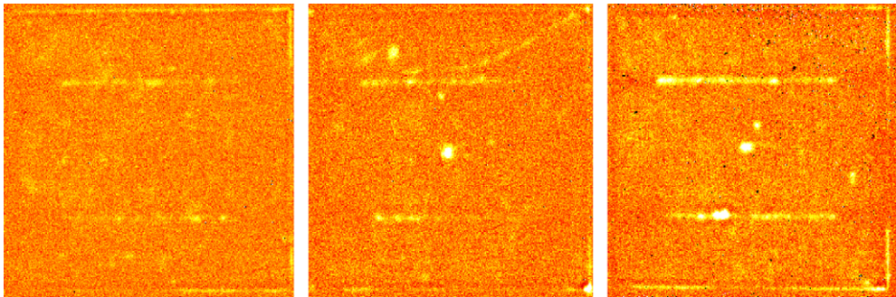
Fig. 4. Dark thermography maps at V_{oc} conditions of industrial solar cells of 156 × 156 mm 2 size. Left: reference industrial laser edge isolation, middle: edge isolation with waterjet-guided laser (variant 2, cf. Table 1), right: dry UV laser edge isolation.
