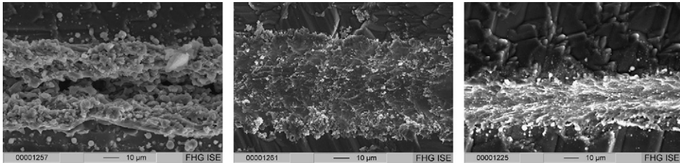
Fig. 5. SEM pictures of laser grooves from different laser processes. Left: reference industrial laser process, middle: waterjet-guided laser (variant 6, cf. Table 1), right: dry UV laser.
