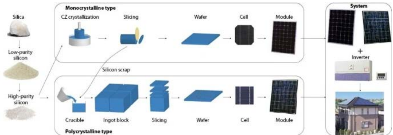
Production process for typical commercial crystalline silicon solar cells (© 2010 Sharp)
