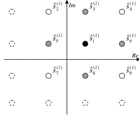
Fig. 6. Example of the simplified BQM for 16QAM.
