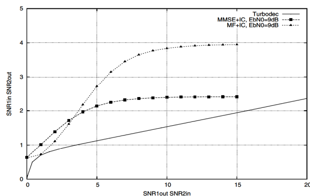
Fig. 5. Performance Comparison between MMSE+PIC and MF+PIC in a 32-user system with E_b/N_0 = 9dB
