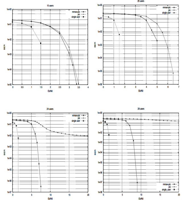
Fig. 3. Ber Performance
