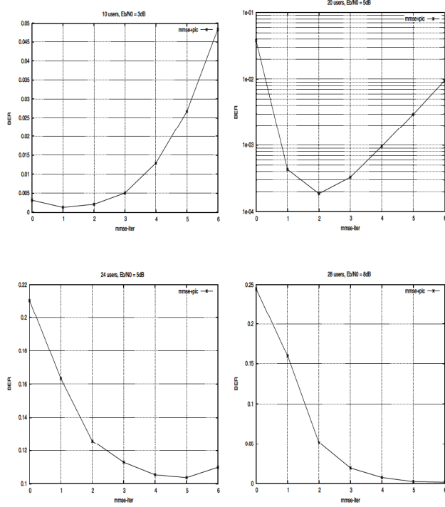
Fig. 2. Ber Performance
