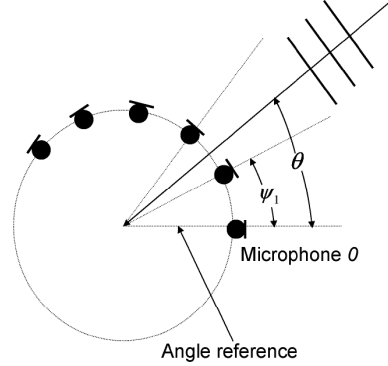
Fig. 1. Circular array geometry.
