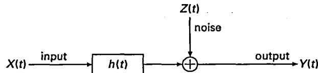
Figure 1.5. Linear Gaussian channel model.
