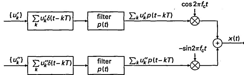
Figure 6.7. DSB-QC modulation.
