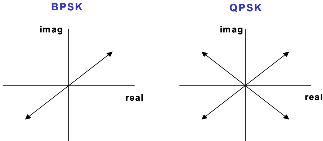
Figure 153T—BPSK and QPSK signaling with the I/Q channels maximally energized
