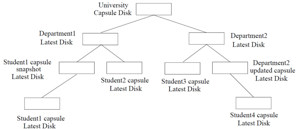
Figure 1: An example capsule hierarchy.
