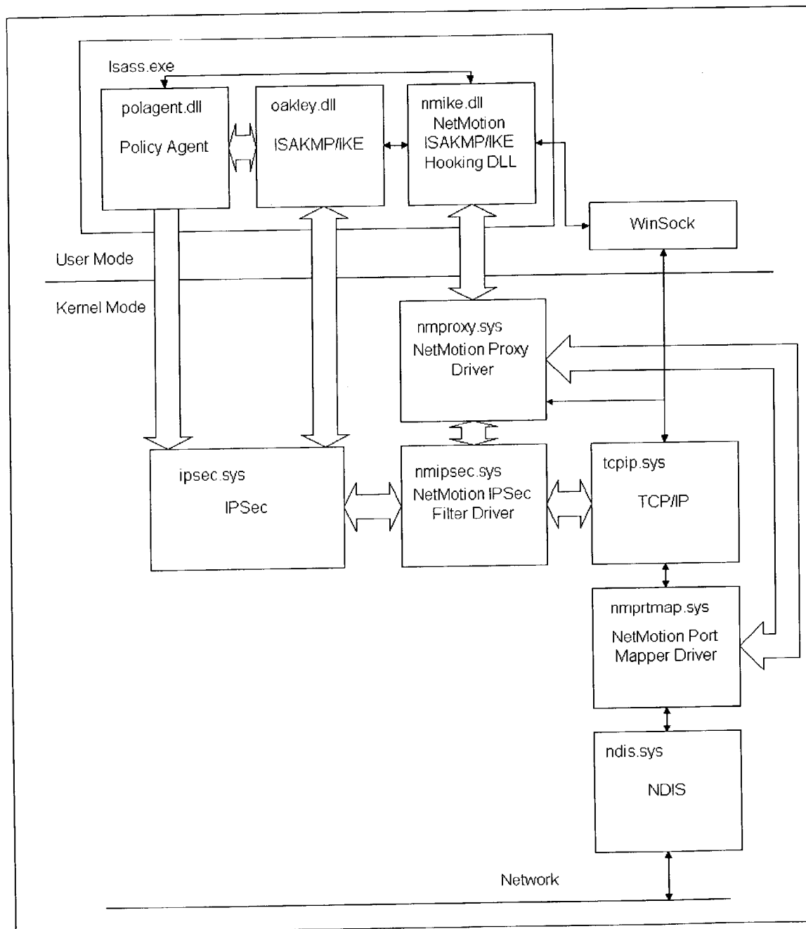
Figure 10 – Example Server Architecture
