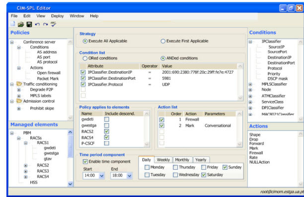
Figure 3 - Graphical editor view
