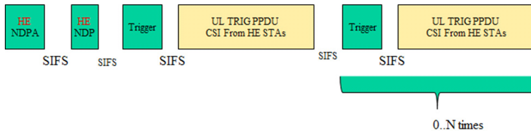
Figure 25-5—An example of the sounding protocol with a single HE beamformee
