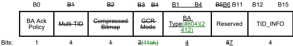
Figure 9-33—BA Control field
