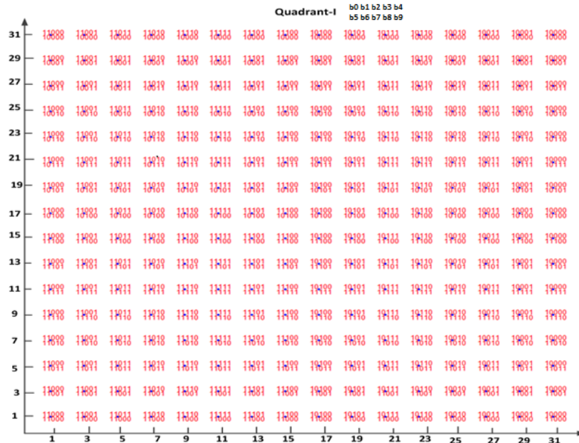
Figure 26-31—Constellation bit encoding for 1024-QAM (1st quadrant)
