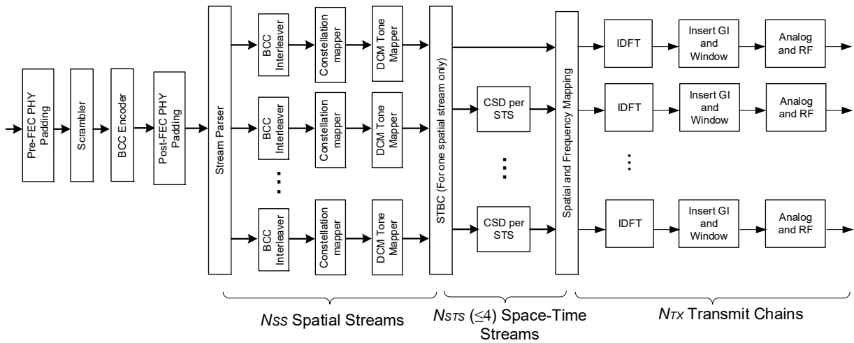
Figure 26-9—Transmitter block diagram for the Data field of an HE SU transmission in a 26-, 52-, 106- or 242-tone RU (#838) with BCC encoding
