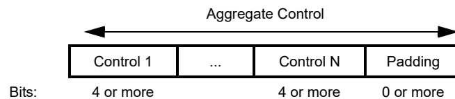
Figure 9-15a—Aggregated Control subfield of the HE variant HT Control field( #360 )( #792 )( #1711 )( #2204 )
