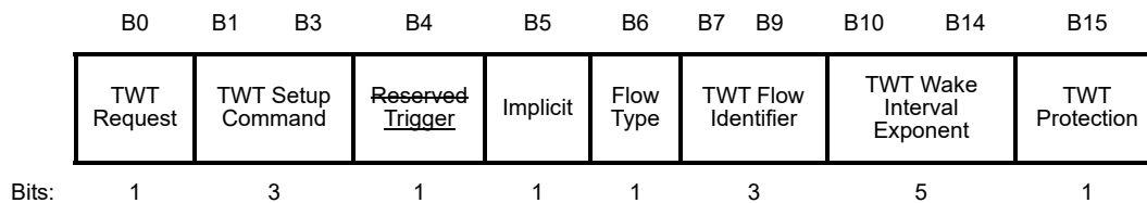
Figure 9-586ay—Request Type field format
