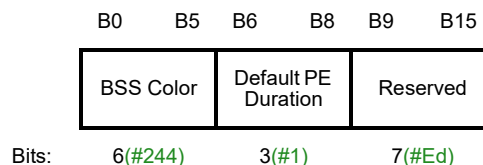
Figure 9-ax6—HE Operation Parameters(#1350) field format
