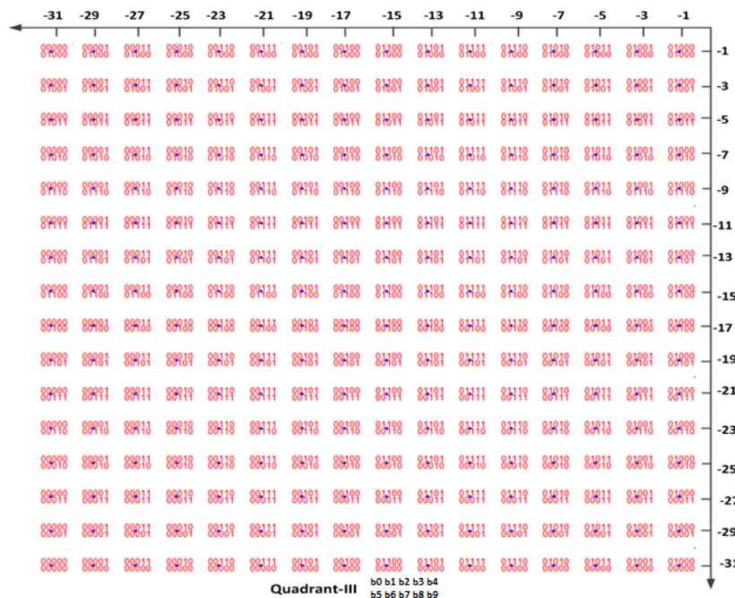
Figure 26-33—Constellation bit encoding for 1024-QAM (3rd quadrant)
