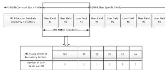
Figure 26-25—Illustration for the mapping of the 8-bit RU allocation subfield and the position of the user-field to the STA's assignment
