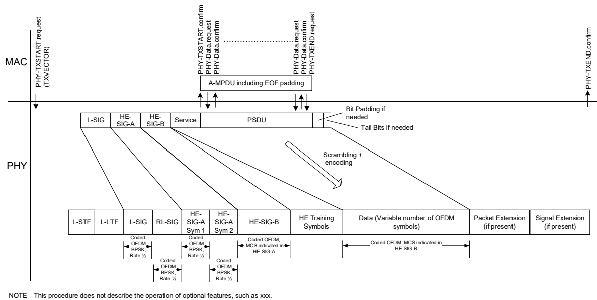
Figure 26-39—PHY transmit procedure for an HE MU PPDU
