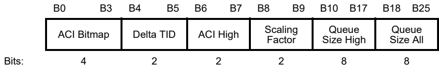
28 29 30 31 Figure 9-15f—Control Information subfield format when Control ID subfield is 3
