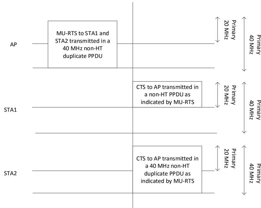
Figure 10-ax3—An example of an MU-RTS frame soliciting CTS frame(#Ed)(#1396) responses on the primary 40 MHz channel(#2224)
