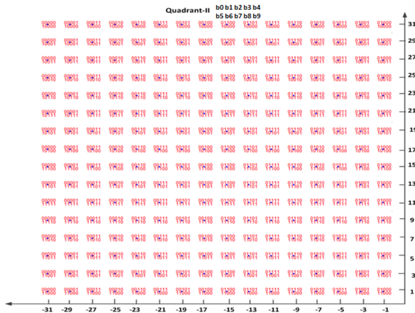
Figure 26-32—Constellation bit encoding for 1024-QAM (2nd quadrant)
