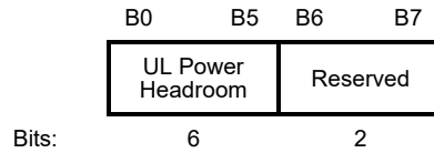
Figure 9-15g—Control Information subfield format when the Control ID subfield is 4
