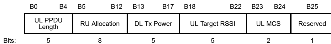
Figure 9-15c—Control Information subfield format when Control ID subfield is 0
