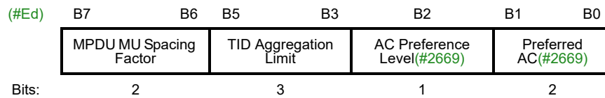
Figure 9-52e—Trigger Dependent User Info field for the Basic Trigger variant
