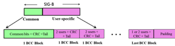
Figure 26-20—HE-SIG-B field encoding structure in each 20 MHz
