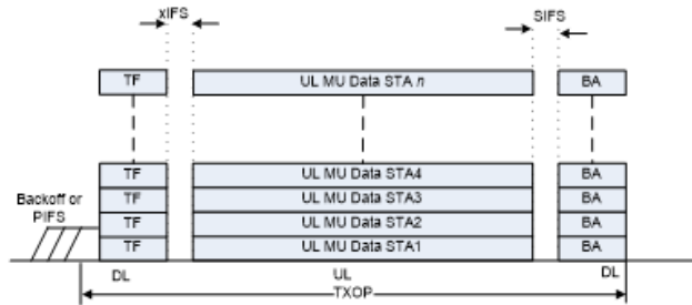
Figure 10-ax5—An example of a TXOP containing an UL MU transmission with an immediate DL MU transmission containing individually addressed (#1512) BlockAck frames acknowledging the frames received from the respective STAs
