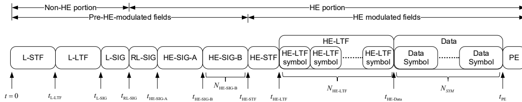
Figure 26-18—Timing boundaries for HE PPDU fields(#899)
