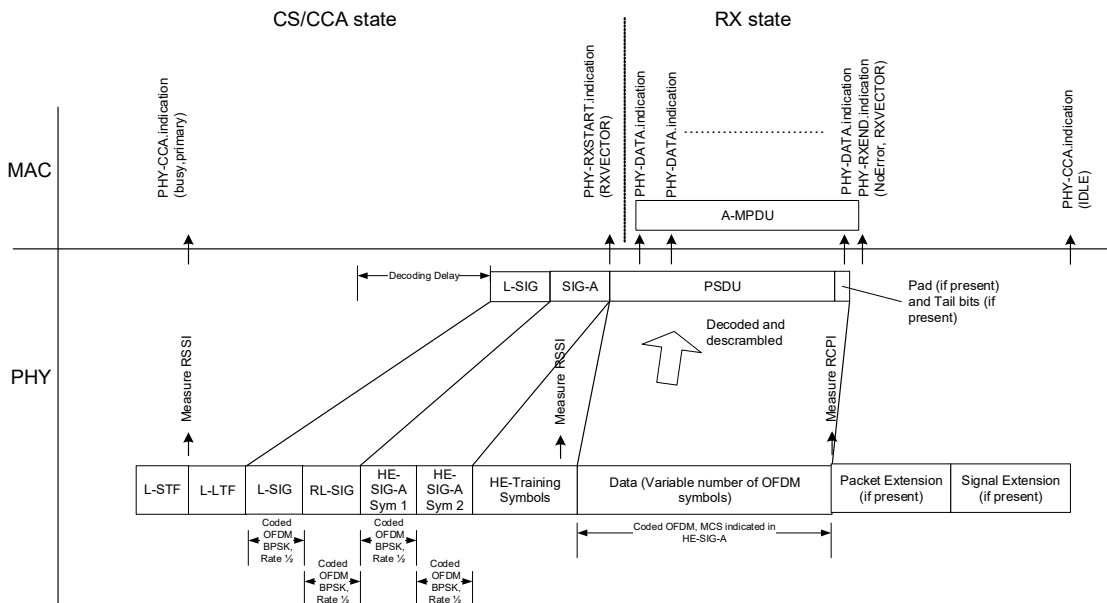
Figure 26-42—PHY receive procedure for an HE SU PPDU
