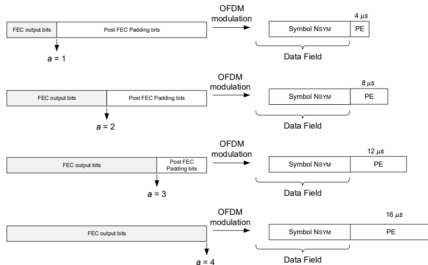
Figure 26-36—PE field when maximum PE duration is 16 \mu s (non STBC)
