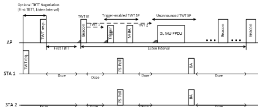
Figure 10-ax2—Example of broadcast TWT operation
