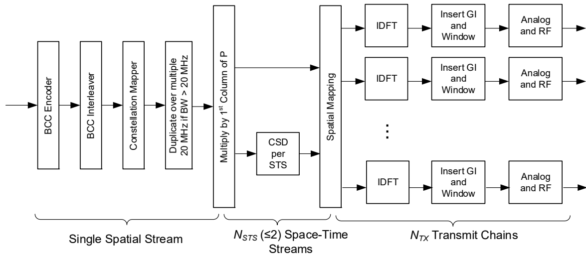
Figure 26-6—Transmitter block diagram for the L-SIG, RL-SIG and HE-SIG-A fields for an HE SU PPDU and HE extended range SU PPDU when the Beam Change field is 0(#2360)(#1659)
