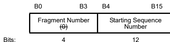
Figure 9-28—Block Ack Starting Sequence Control subfield(#515)
