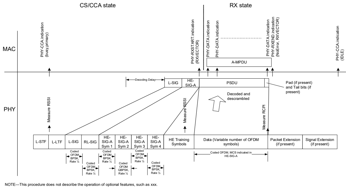
Figure 26-43—PHY receive procedure for an HE extended range SU PPDU
