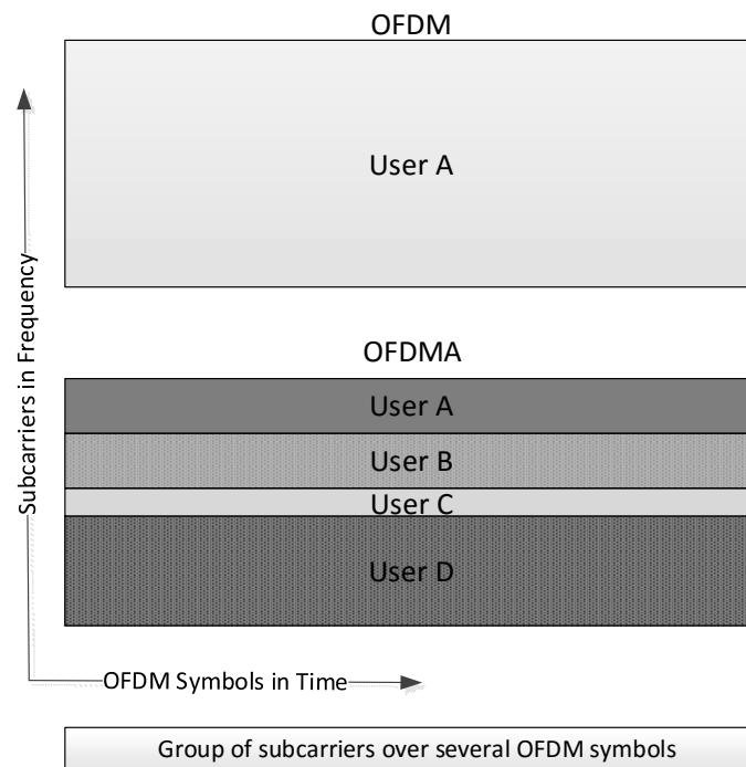
Figure 26-14—Illustration of OFDM and OFDMA concepts
