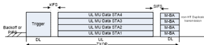
Figure 10-ax7—An example of a TXOP containing UL MU transmissions with an immediate DL non-HT duplicate PPDU containing the Multi-STA BlockAck frame. The UL MU transmissions may be OFDMA or MU-MIMO
