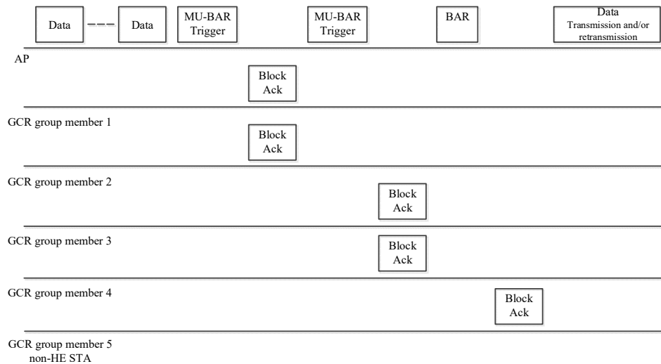
Figure 10-36a—Example of a frame exchange with GCR block ack retransmission policy (#22)(#415)(#1442)
