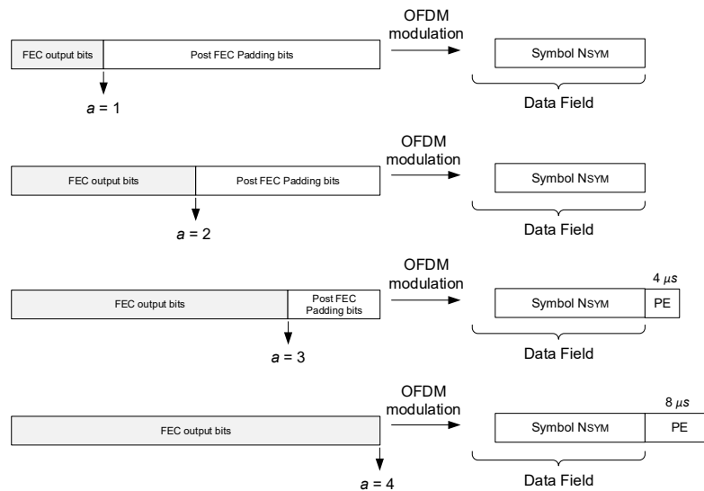
Figure 26-35—PE field when maximum PE duration is 8 \mu s (non STBC)
