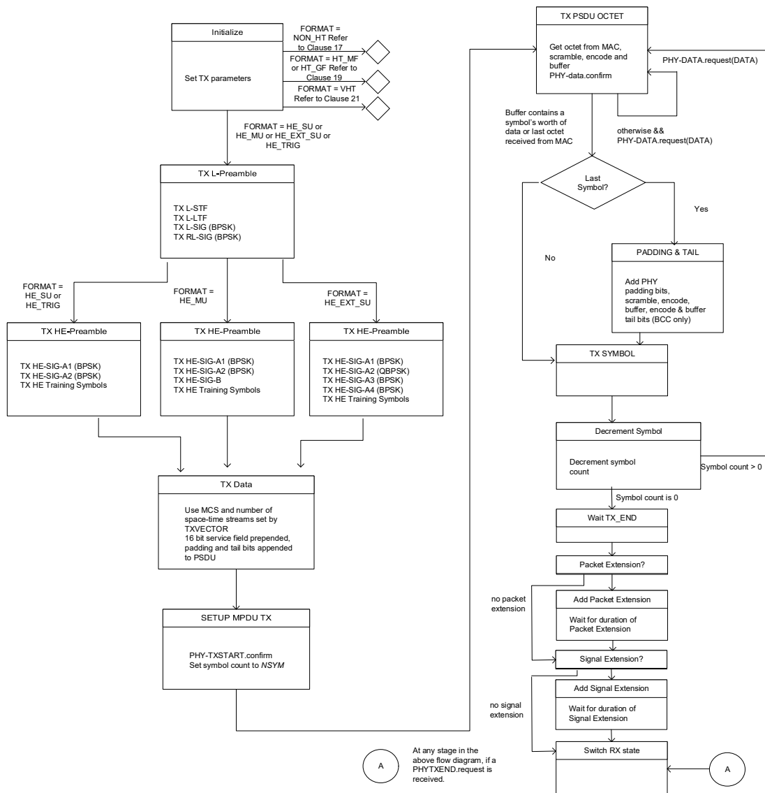
Figure 26-41—PHY transmit state machine for an HE PPDU
