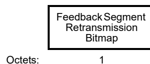
Figure 9-52f—Trigger Dependent User Info field for the Beamforming Report Poll variant
