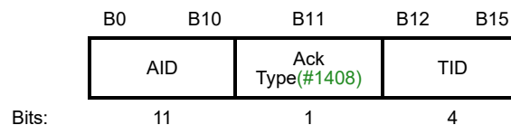
Figure 9-38b—Per AID TID Info subfield format
