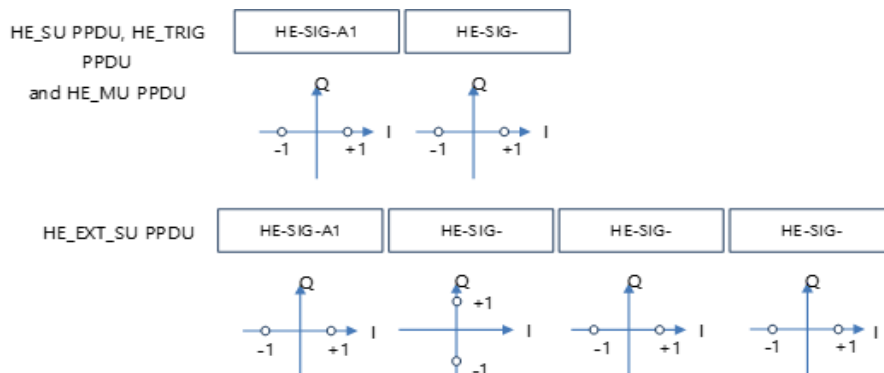
Figure 26-19—Data tone constellation of HE-SIG-A symbols
