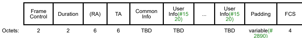
Figure 9-52a—Trigger frame
