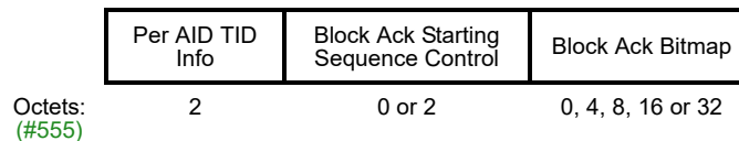
Figure 9-38a—Per STA Info subfield format
