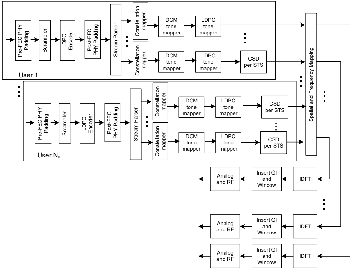
Figure 26-11—Transmitter block diagram for the Data field of an HE downlink MU-MIMO transmission in 106-, 242-, 484- or 996-tone(#838) RU with LDPC encoding(#277)
