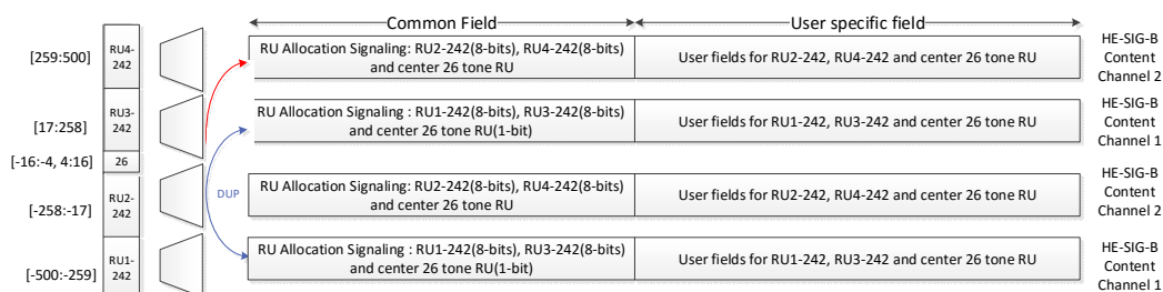
Figure 26-23—Default mapping of the two HE-SIG-B channels and their duplication in an 80 MHz PPDU
