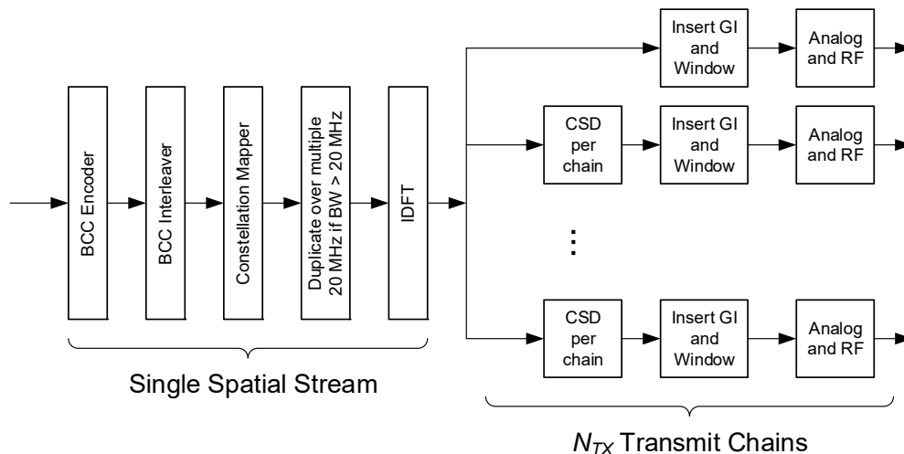
Figure 26-5—Transmitter block diagram for the L-SIG, RL-SIG and HE-SIG-A fields for an HE SU PPDU and HE extended range SU PPDU when the Beam Change field is 1 and the HE MU PPDU(#1659)
