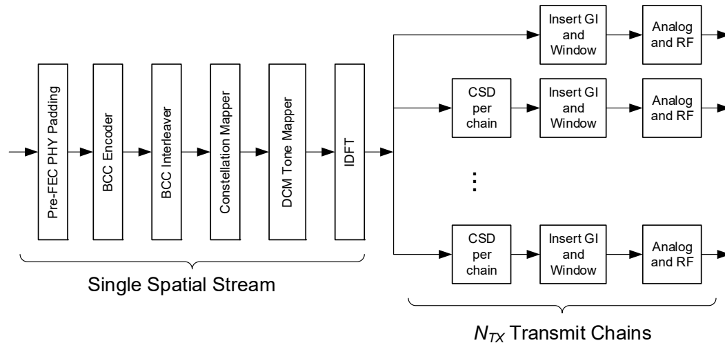
Figure 26-8—Transmitter block diagram for the HE-SIG-B field
