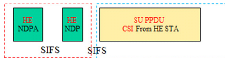
Figure 25-4—An example of the sounding protocol with a single HE beamformee
