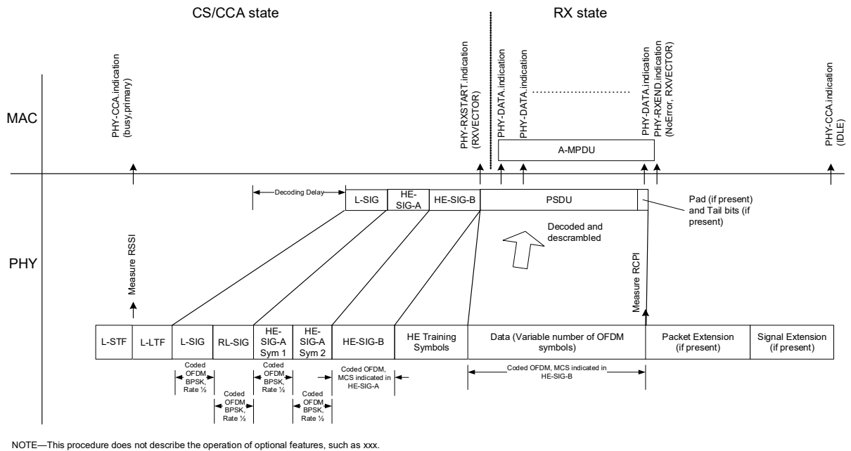
Figure 26-44—PHY receive procedure for an HE MU PPDU
