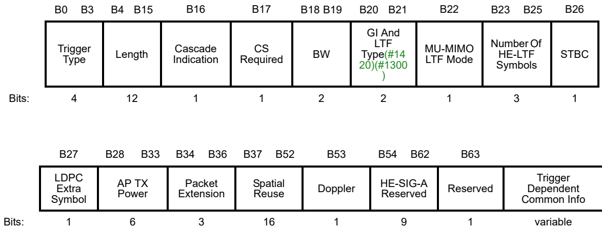
Figure 9-52b—Common Info field(#2134)(#101)
