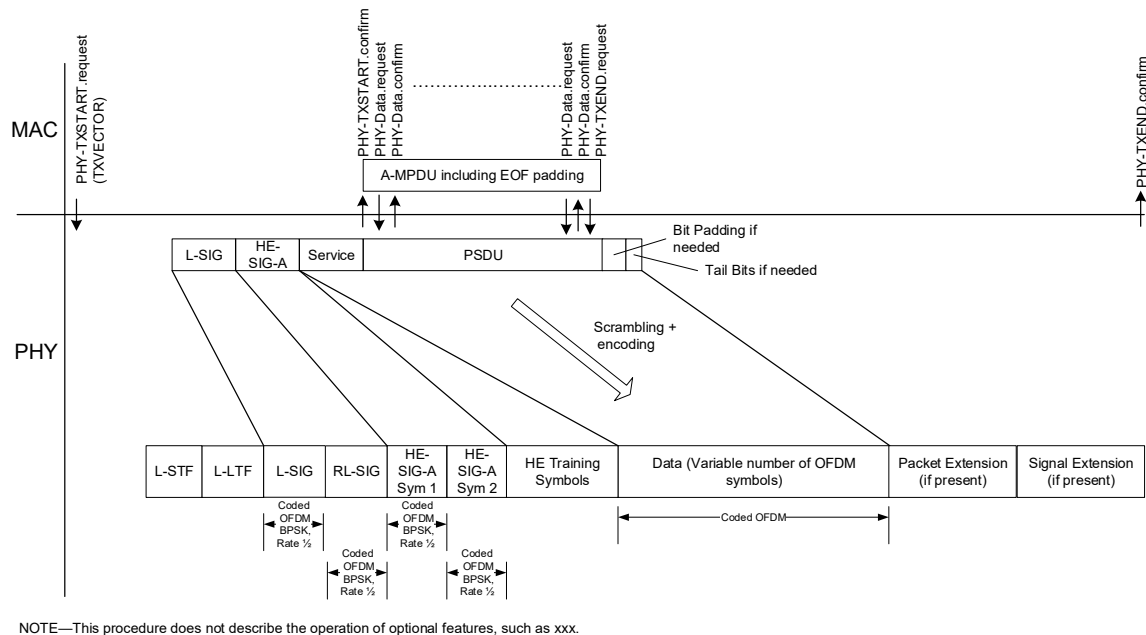
Figure 26-40—PHY transmit procedure for an HE trigger-based PPDU
