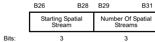
Figure 9-52d—SS Allocation subfield format
