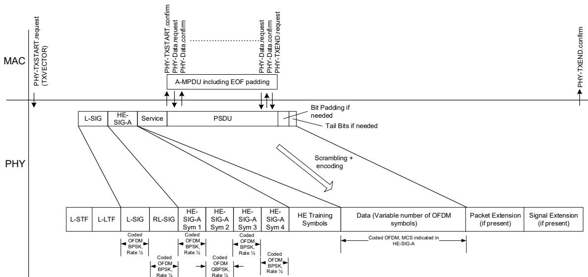
Figure 26-38—PHY transmit procedure for an HE extended range SU PPDU
