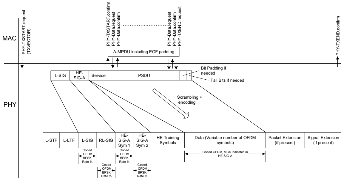
Figure 26-37—PHY transmit procedure for an HE SU PPDU
