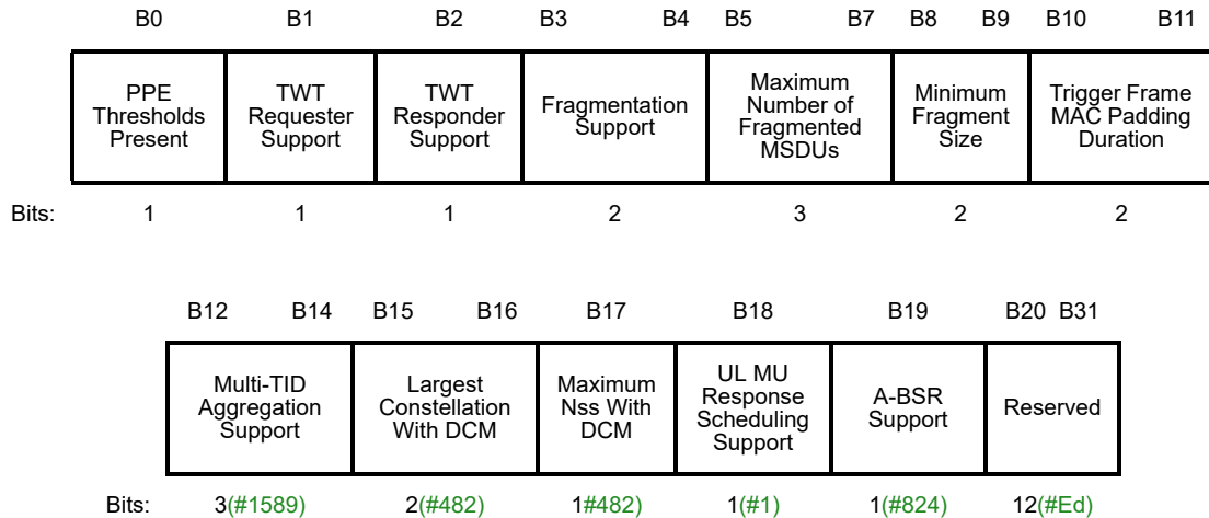
Figure 9-ax2—HE Capabilities Information field format
