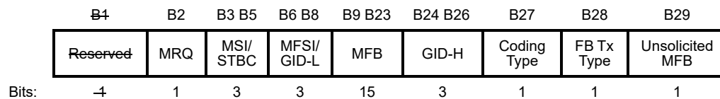
Figure 9-13— V H T Control Middle subfield of the VHT variant HT Control field
