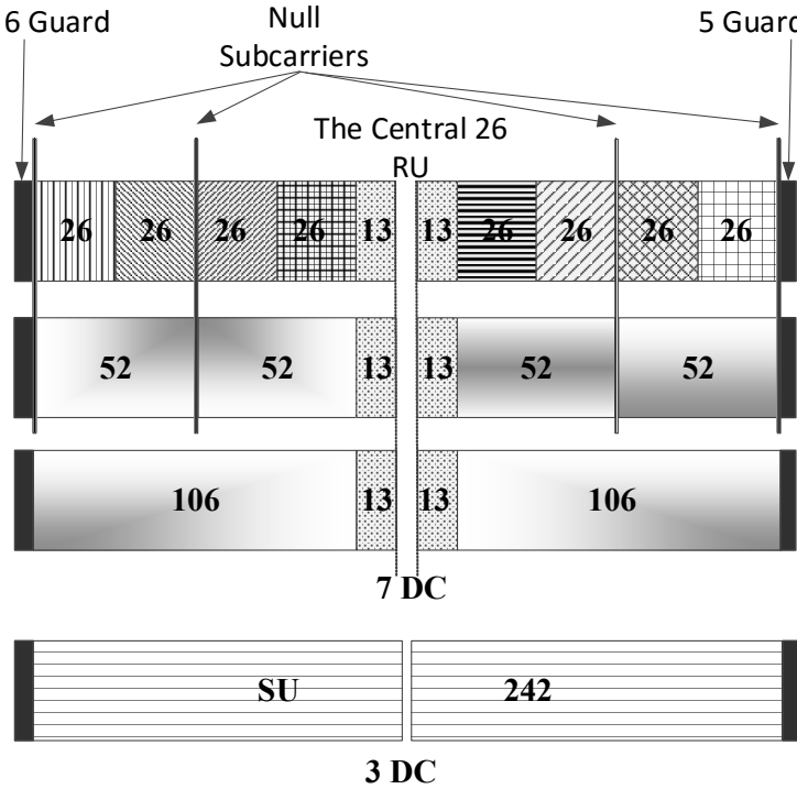
Figure 26-15—RU locations in a 20 MHz HE PPDU
