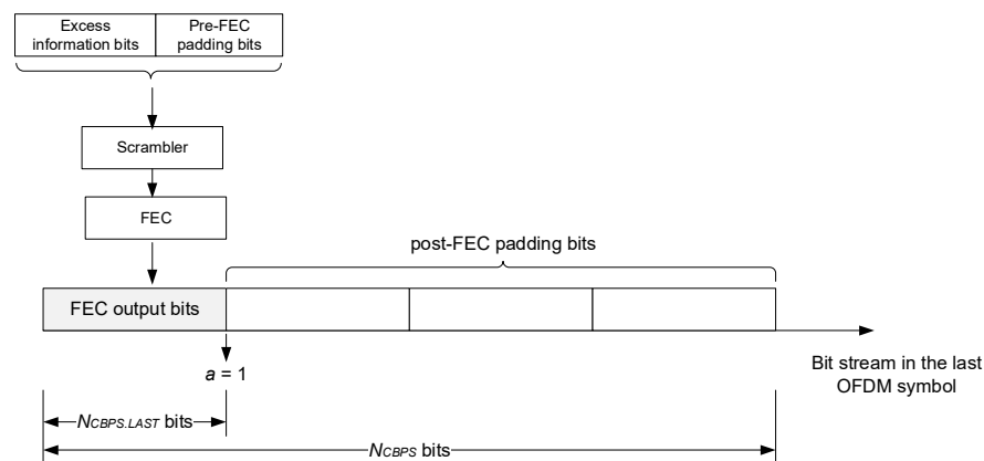
Figure 26-29—HE PPDU padding process in the last OFDM symbol (non STBC) when a = 1
