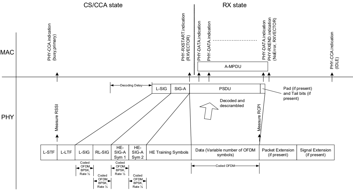
Figure 26-45—PHY receive procedure for an HE trigger-based PPDU
