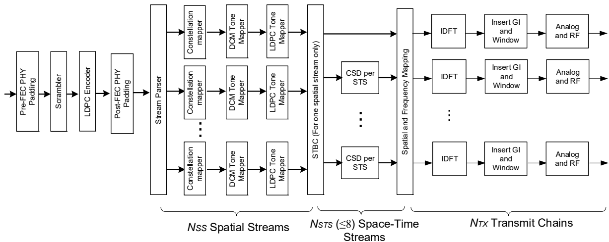
Figure 26-10—Transmitter block diagram for the Data field of an HE SU transmission in 26-, 52-, 106-, 242-, 484- or 996-tone (#838) RU with LDPC encoding
