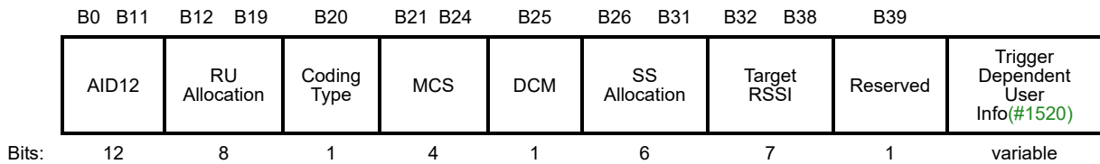
Figure 9-52c—User Info(#1520) field(#262)(#663)
