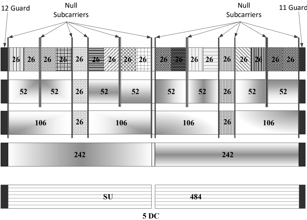
Figure 26-16—RU locations in a 40 MHz HE PPDU
