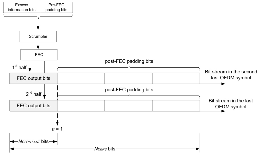
Figure 26-30—HE PPDU padding process in the last OFDM symbol (STBC) when a = 1
