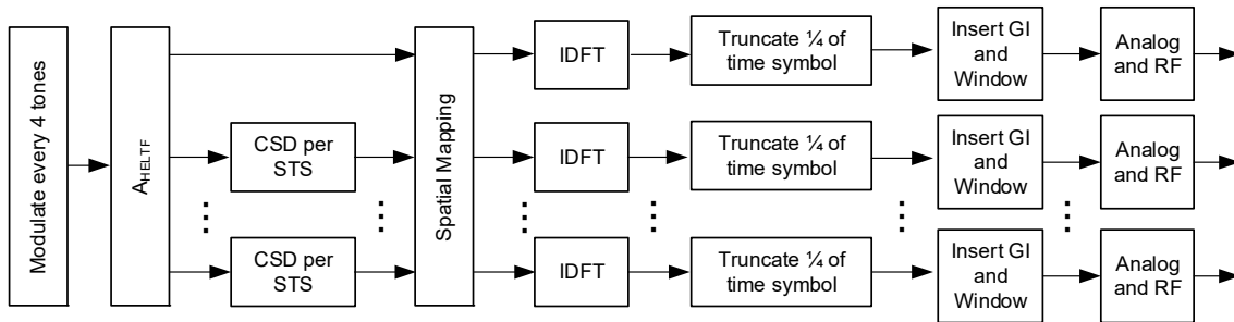
Figure 26-27—Generation of 1x HE-LTF symbols per frequency segment
