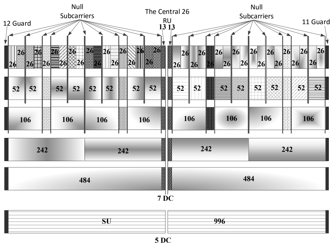
Figure 26-17—RU locations in an 80 MHz HE PPDU
