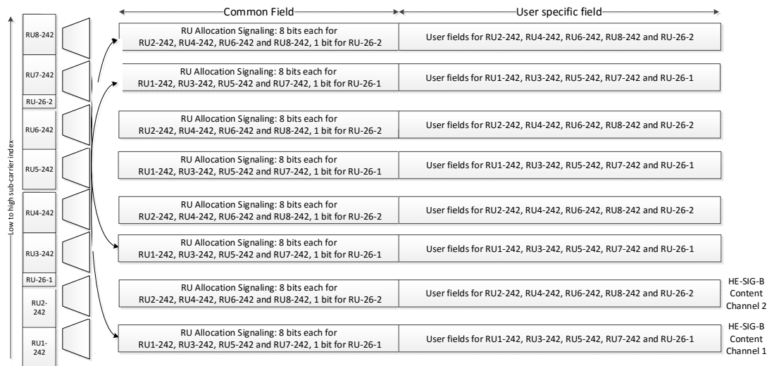
Figure 26-24—Default mapping of the two HE-SIG-B channels and their duplication in a 160 MHz PPDU
