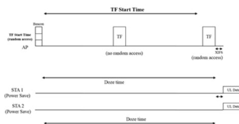
Figure 25-6—Trigger frame (TF) start time in the Beacon frame for power save operation with random access operation(#2852)
