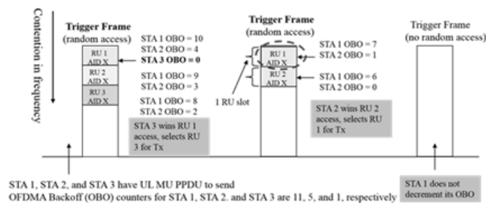
Figure 25-1—Illustration of the UL OFDMA-based random access procedure
