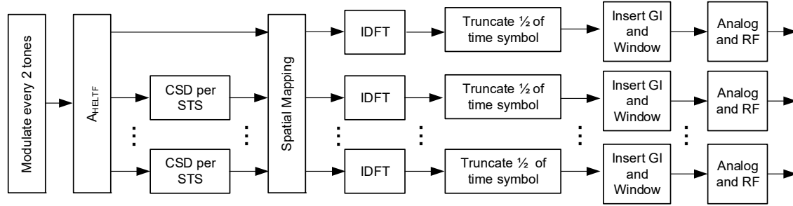
Figure 26-28—Generation of 2x HE-LTF symbols per frequency segment
