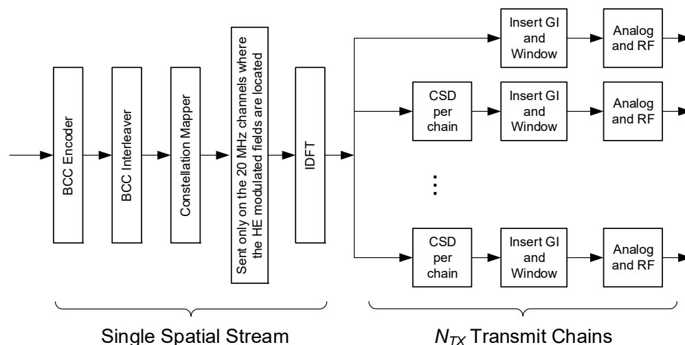
Figure 26-7—Transmitter block diagram for the L-SIG, RL-SIG and HE-SIG-A fields of an HE trigger-based PPDU(#1659)
