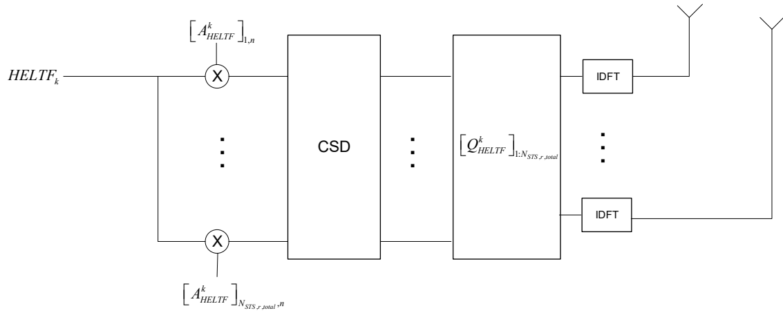
Figure 26-26—Generation of HE-LTF symbols per frequency segment in an HE SU PPDU, HE MU PPDU, HE extended range SU PPDU, and HE trigger-based PPDU using single stream pilots
