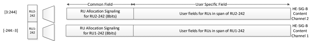
Figure 26-22—HE-SIG-B content channel for a 40 MHz PPDU
