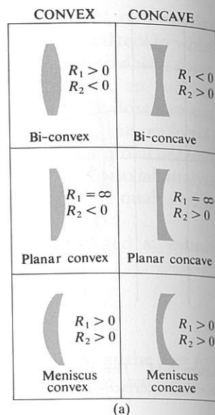
Figure 5.15 Cross sections of various centered spherical simple lenses. The surface on the left is #1 since it is encountered first. Its radius is R_1 . (Photo courtesy of Melles Griot.)
