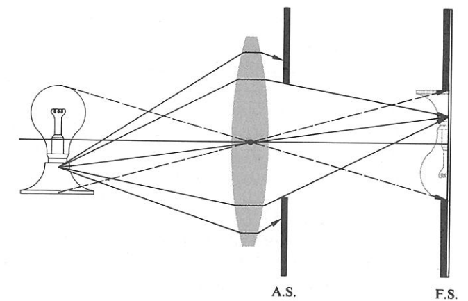
Figure 5.32 Aperture stop and field stop.
