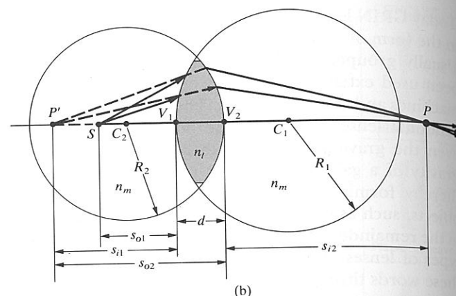
C_2 is normal to the second surface; and as the ray emerges, since n_l > n_a , the ray bends down away from that normal. (b) The geometry.
