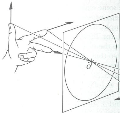
Figure 5.28 Image orientation for a thin lens.
