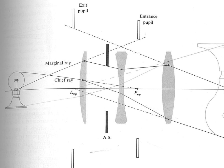
Figure 5.35 Pupils and stops for a three-lens system.
