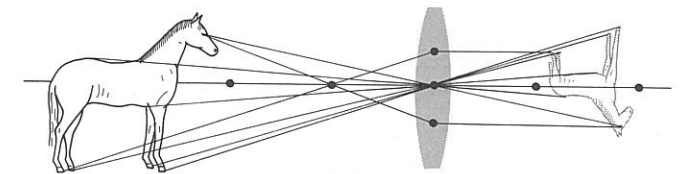
Figure 5.27 The transverse magnification is different from the longitudinal magnification.
