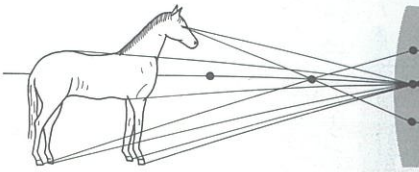
Figure 5.27 The transverse magnification longitudinal magnification.
