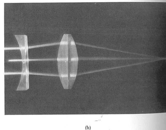
Figure 5.31 A positive and negative thin-lens combination. (Photo by E.H.)
