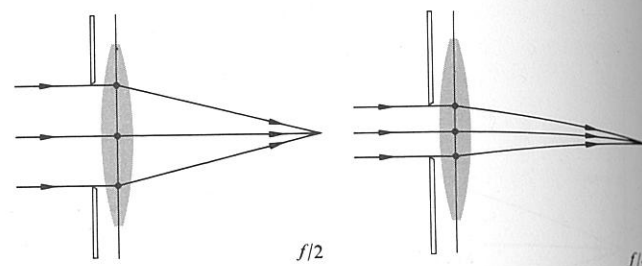
Figure 5.37 Stopping down a lens to change the f -number.
