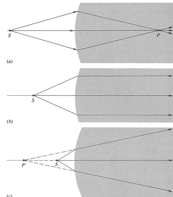
Figure 5.16 Refraction at a spherical interface.
