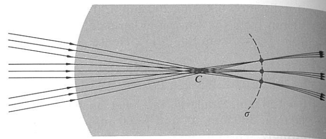
Figure 5.20 Focusing of several ray bundles.
