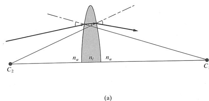
Figure 5.17 A spherical lens. (a) Refraction at the interfaces. The radius drawn from C_1 is normal to the first surface, and as the ray enters the lens it bends down toward that normal. The radius from
