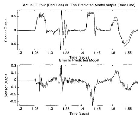
Figure 6 – Chassis Fusion Results
