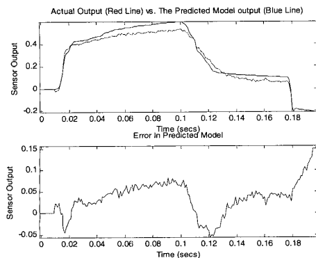
Figure 7 – Powertrain Fusion Results
