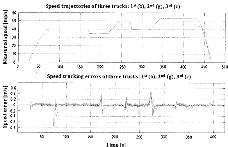
Fig. 4 Variable maximum speed platooning of three trucks. upper measured speed trajectories, and maneuver ID; Speed changes are 0 \rightarrow 40 \rightarrow 35 \rightarrow 50 \rightarrow 40 \rightarrow 53 mph; lower speed tracking errors of three trucks
