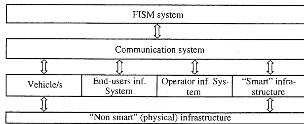
Fig. 5 CityMobil2 ARTS subsystem architecture
