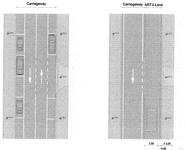
Fig. 4 Integration example of an ARTS dedicated lane in a collector street
