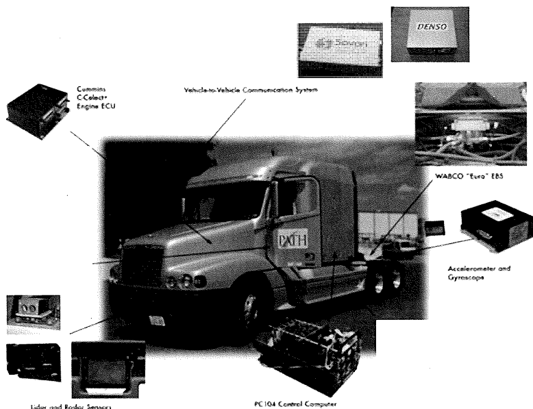
Fig. 2 Sensors and actuators installed on three trucks
