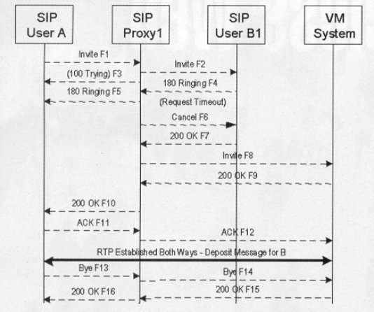
FIGURE C FORWARDED ON NO ANSWER
