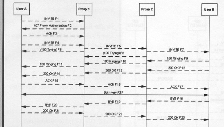
FIGURE A BASIC CALL FLOW
