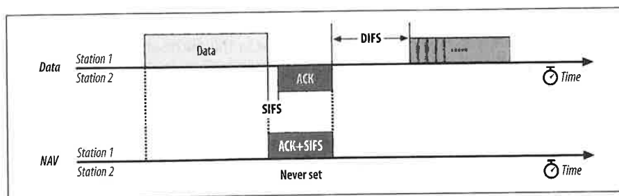
Figure 3-15. Basic positive acknowledgment of data
