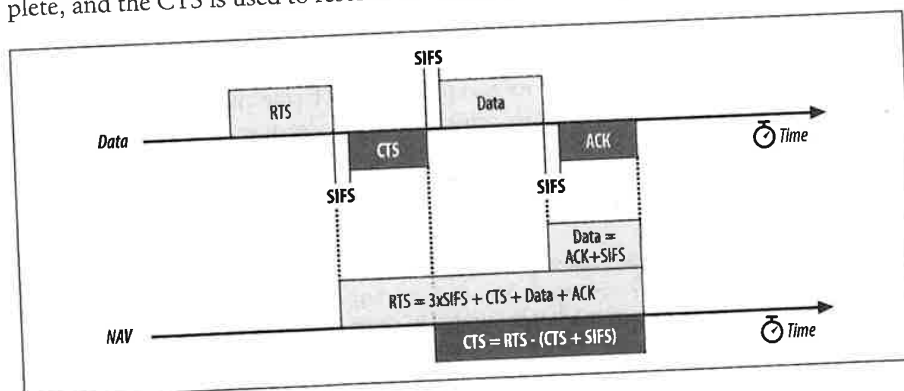
Figure 3-17. RTS/CTS lockdown
