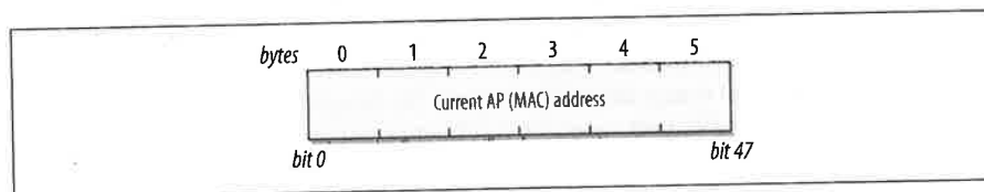
Figure 4-25. Current AP Address field
