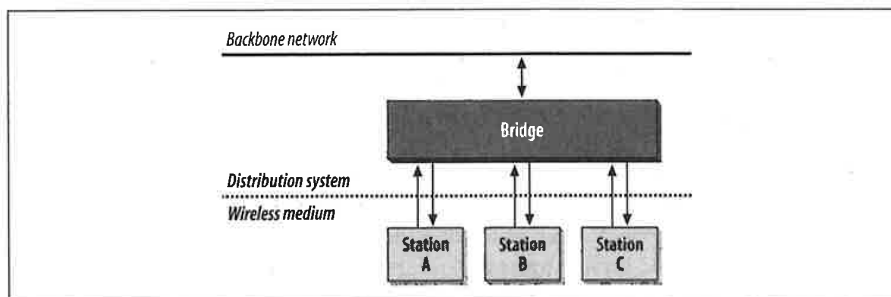
Figure 2-6. Distribution system in common 802.11 access point implementations
