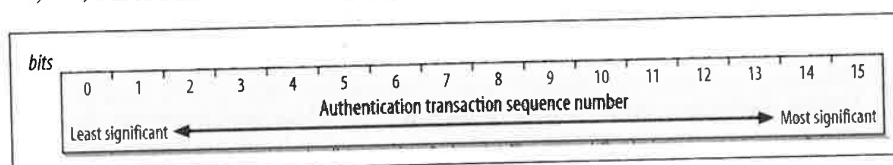
Figure 4-22. Authentication Transaction Sequence Number field
