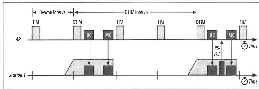
Figure 7-12. Multicast and broadcast buffer transmission after DTIMs
