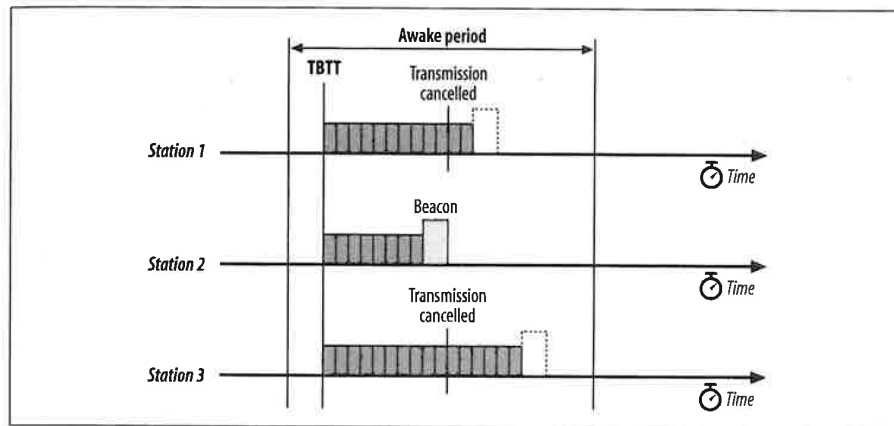
Figure 7-18. Distributed Beacon generation
