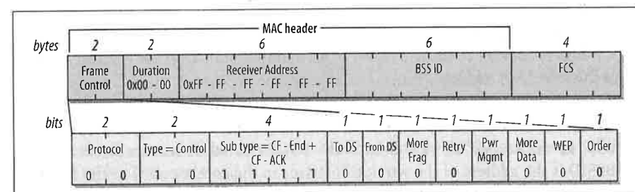
Figure 8-8. CF-End+CF-Ack frame
