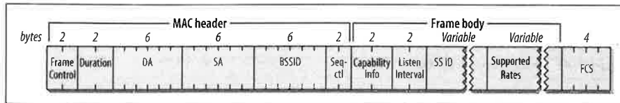
Figure 4-44. Association Request frame
