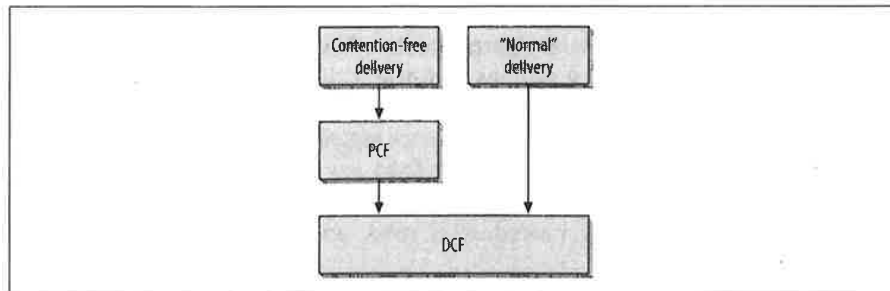
Figure 3-4. MAC coordination functions
