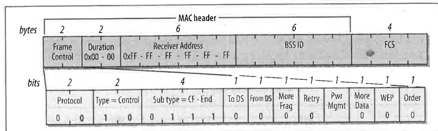
Figure 8-7. CF-End frame
