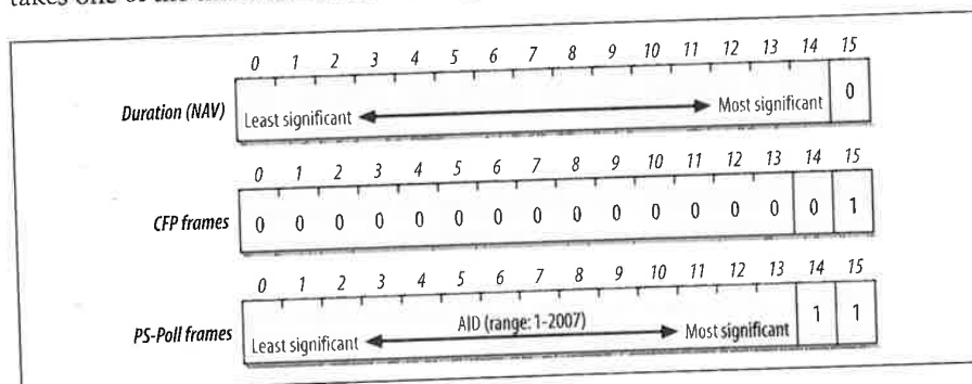
Figure 3-11. Duration/ID field
