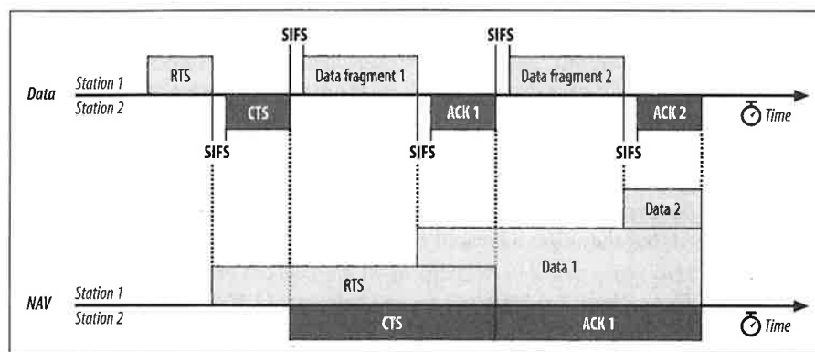
Figure 3-18. RTS/CTS with fragmentation
