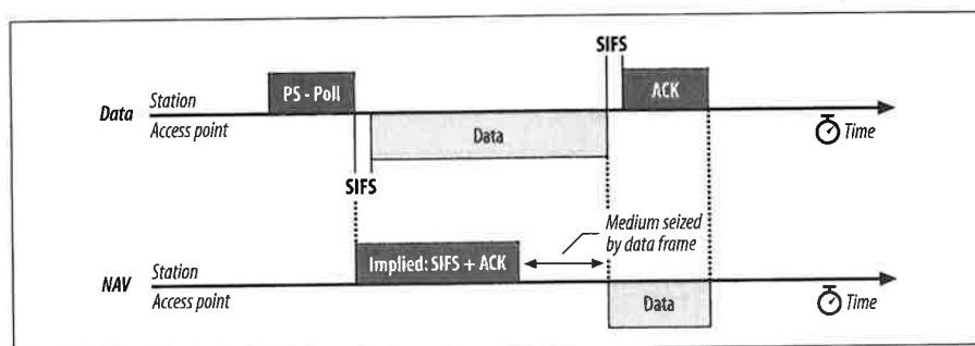
Figure 3-19. Immediate PS-Poll response
