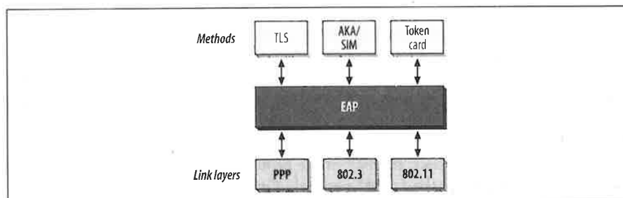
Figure 6-1. EAP architecture
