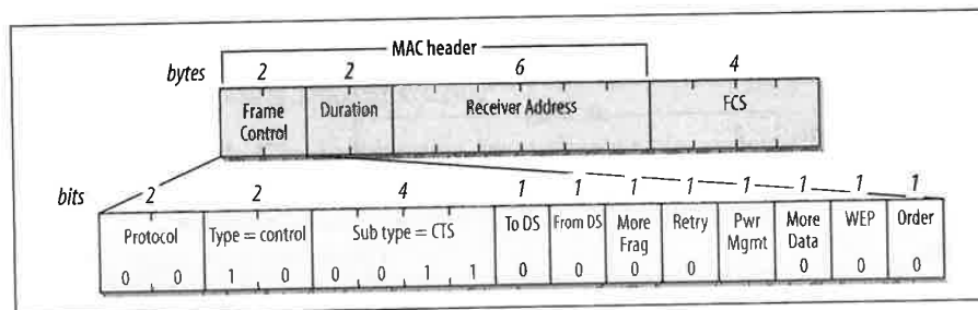
Figure 4-15. CTS frame
