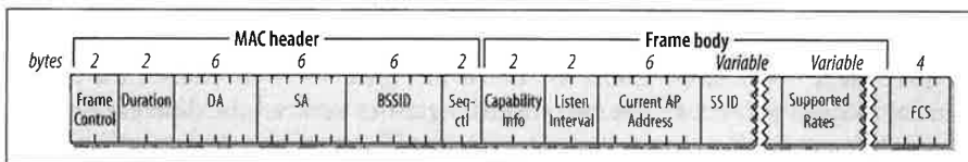
Figure 4-45. Reassociation Request frame
