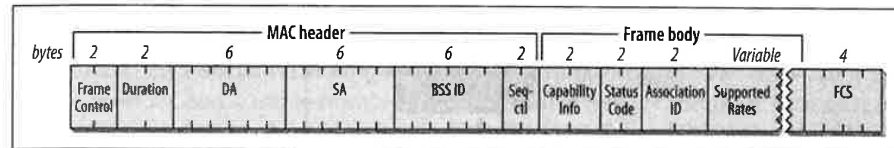
Figure 4-46. (Re)Association Response frame
