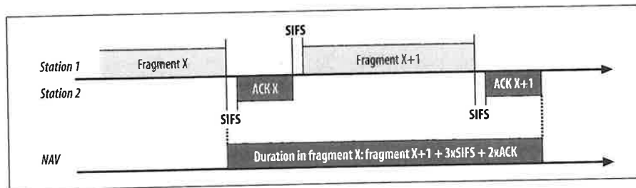
Figure 4-3. Duration settings on nonfinal fragment
