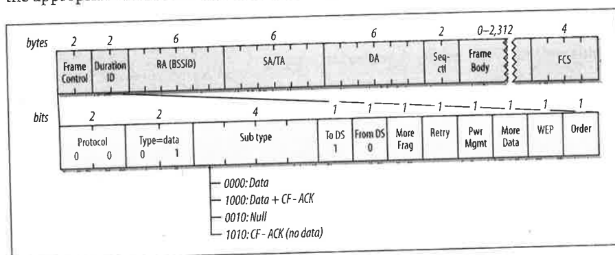
Figure 4-10. Data frames to the AP
