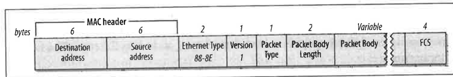
Figure 6-7. EAPOL frame format
