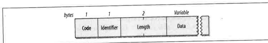
Figure 6-2. EAP packet format
