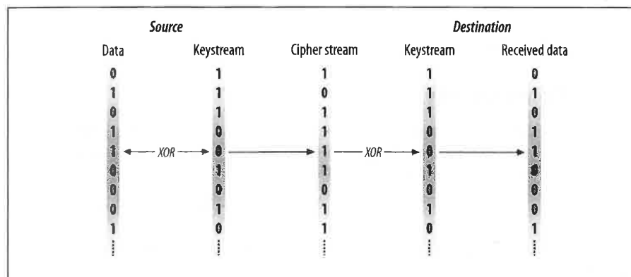
Figure 5-1. Generic stream cipher operation
