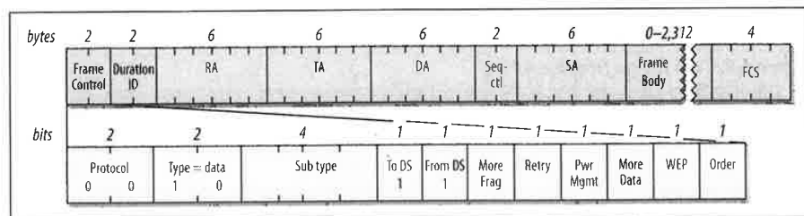
Figure 4-11. WDS frames
