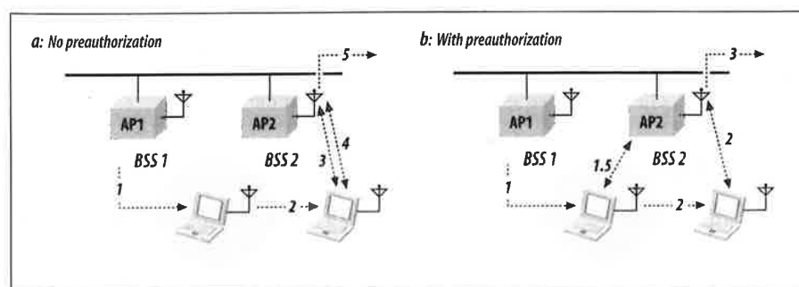
Figure 7-6. Time savings of preauthentication
