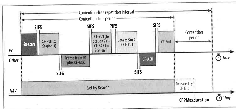
Figure 8-1. Using the PCF
