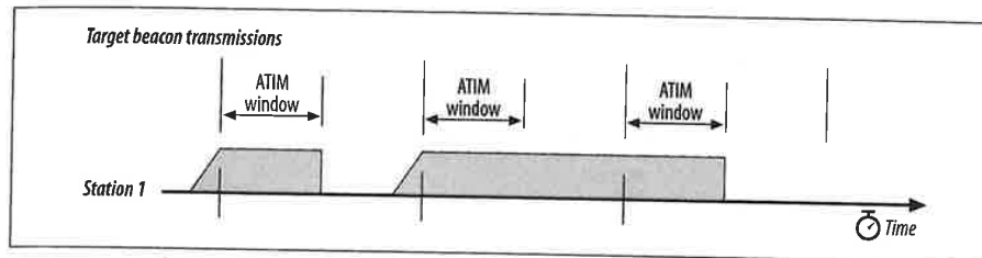
Figure 7-15. ATIM effects on power-saving modes
