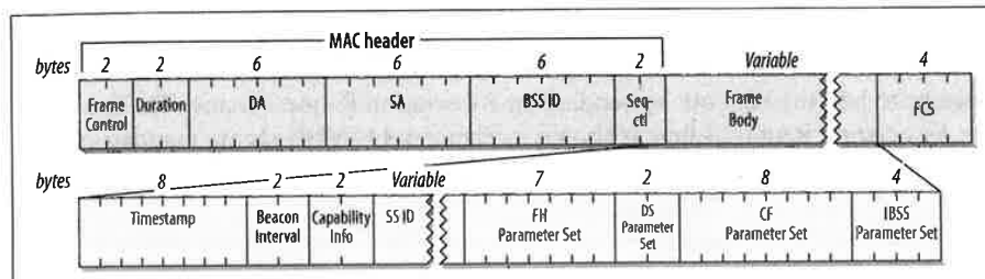
Figure 4-41. Probe Response frame
