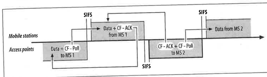
Figure 8-6. CF-Ack+CF-Poll usage
