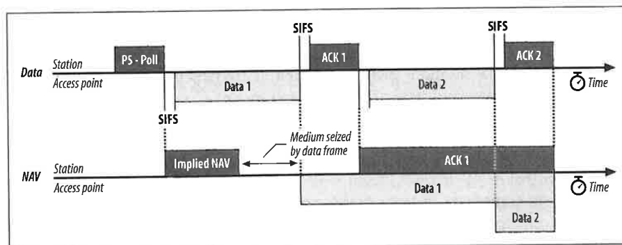
Figure 3-20. Immediate PS-Poll response with fragmentation
