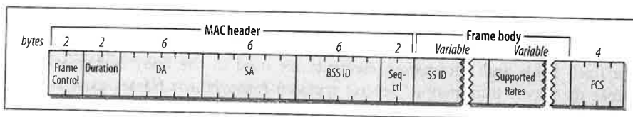
Figure 4-40. Probe Request frame
