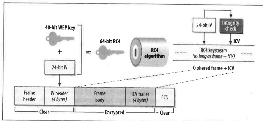
Figure 5-3. WEP operations
