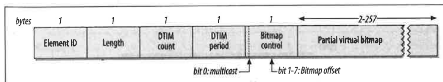
Figure 4-36. Traffic Indication Map information element
