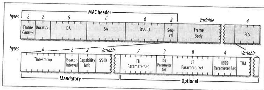
Figure 4-39. Beacon frame
