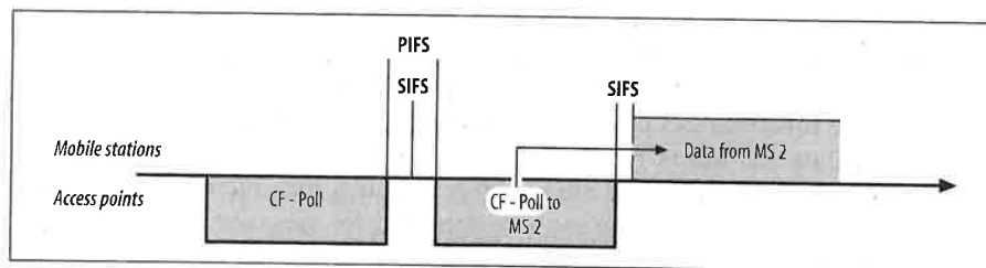
Figure 8-5. CF-Poll framing usage
