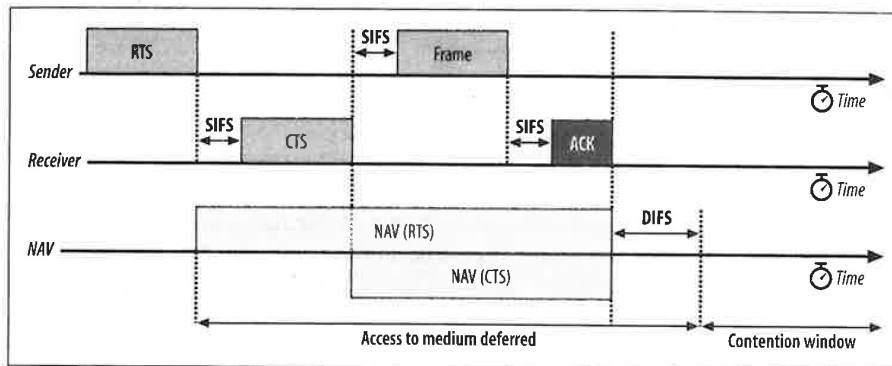
Figure 3-5. Using the NAV for virtual carrier sensing
