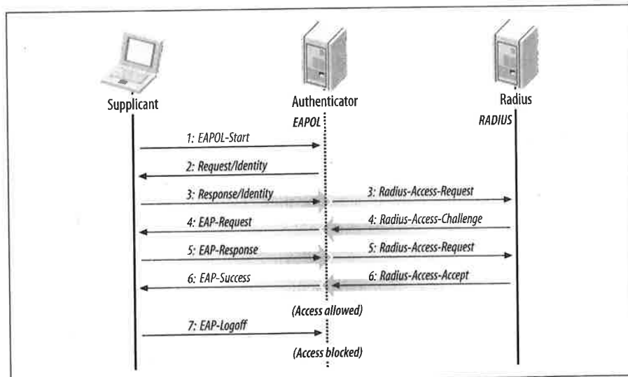
Figure 6-8. Typical EAPOL exchange
