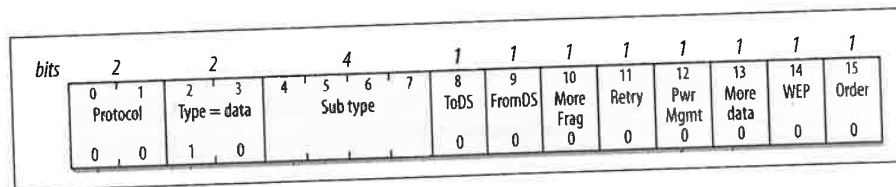
Figure 4-12. Frame Control field in control frames
