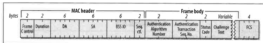
Figure 4-47. Authentication frames
