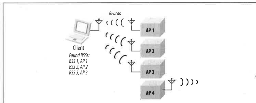
Figure 7-2. Passive scanning
