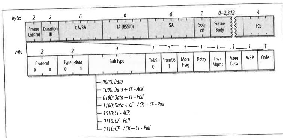
Figure 4-9. Data frames from the AP
