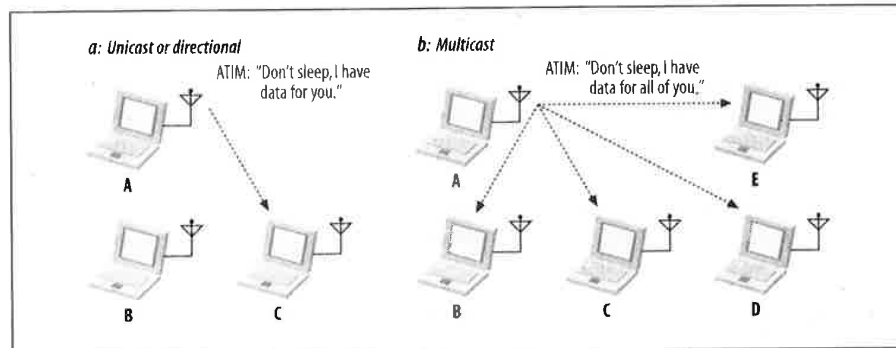
Figure 7-13. ATIM usage
