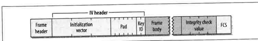
Figure 5-4. WEP frame extensions
