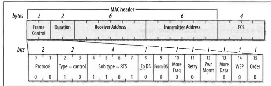
Figure 4-13. RTS frame
