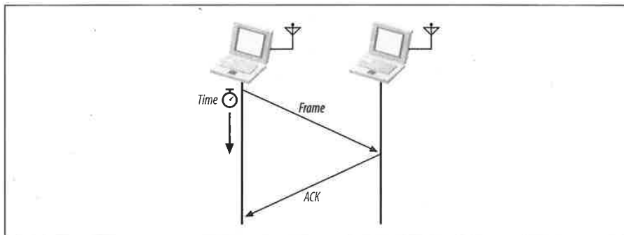
Figure 3-1. Positive acknowledgment of data transmissions
