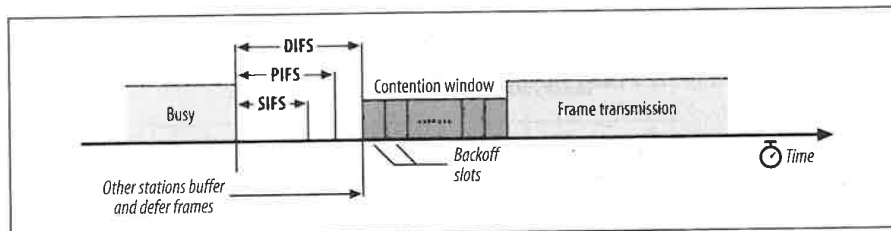
Figure 3-6. Interframe spacing relationships
