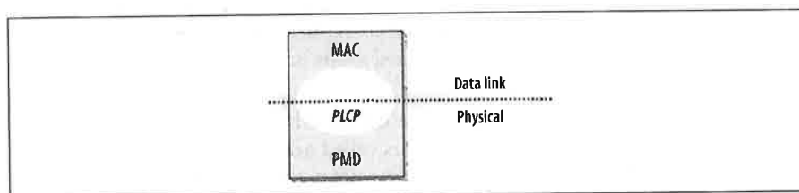
Figure 2-2. PHY components
