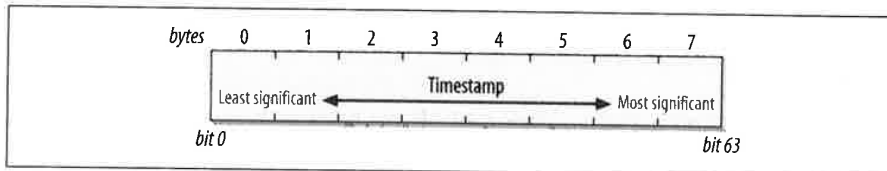
Figure 4-28. Timestamp field
