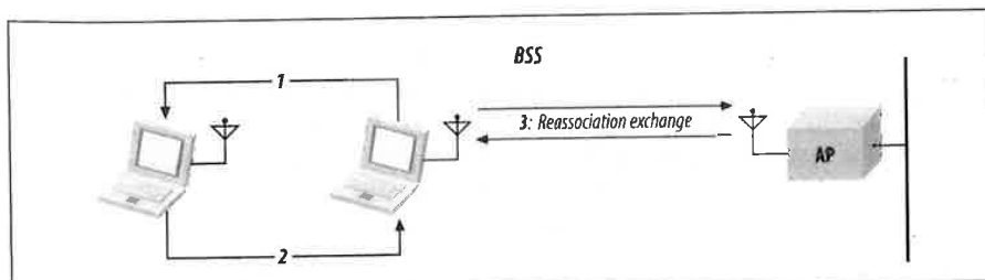
Figure 7-9. Reassociation with the same access point
