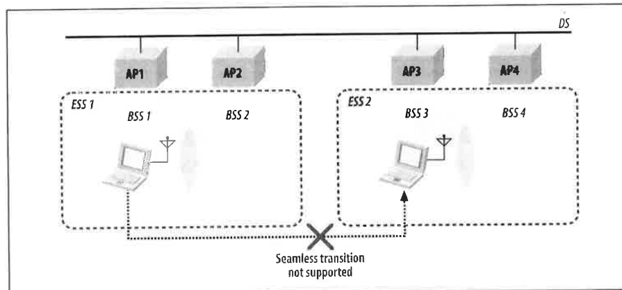
Figure 2-10. ESS transition
