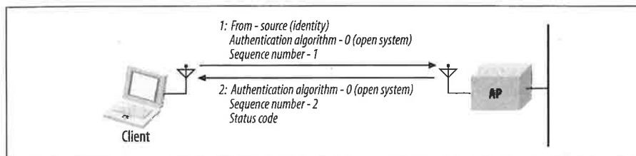
Figure 7-4. Open-system authentication exchange
