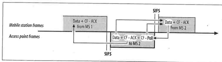
Figure 8-4. Usage of Data+CF-Ack+CF-Poll
