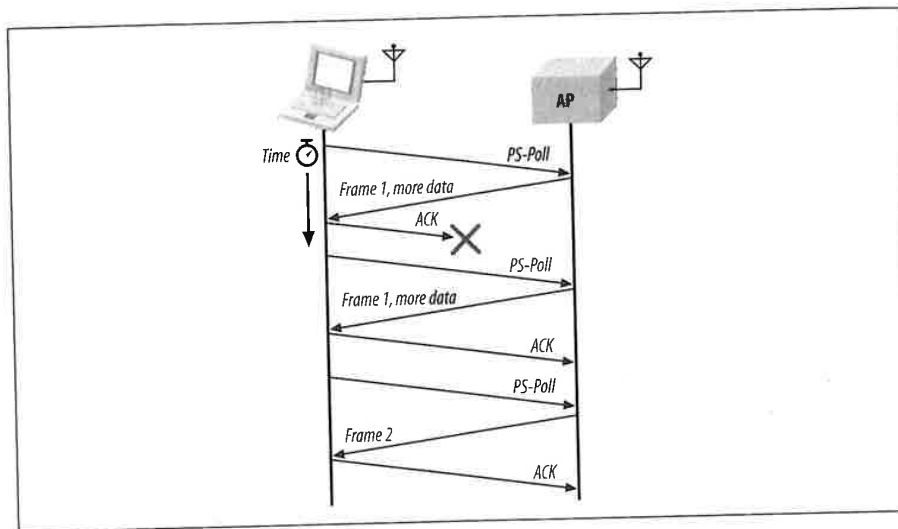
Figure 7-10. PS-Poll frame retrieval
