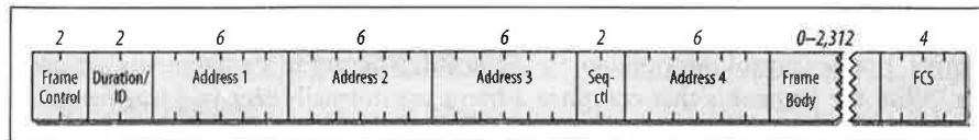
Figure 3-9. Generic 802.11 MAC frame
