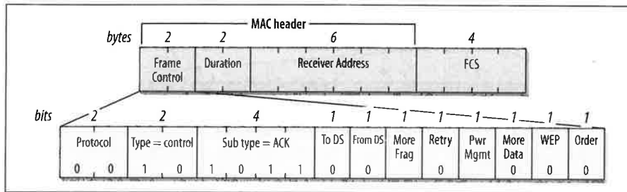
Figure 4-17. ACK frame
