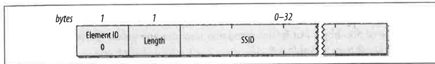
Figure 4-32. Service Set Identity information element
