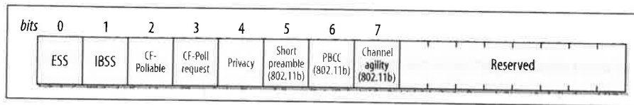
Figure 4-24. Capability Information field
