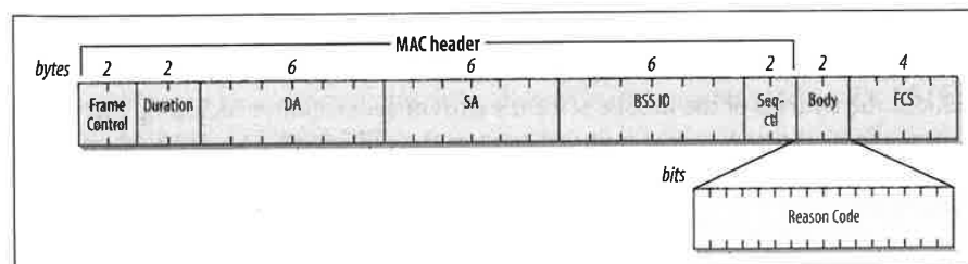
Figure 4-43. Disassociation and Deauthentication frames
