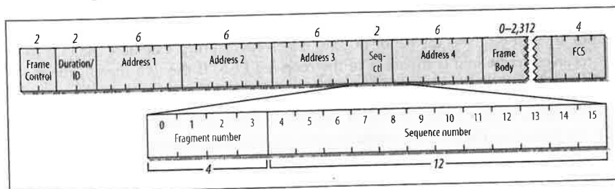
Figure 3-12. Sequence Control field
