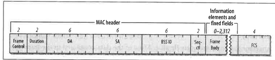
Figure 4-20. Generic management frame
