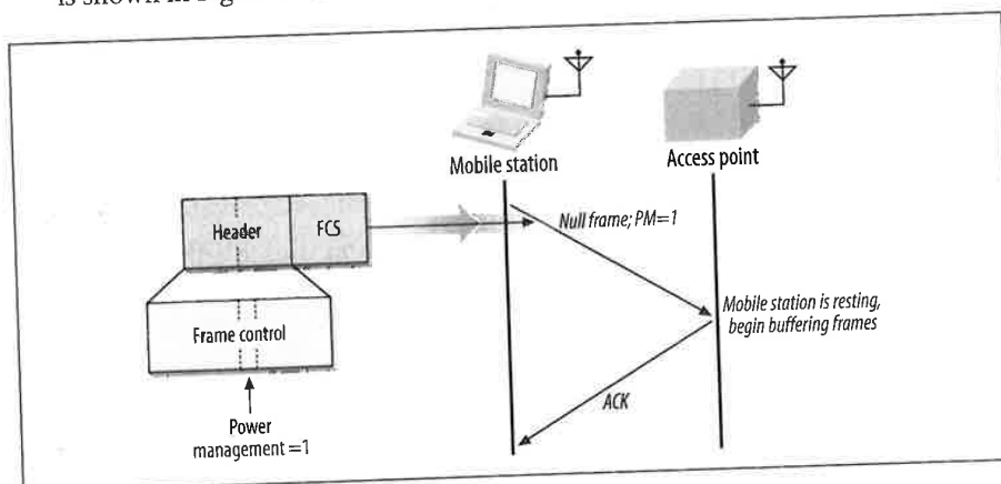
Figure 4-7. Data frame of subtype Null
