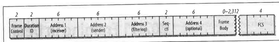
Figure 4-1. Generic data frame
