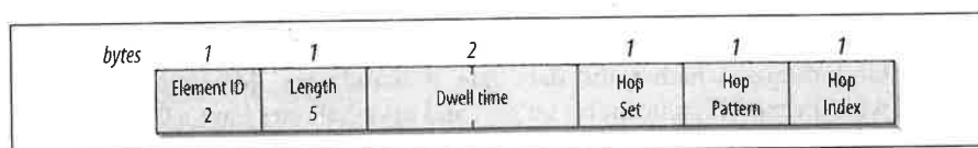
Figure 4-34. FH Parameter Set information element
