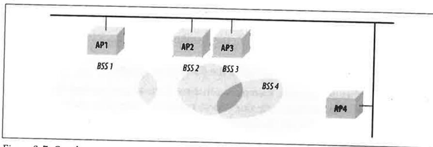
Figure 2-7. Overlapping BSSs in an ESS
