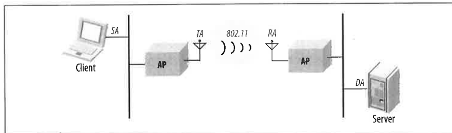
Figure 4-6. Wireless distribution system
