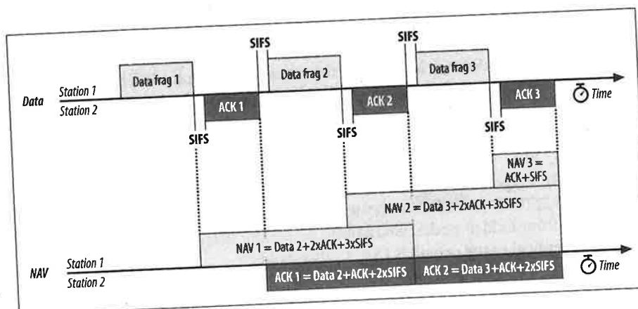
Figure 3-16. Fragmentation
