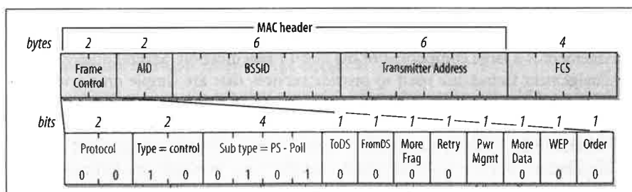
Figure 4-19. PS-Poll frame
