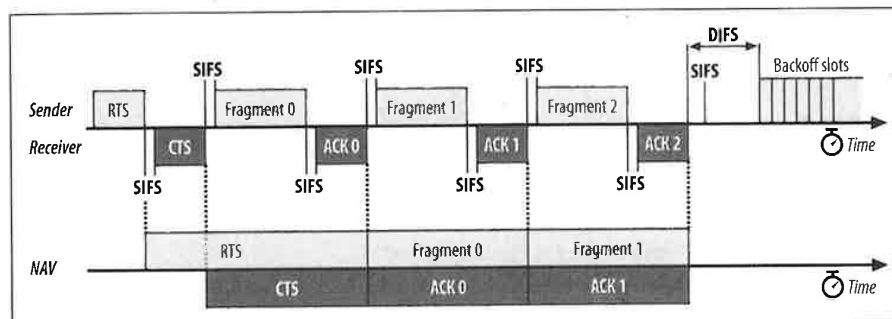
Figure 3-8. Fragmentation burst
