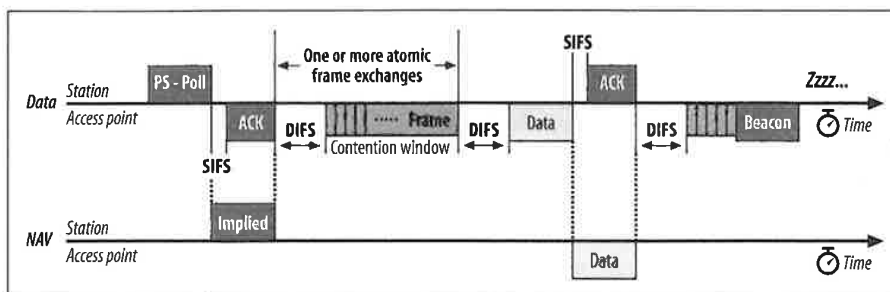
Figure 3-21. Deferred PS-Poll response example
