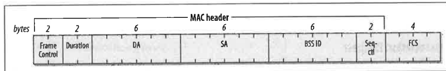
Figure 4-42. ATIM frame
