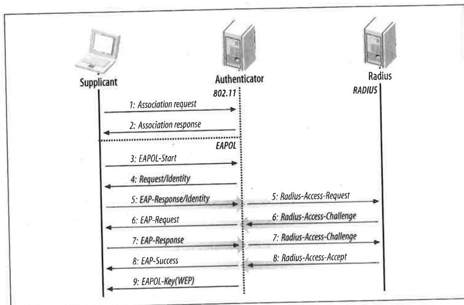
Figure 6-9. EAPOL exchange on an 802.11 network
