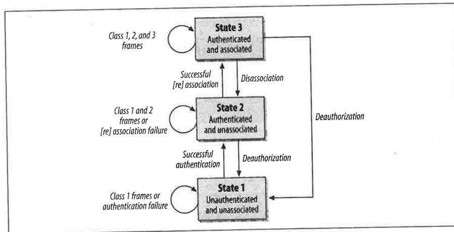
Figure 4-48. Overall 802.11 state diagram
