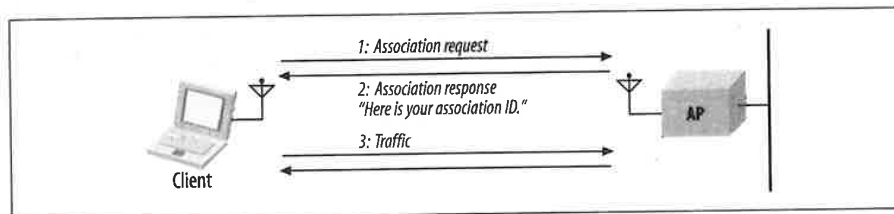
Figure 7-7. Association procedure
