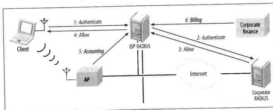
Figure 6-10. 802.11x supporting public Ethernet ports
