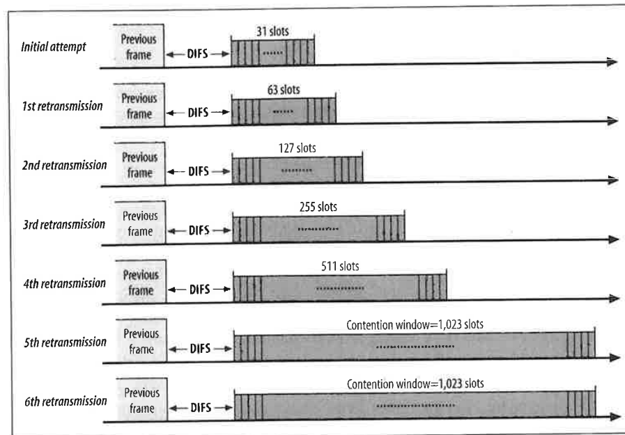
Figure 3-7. DSSS contention window size
