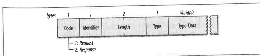
Figure 6-3. EAP Request and EAP Response packets
