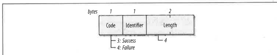
Figure 6-4. EAP Success and Failure frames
