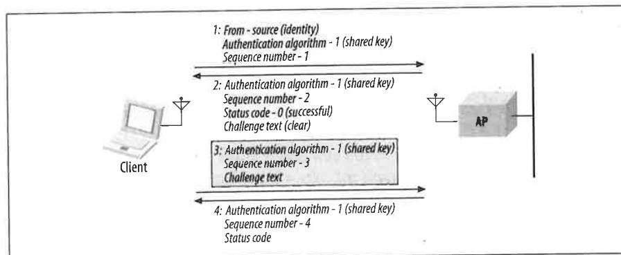
Figure 7-5. Shared-key authentication exchange
