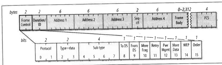
Figure 3-10. Frame control field
