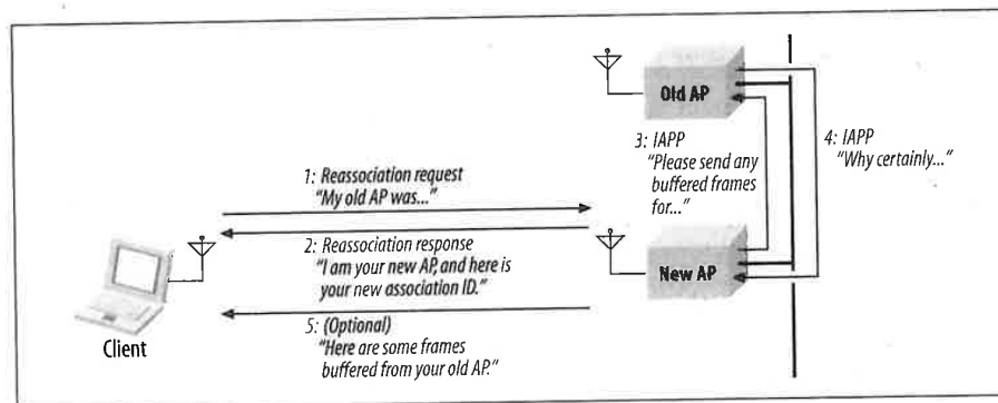
Figure 7-8. Reassociation procedure
