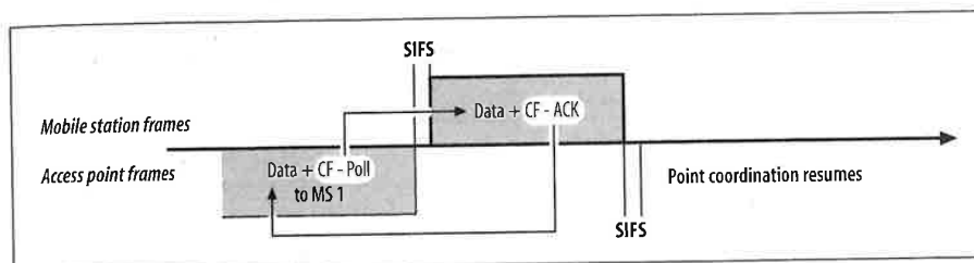
Figure 8-3. Data+CF-Ack usage
