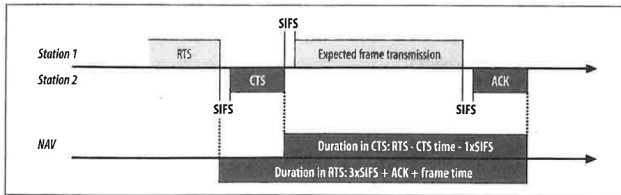
Figure 4-16. CTS duration
