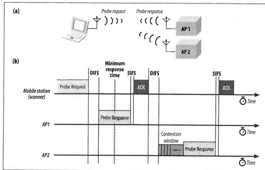
Figure 7-3. Active scanning procedure and medium access
