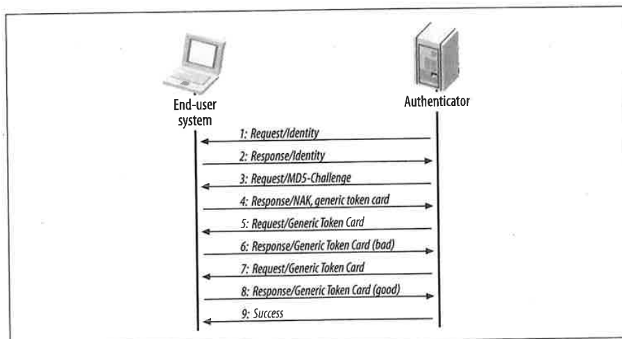
Figure 6-5. Sample EAP exchange
