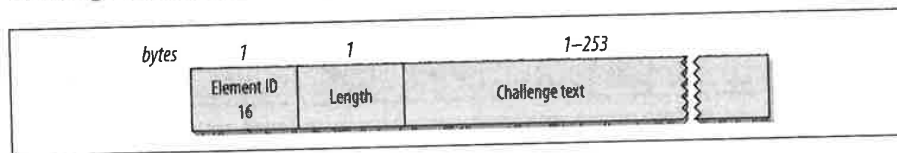
Figure 4-38. Challenge Text information element
