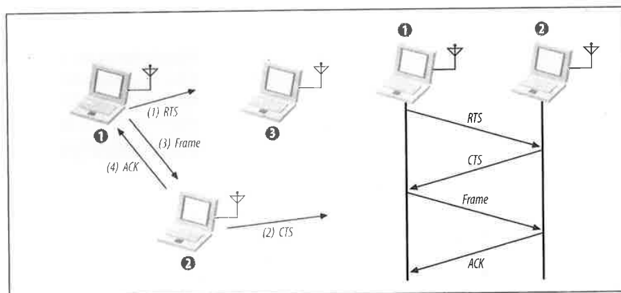
Figure 3-3. RTS/CTS clearing
