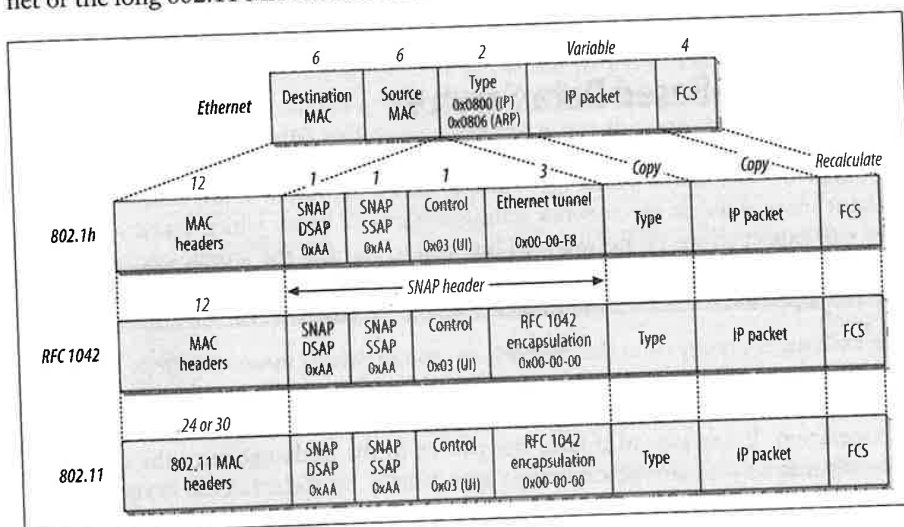
Figure 3-13. IP encapsulation in 802.11
