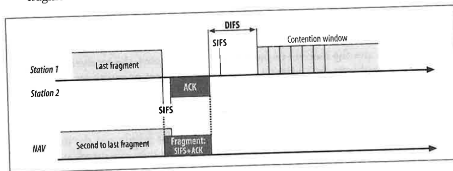
Figure 4-2. Duration setting on final fragment
