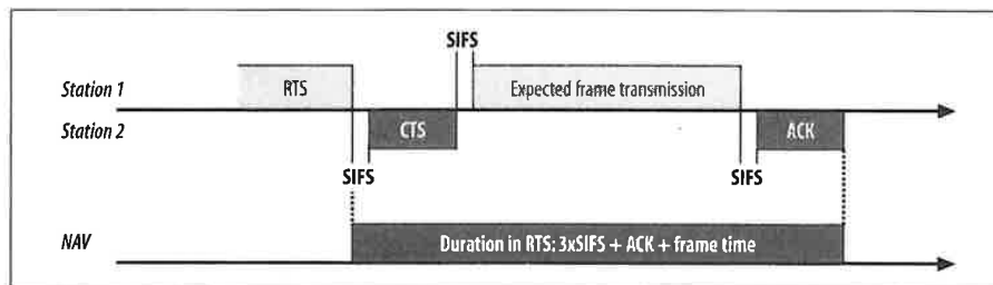
Figure 4-14. Duration field in RTS frame
