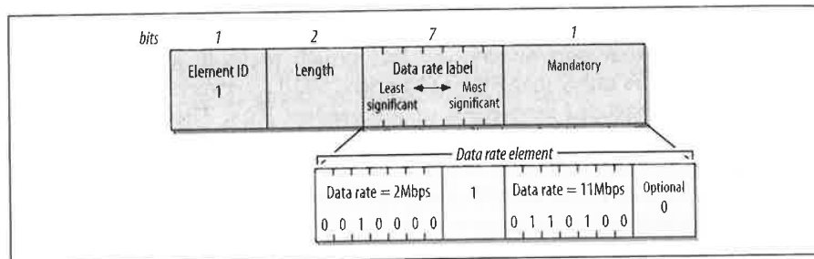
Figure 4-33. Supported Rates information element
