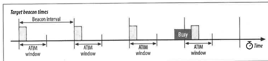
Figure 7-14. ATIM window
