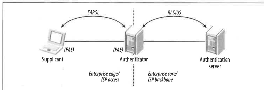
Figure 6-6. 802.1x architecture
