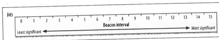
Figure 4-23. Beacon Interval field
