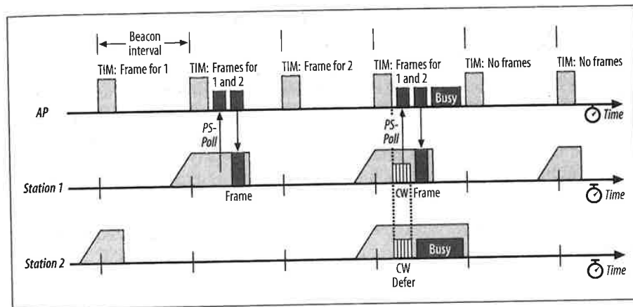
Figure 7-11. Buffered frame retrieval process
