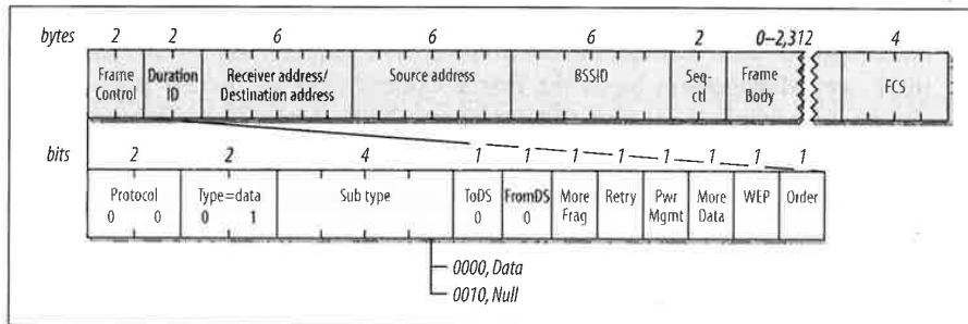
Figure 4-8. IBSS data frame
