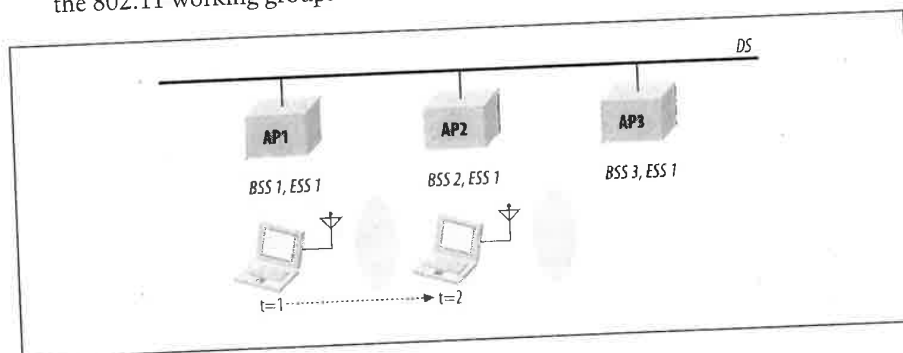
Figure 2-9. BSS transition
