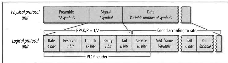
Figure 11-11. OFDM PLCP framing format
