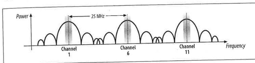
Figure 10-16. Channel separation in 802.11 DS networks
