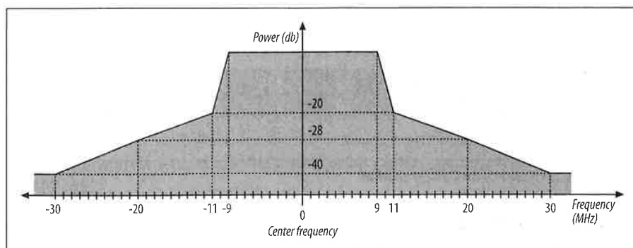
Figure 11-9. Transmit spectrum mask for 802.11a
