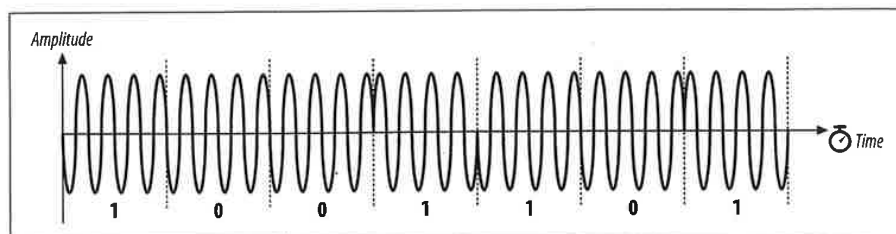
Figure 10-20. The letter M encoded in DBPSK
