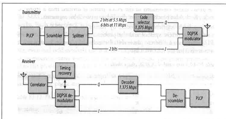
Figure 10-28. HR/DSSS transceiver
