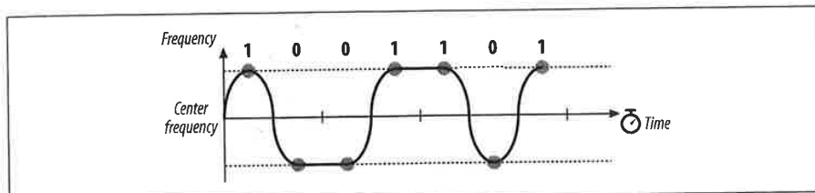
Figure 10-6. 2GFSK encoding of the letter M
