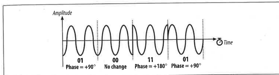
Figure 10-22. The letter M encoded in DQPSK
