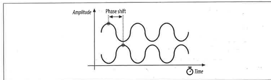
Figure 10-18. Phase difference between two sine waves
