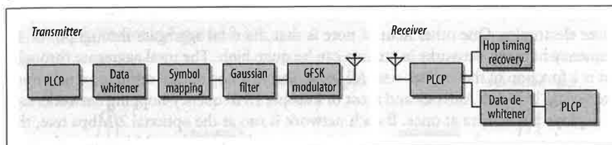
Figure 10-10. Frequency-hopping transceiver
