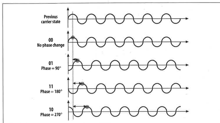
Figure 10-21. DQPSK encoding
