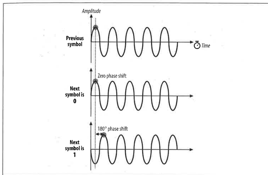
Figure 10-19. DBPSK encoding
