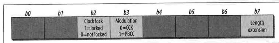
Figure 10-27. Service field in the HR/DSSS PLCP header
