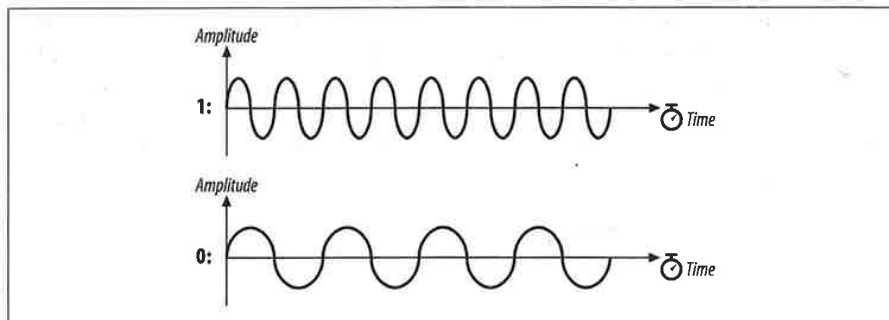
Figure 10-5. 2-level GFSK
