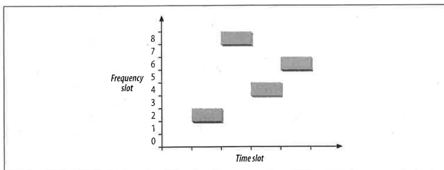
Figure 10-1. Frequency hopping
