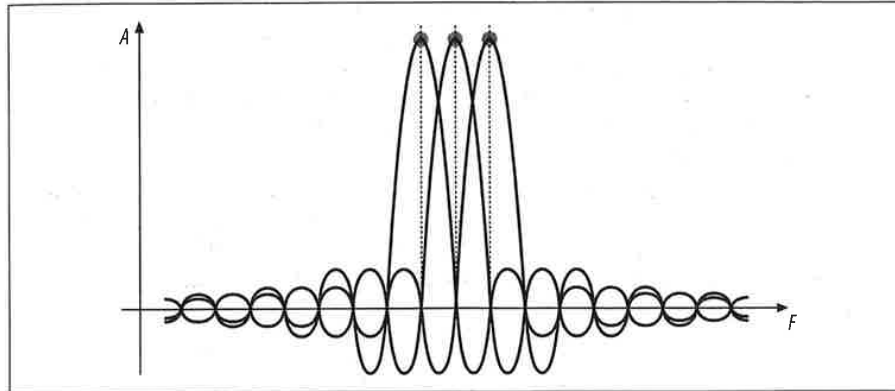
Figure 11-3. Orthogonality in the frequency domain
