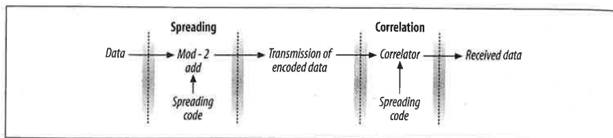
Figure 10-13. Chipping
