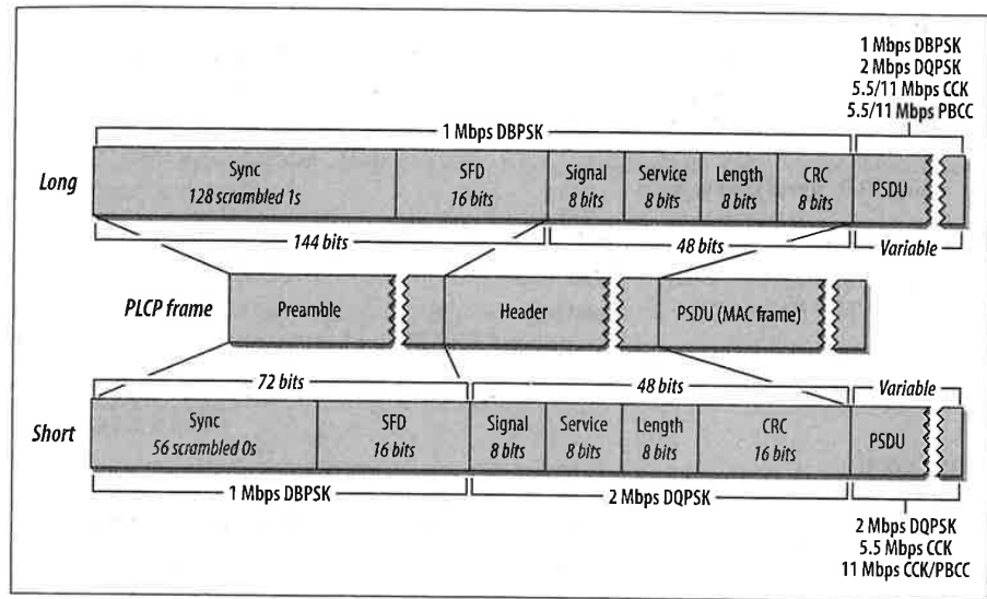
Figure 10-26. HR/DSSS PLCP framing
