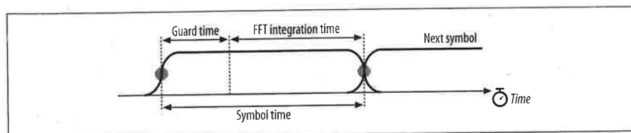
Figure 11-7. Cosine windowing technique
