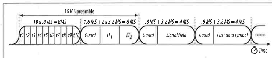
Figure 11-12. Preamble and frame start
