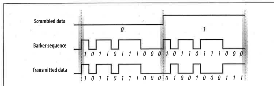
Figure 10-14. Encoding with the Barker word
