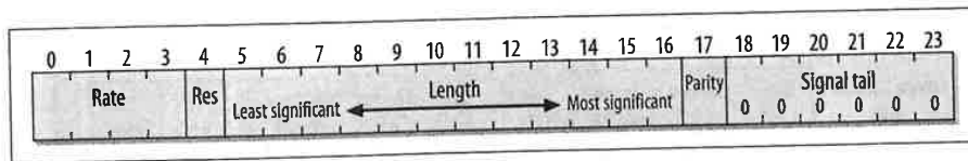
Figure 11-13. Signal field of OFDM PLCP frame
