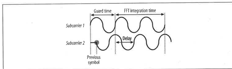
Figure 11-6. Cyclic prefix extension
