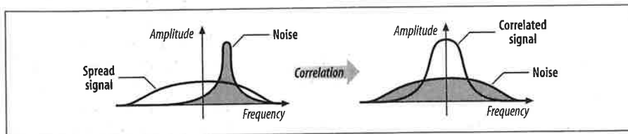
Figure 10-12. Spreading of noise by the correlation process
