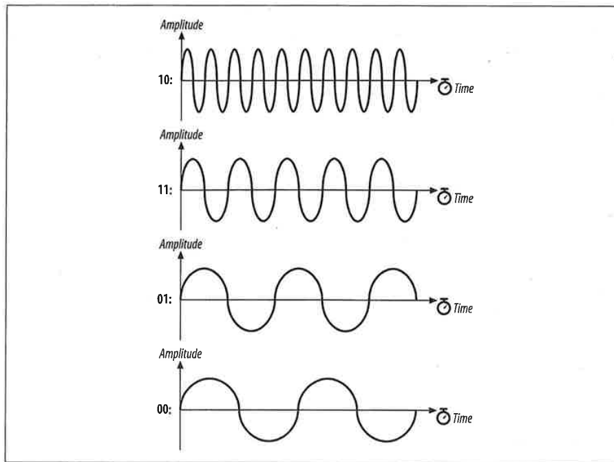
Figure 10-7. Mapping of symbols to frequencies in 4GFSK
