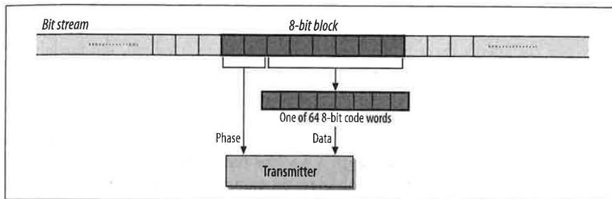
Figure 10-30. 802.11b transmission at 11 Mbps
