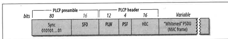
Figure 10-9. PLCP framing in the FH PHY
