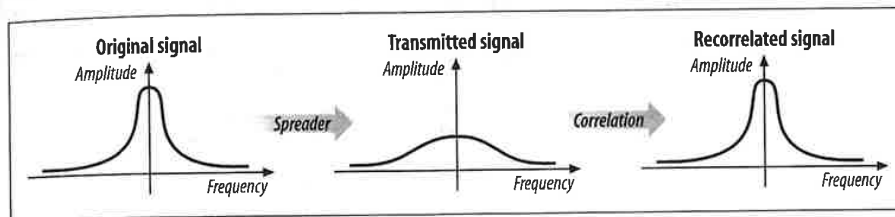
Figure 10-11. Basic DSSS technique
