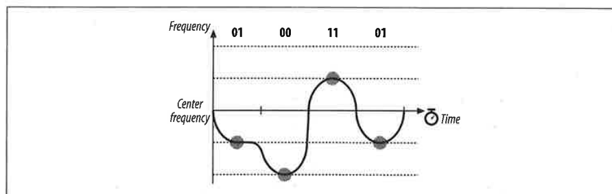
Figure 10-8. 4GFSK encoding of the letter M
