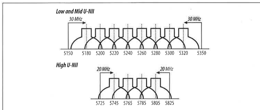
Figure 11-10. Operating bands from Table 11-1
