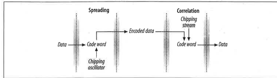
Figure 10-25. Code symbols in CCK
