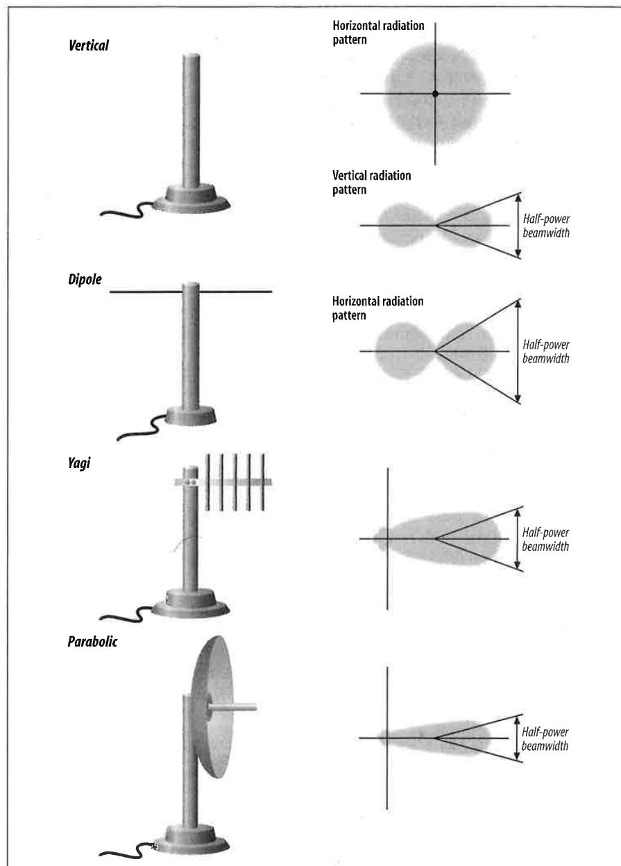
Figure 15-5. Antenna types
