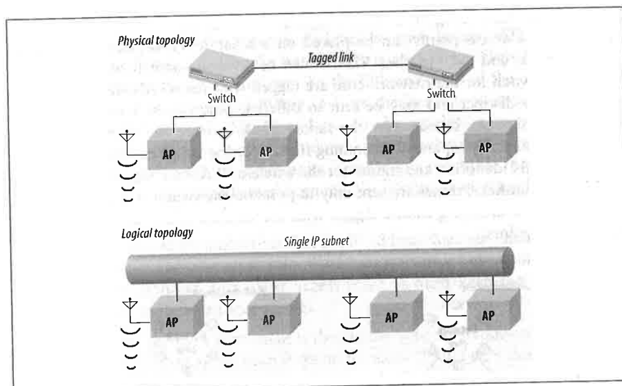
Figure 15-3. Using VLANs to span multiple switches
