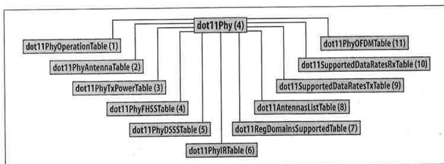
Figure A-7. Physical-layer MIB branches
