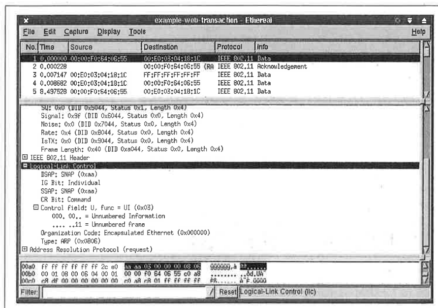
Figure 16-8. LLC SNAP header
