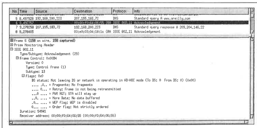
Figure 16-23. ACK of DNS request
