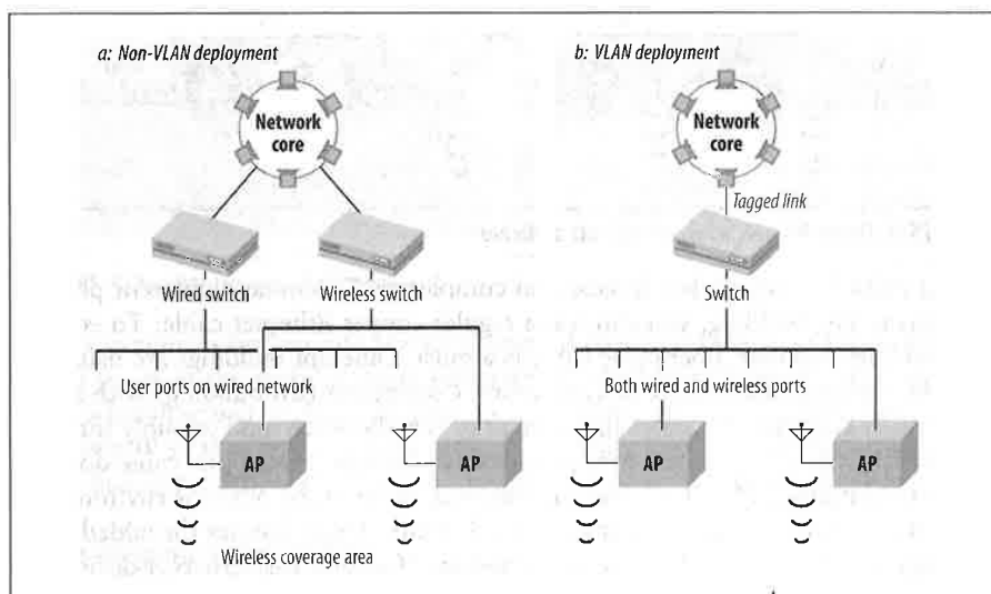
Figure 15-2. Physical topologies for 802.11 network deployment
