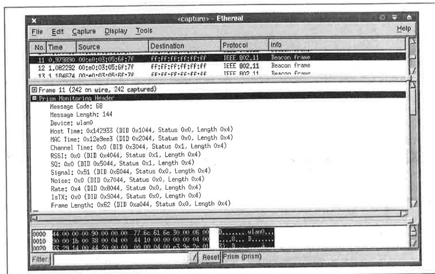
Figure 16-7. PRISM monitoring header
