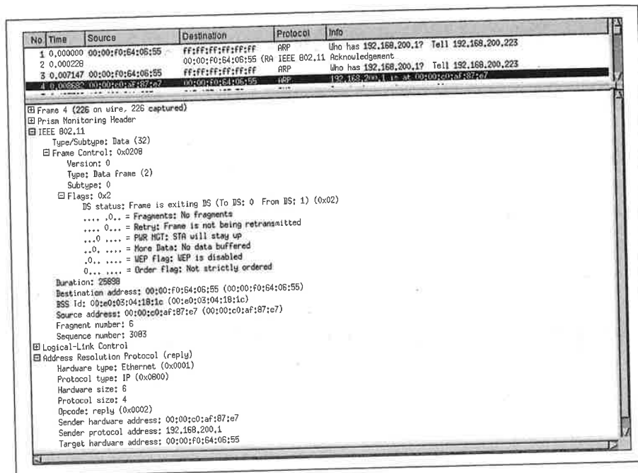
Figure 16-21. ARP reply
