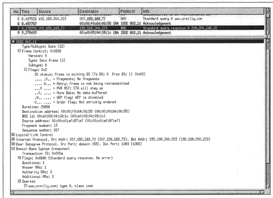
Figure 16-24. DNS reply
