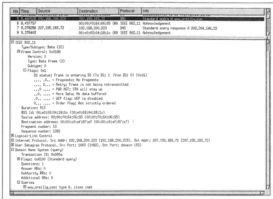
Figure 16-22. DNS request
