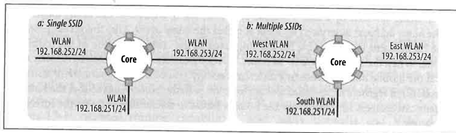
Figure 15-4. Noncontiguous deployments
