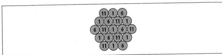
Figure 15-6. Frequency planning
