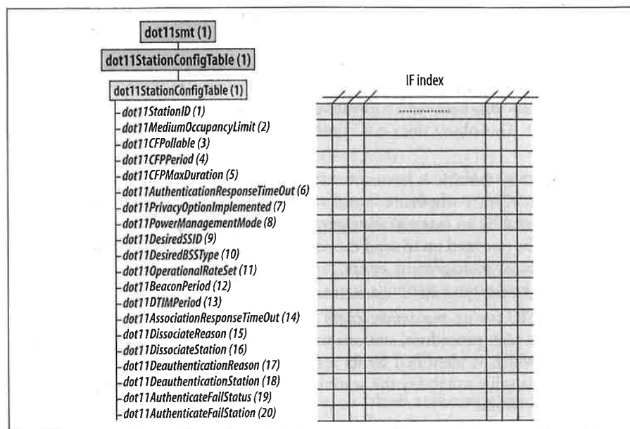
Figure A-3. The station configuration table dot11StationConfigTable
