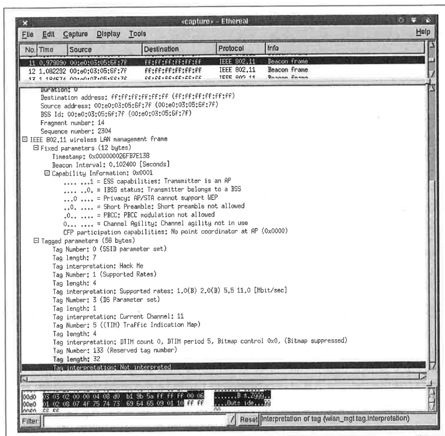
Figure 16-6. Beacon frame decode
