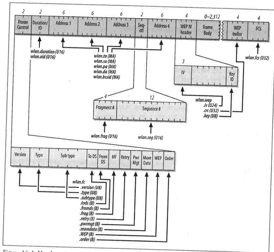
Figure 16-4. Header component variables
