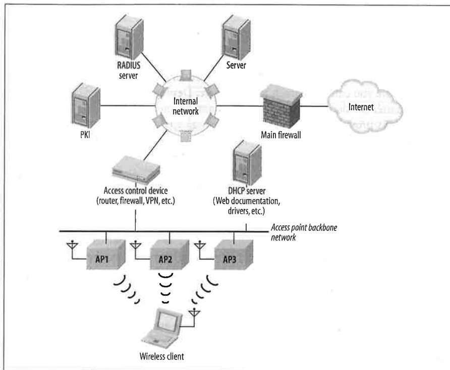
Figure 15-1. Standard wireless LAN deployment topology
