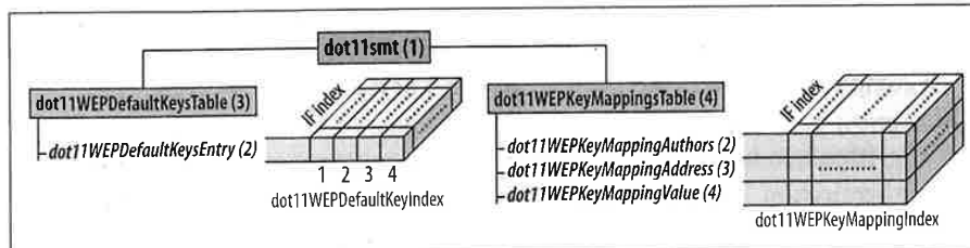
Figure A-5. WEP key tables
