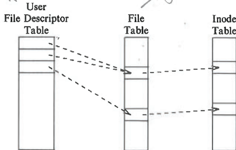
Figure 2.2. File Descriptors, File Table, and Inode Table
