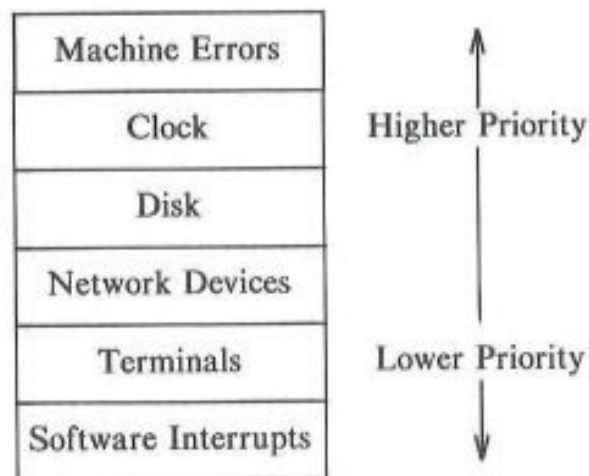
Figure 1.6. Typical Interrupt Levels
