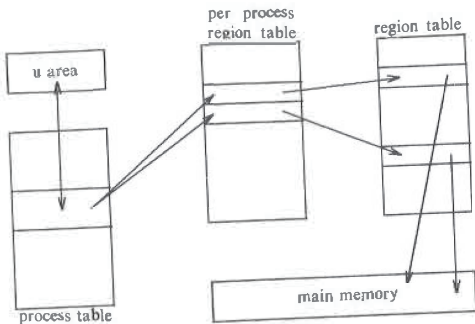
Figure 2.5. Data Structures for Processes
