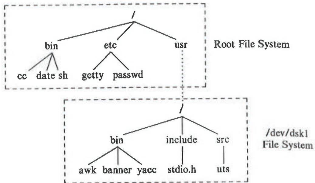
Figure 5.22. File System Tree Before and After Mount
