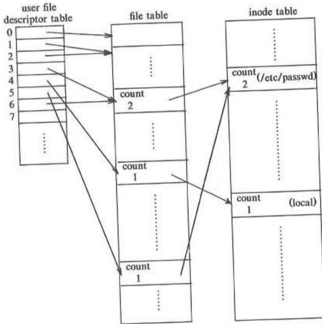
Figure 5.20. Data Structures after Dup
