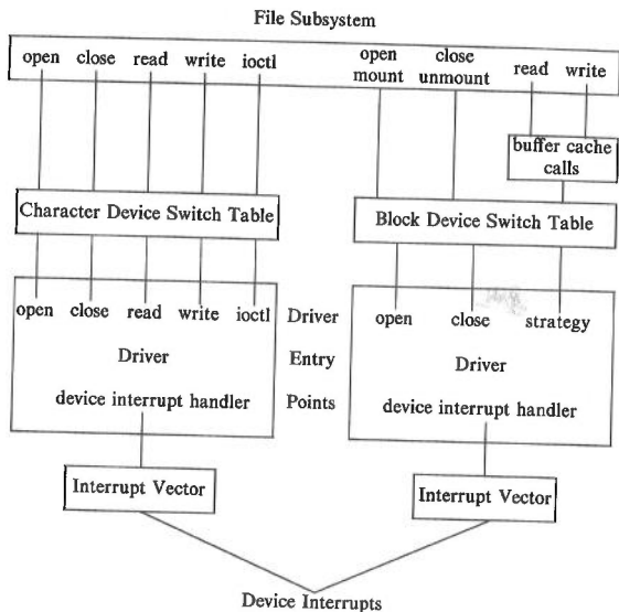
Figure 10.1. Driver Entry Points
