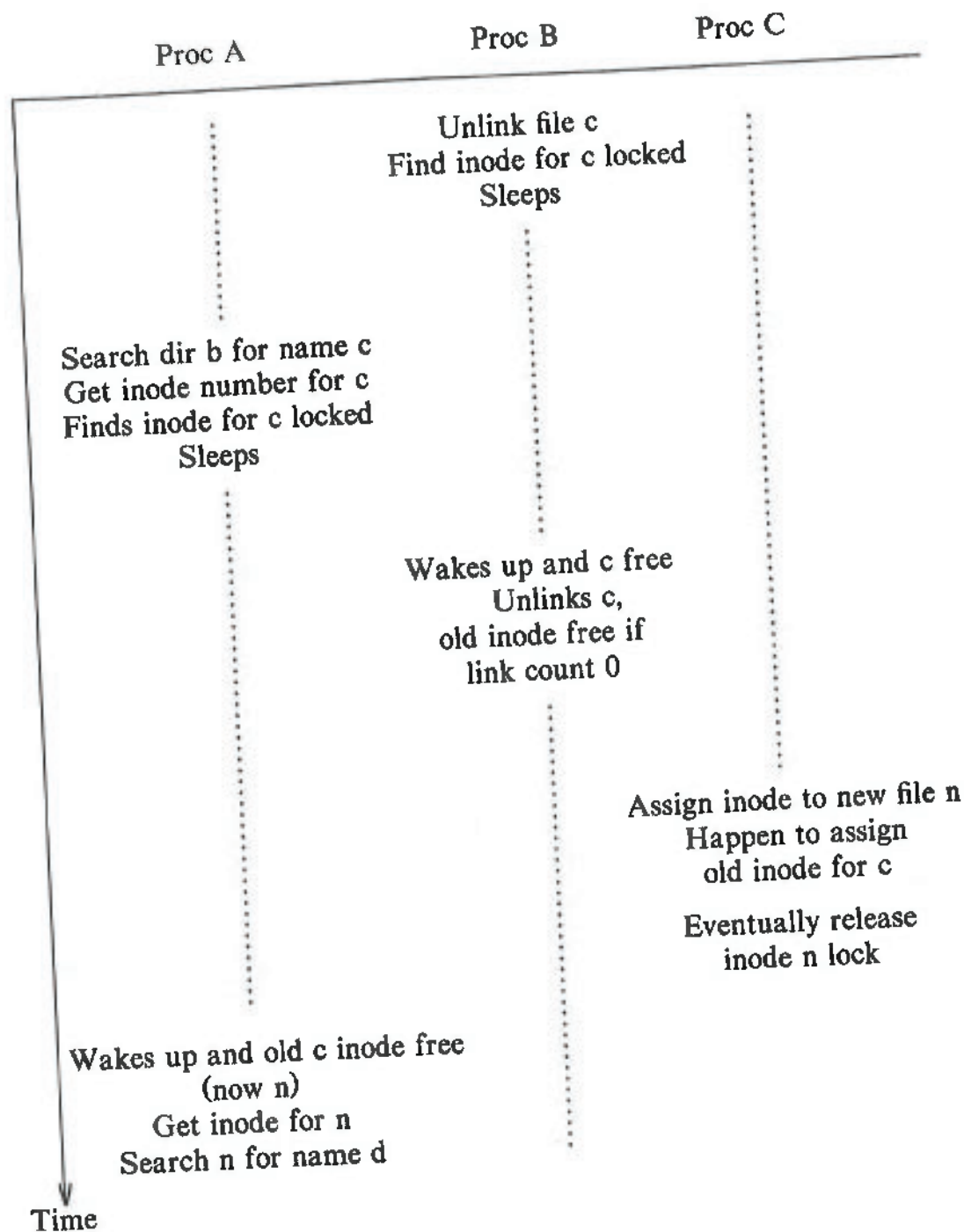
Figure 5.32. Unlink Race Condition
