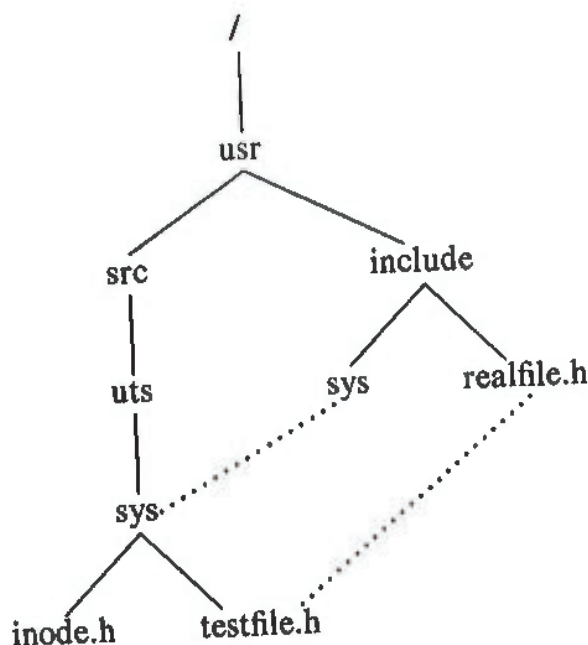
Figure 5.28. Linked Files in File System Tree
