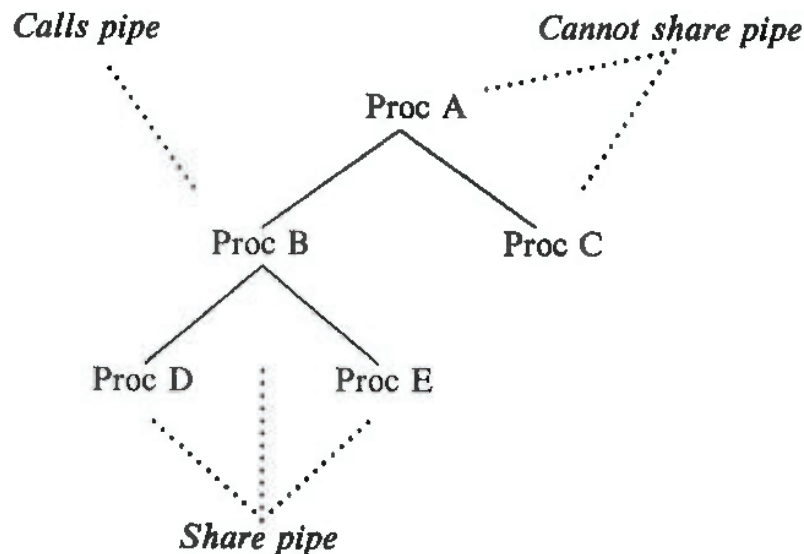
Figure 5.15. Process Tree and Sharing Pipes
