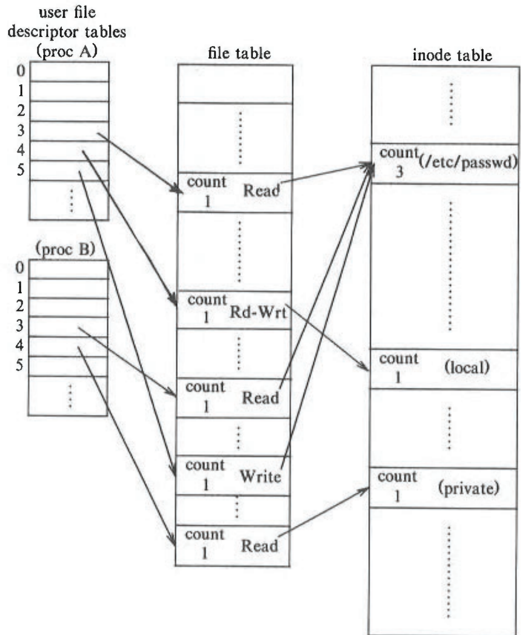
Figure 5.4. Data Structures after Two Processes Open Files
