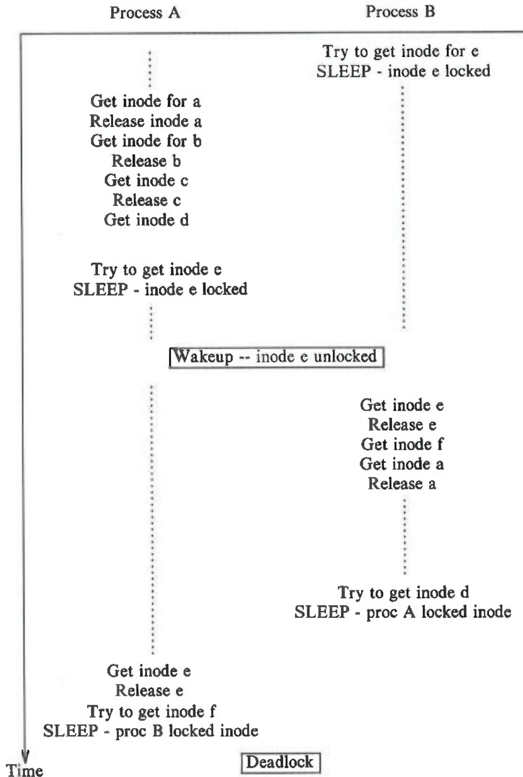
Figure 5.30. Deadlock Scenario for Link
