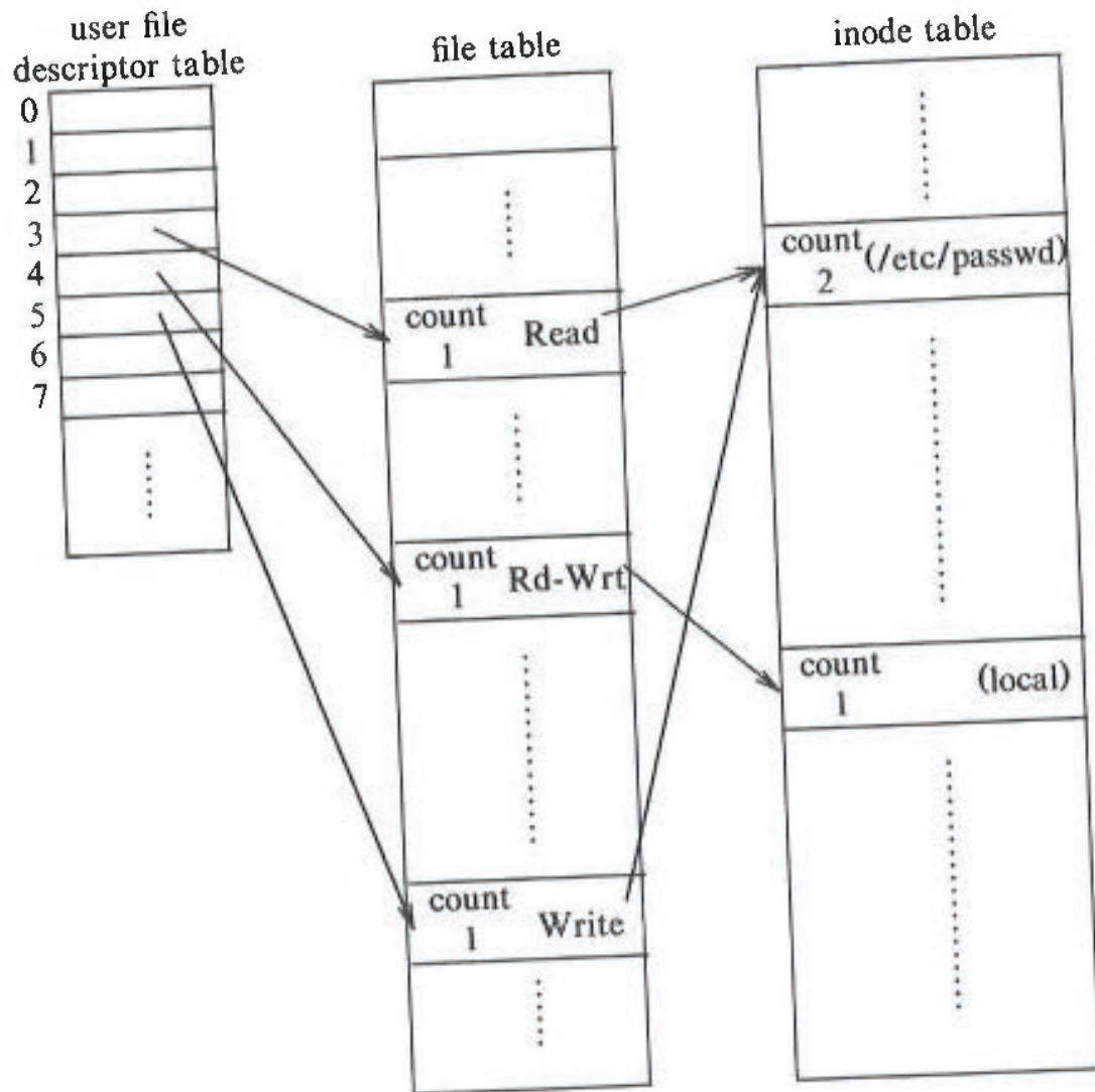
Figure 5.3. Data Structures after Open
