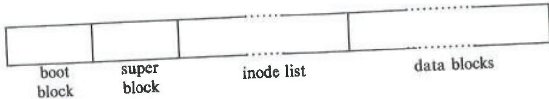
Figure 2.3. File System Layout
