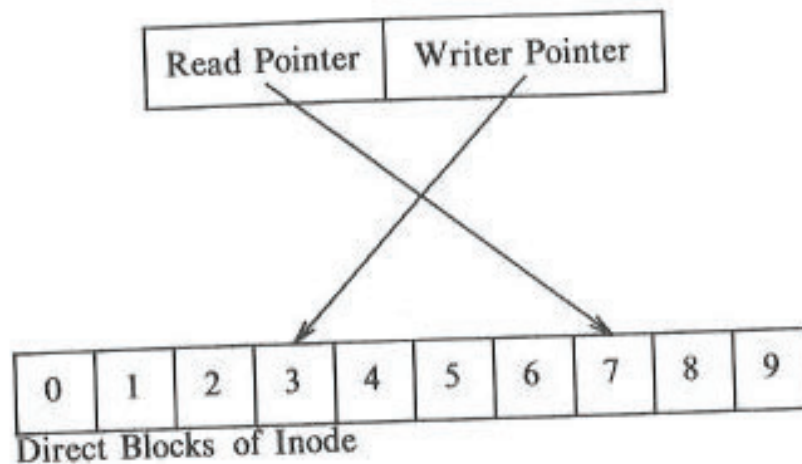
Figure 5.17. Logical View of Reading and Writing a Pipe
