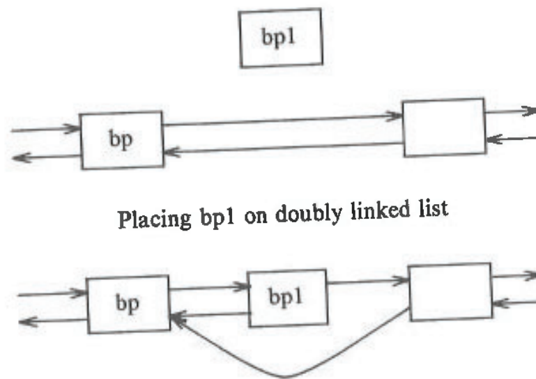
Figure 2.8. Incorrect Linked List because of Context Switch
