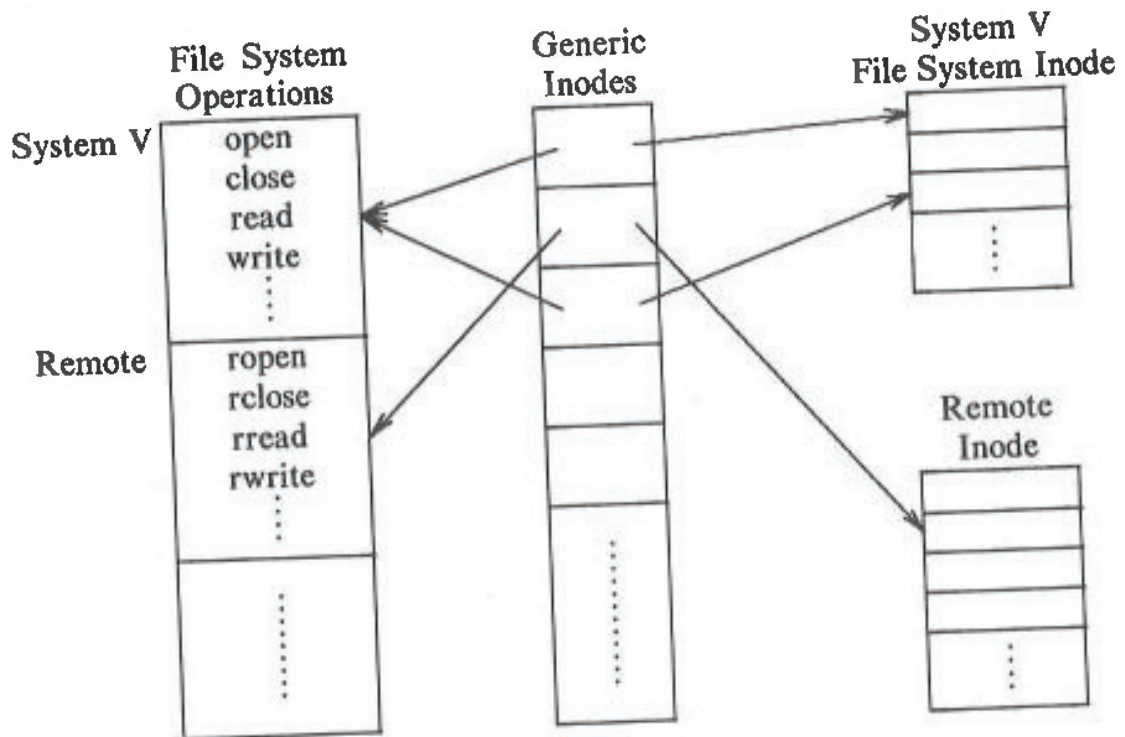
Figure 5.34. Inodes for File System Types
