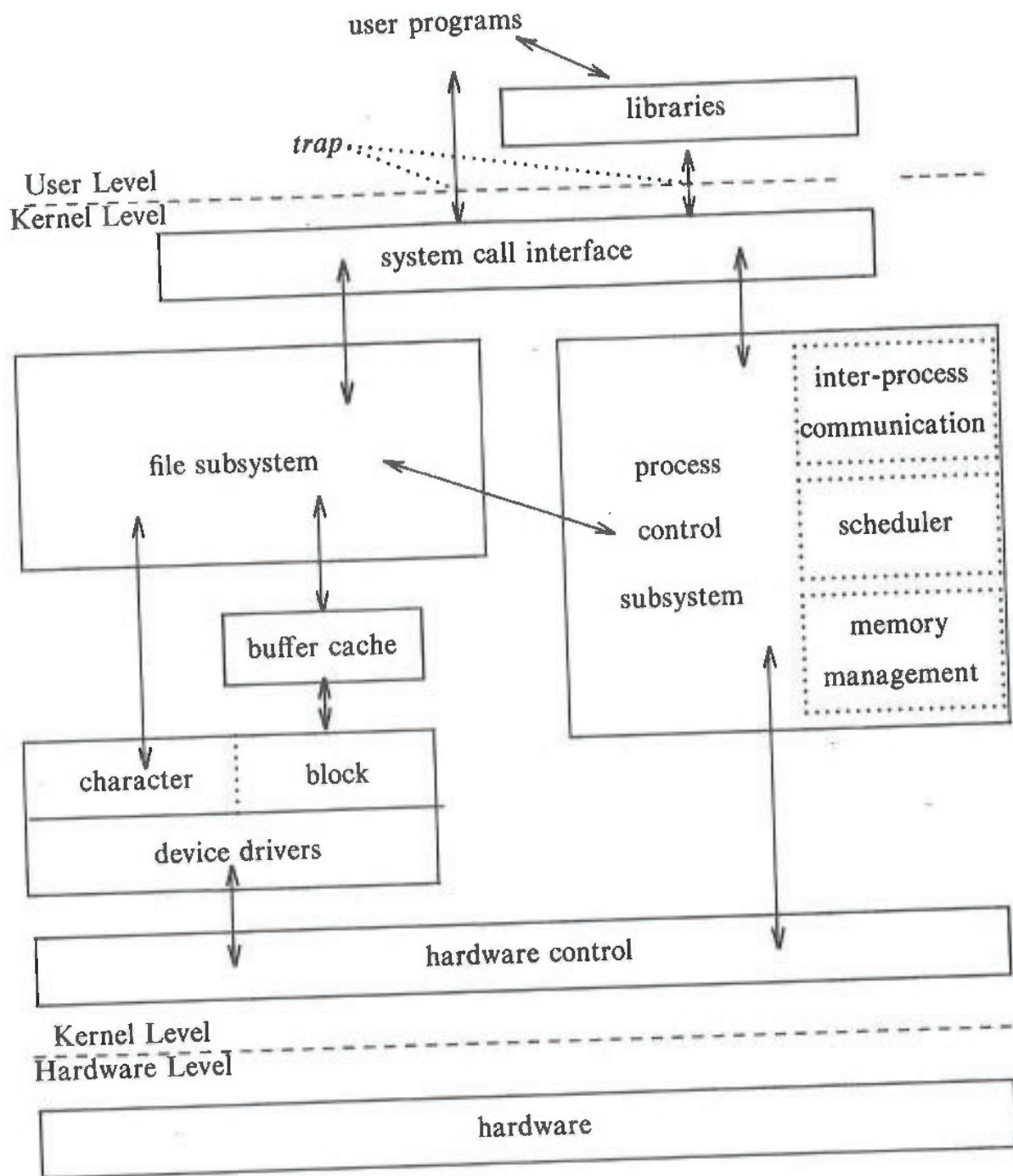
Figure 2.1. Block Diagram of the System Kernel
