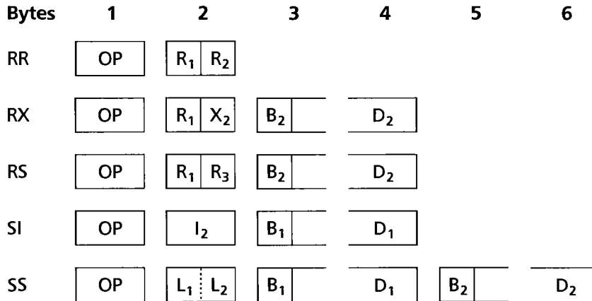
FIGURE 2.4 • IBM 370 instruction formats.
