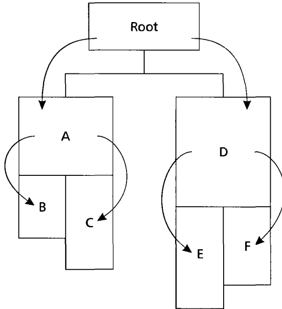
FIGURE 8.4 • Typical overlay tree format.
