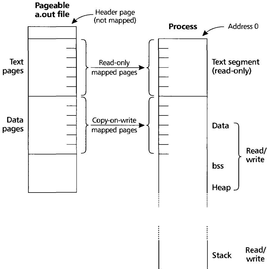
FIGURE 3.4 • Mapping a ZMAGIC a.out file into a process.
