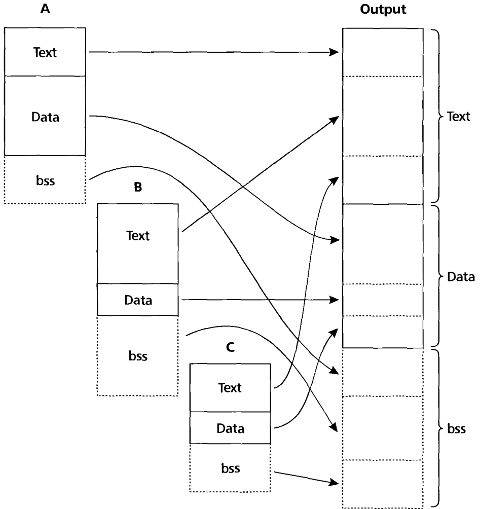
FIGURE 4.2 • Multiple-segment storage allocation.
