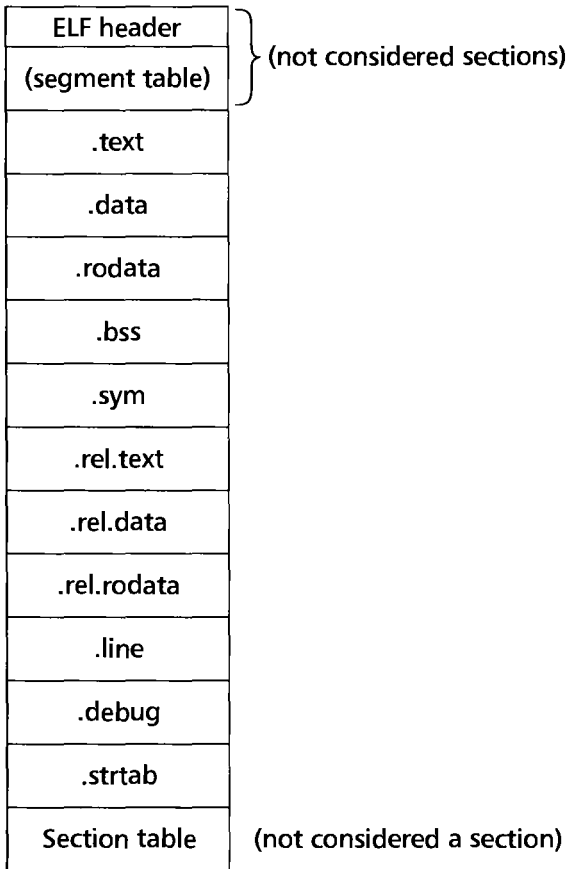
FIGURE 3.14 • Sample relocatable ELF file.
