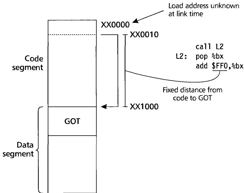
FIGURE 8.3 • PIC code and data with fixed offsets.
