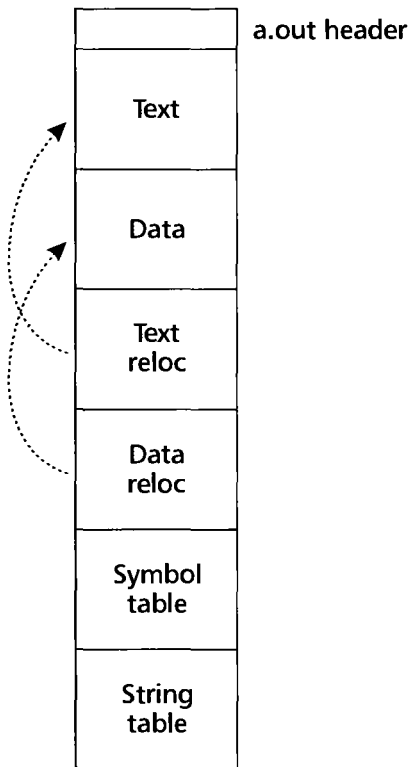
FIGURE 3.7 • Simplified relocatable a.out.
