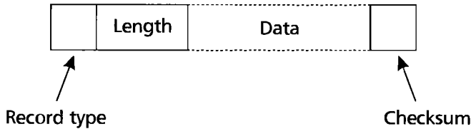
FIGURE 3.25 • OMF record format.
