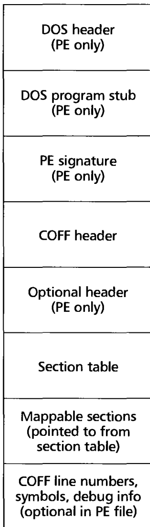
FIGURE 3.22 • Microsoft PE and COFF file.
