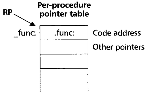
FIGURE 8.2 • Accessing code by means of data pointers.
