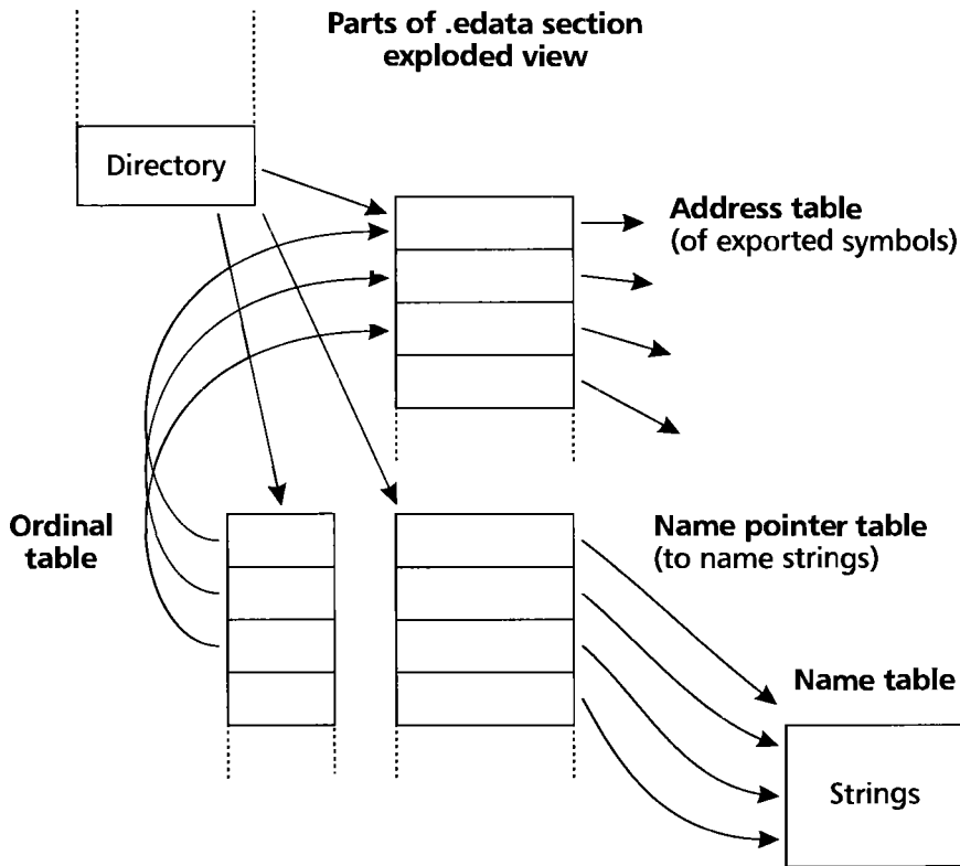
FIGURE 10.5 • Structure of .edata section.
