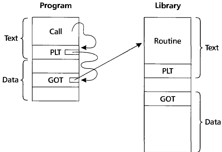
FIGURE 10.1 • PLT and GOT.
