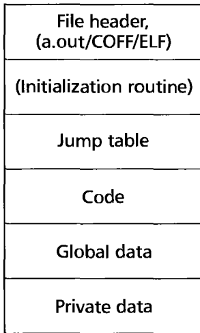
FIGURE 9.2 • Structure of typical shared library.
