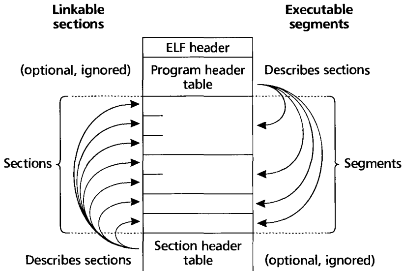
FIGURE 3.10 • Two views of an ELF file.
