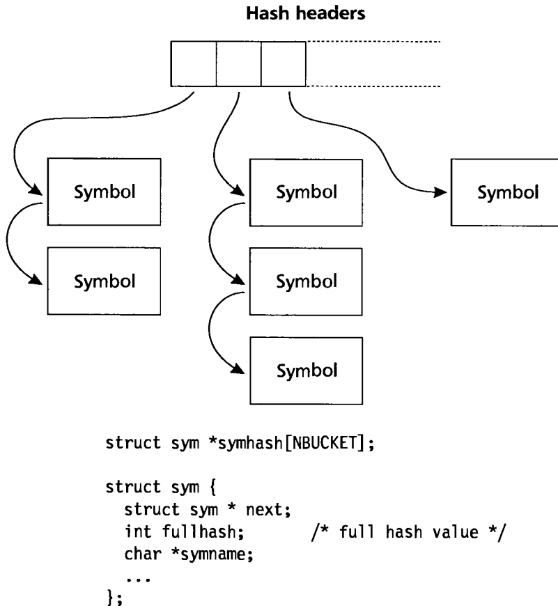
FIGURE 5.1 • Symbol table.
