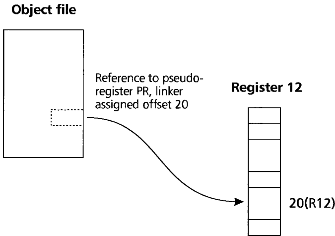
FIGURE 4.5 • Pseudo-registers.
