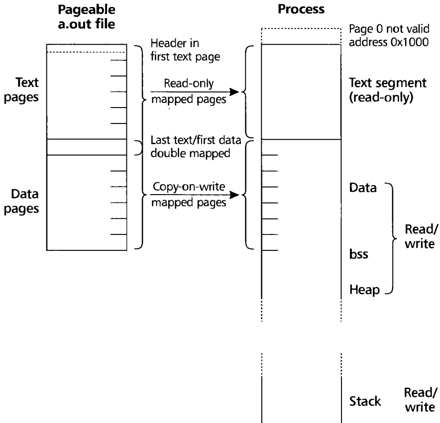
FIGURE 3.5 • Mapping a compact QMAGIC a.out into a process.
