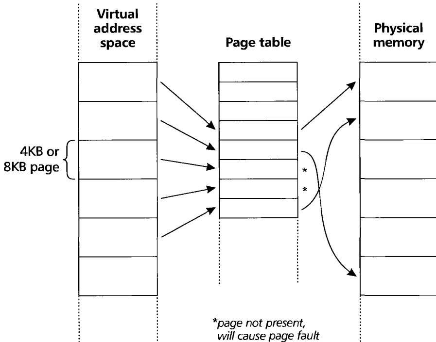
FIGURE 2.7 • Page mapping.
