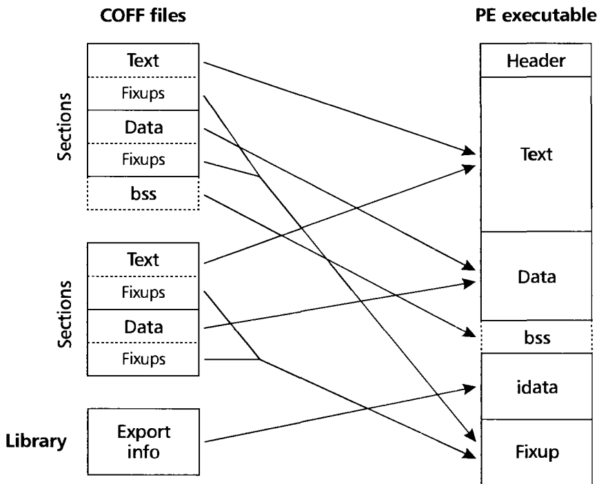
FIGURE 4.10 • PE storage allocation.
