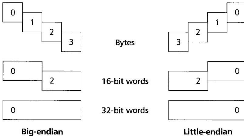
FIGURE 2.1 • Byte-addressable memory.
