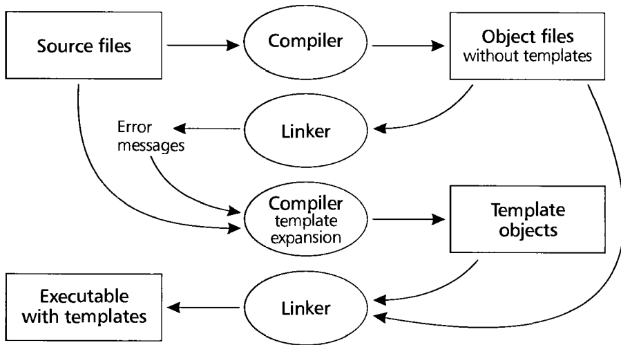
FIGURE 11.1 • Trial linking.
