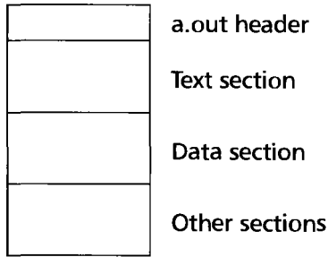
FIGURE 3.1 • Simplified a.out.
