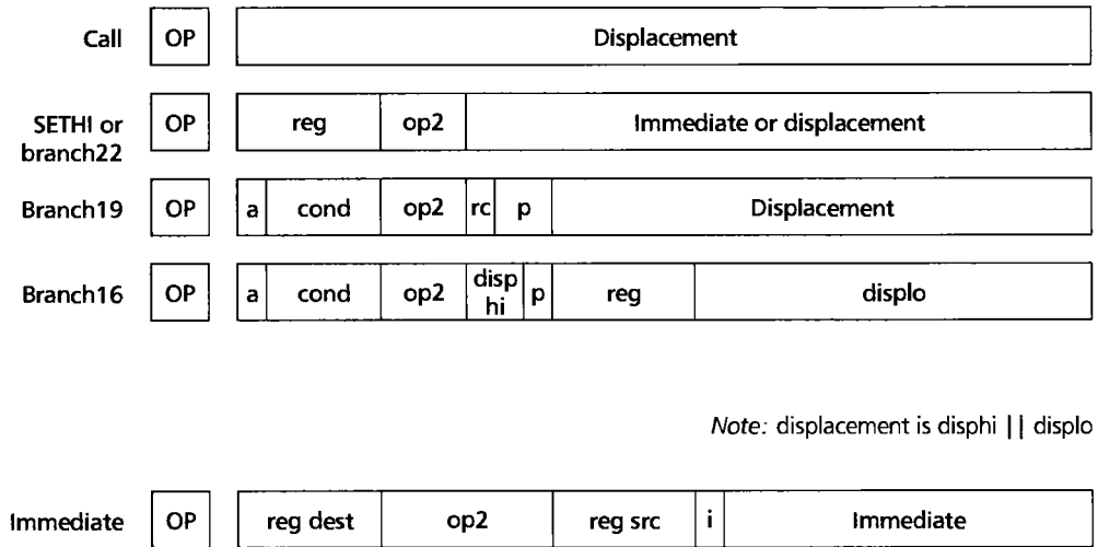
FIGURE 2.5 • SPARC.
