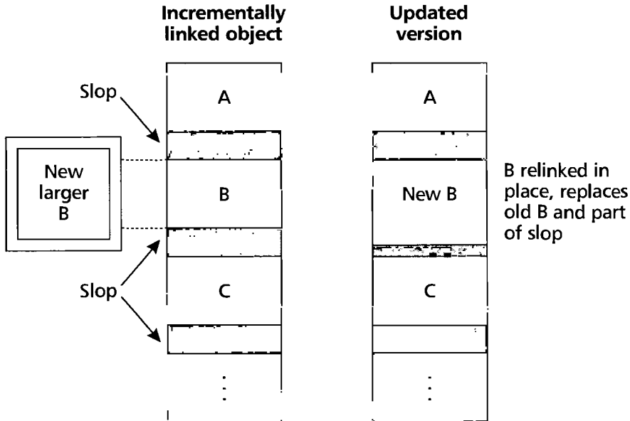
FIGURE 11.3 • Incremental linking.
