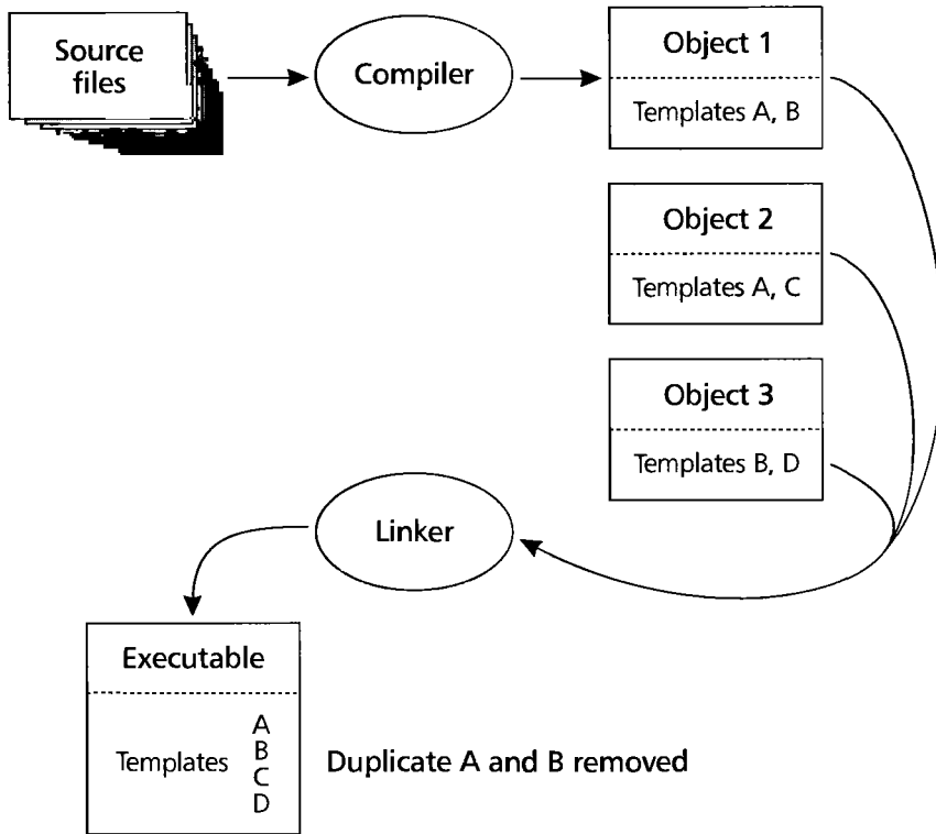
FIGURE 11.2 • Duplicate elimination.
