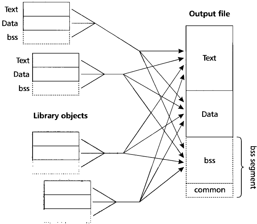
FIGURE 4.8 • a.out linking.
