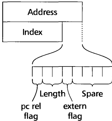
FIGURE 3.8 • Relocation entry format.
