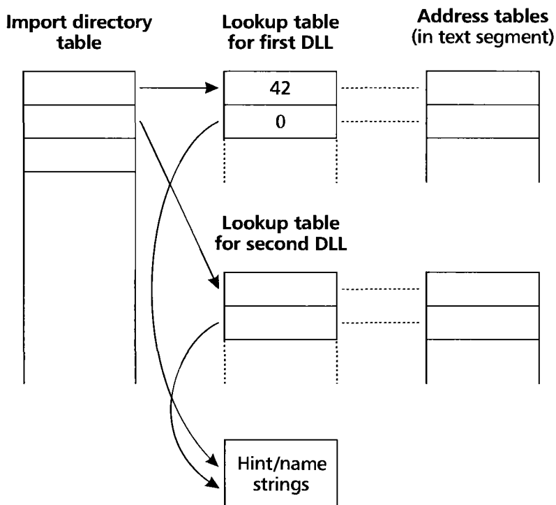
FIGURE 10.6 • Structure of .idata section.
