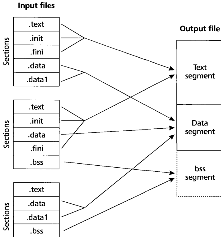
FIGURE 4.9 • ELF linking.
