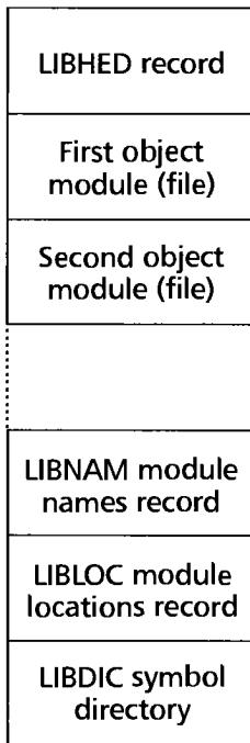
FIGURE 6.5 • OMF libraries.
