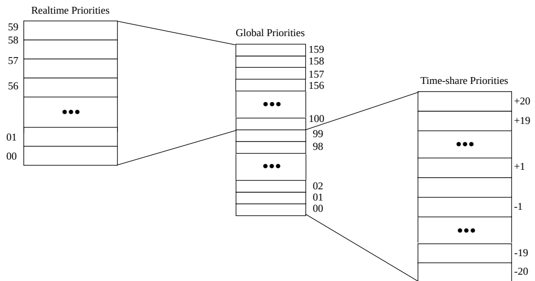
Figure 7-5 The Kernel Dispatch Queue
