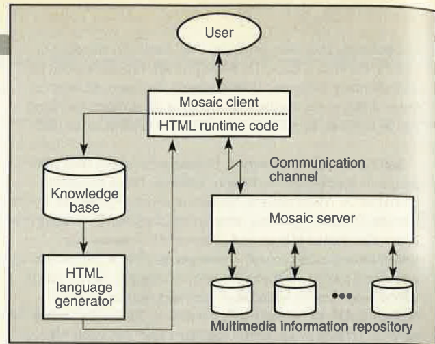
Figure 3. Mosaic extension model. An intelligent agent monitors user preferences to create a knowledge base that dynamically filters the hyperlinks presented to the user.
