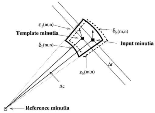
Fig. 14. Bounding box and its adjustment.
