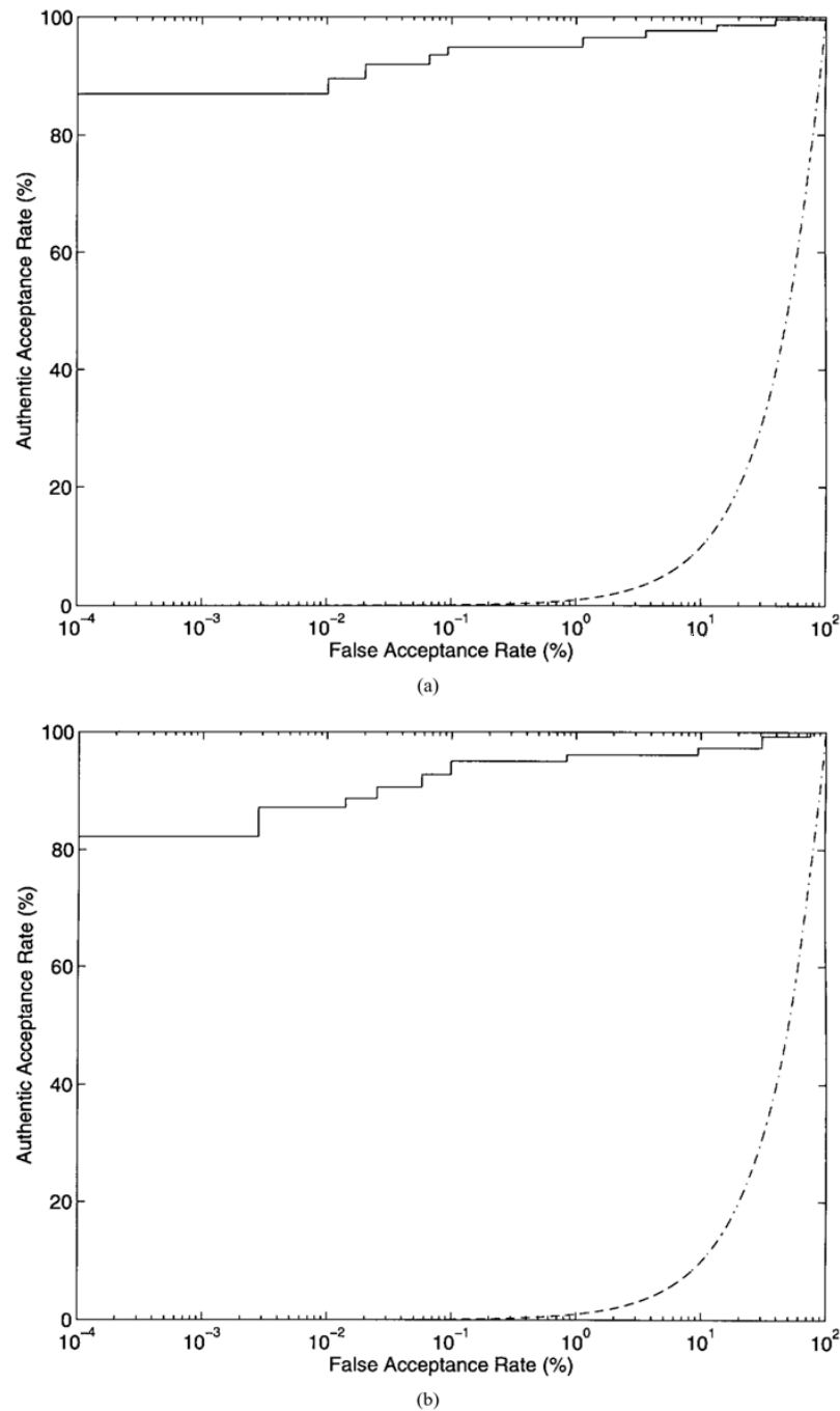
Fig. 20. ROC. (a) MSU data base. (b) NIST 9 (CD no. 1).
