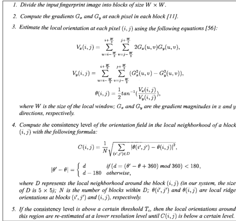
Fig. 8. Hierarchical orientation-field estimation algorithm.
