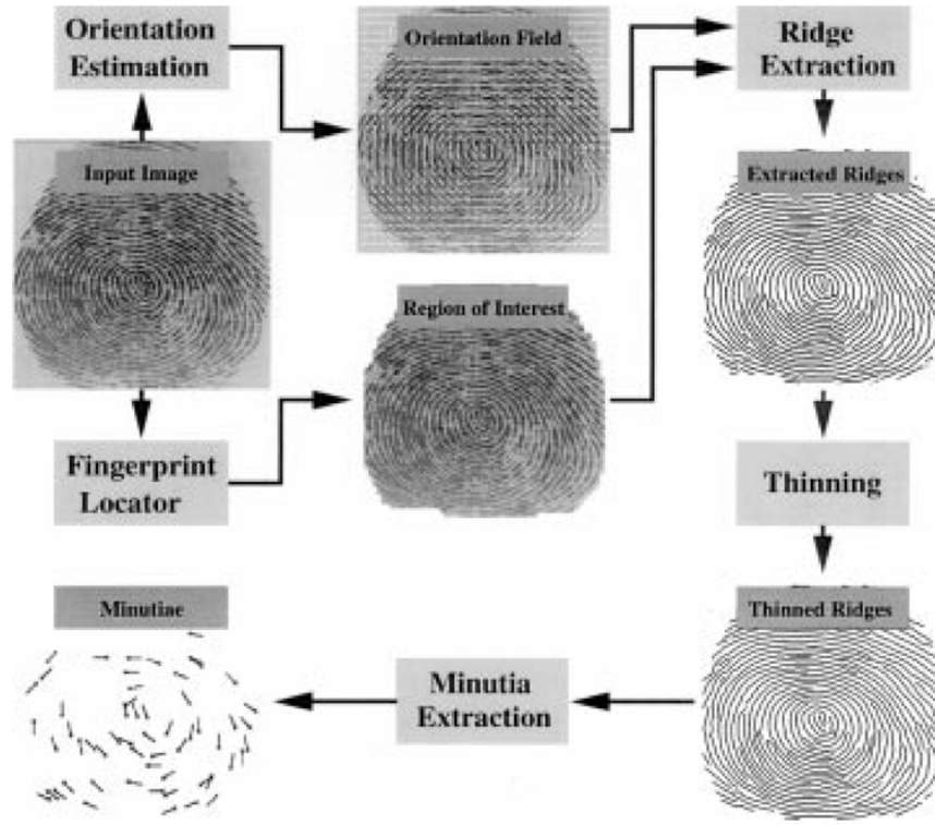
Fig. 7. Flowchart of the minutiae-extraction algorithm.
