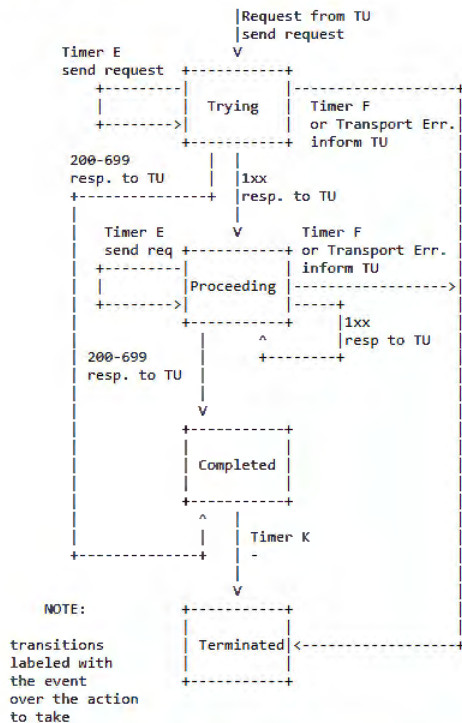
Figure 6: non-INVITE client transaction
