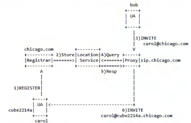
Figure 2: REGISTER example
