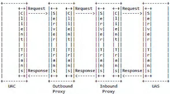
Figure 4: Transaction relationships
