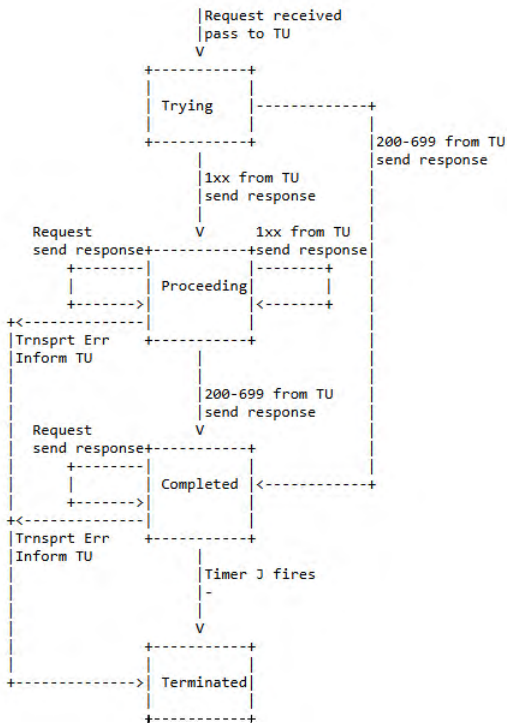
Figure 8: non-INVITE server transaction
