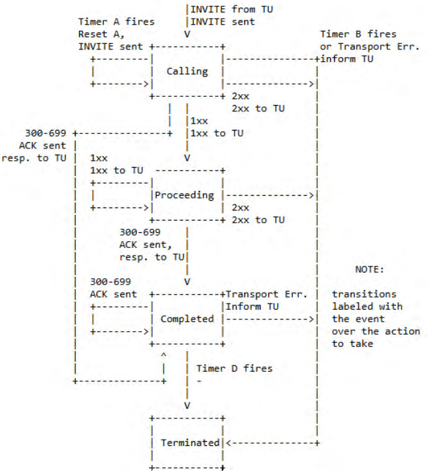
Figure 5: INVITE client transaction
