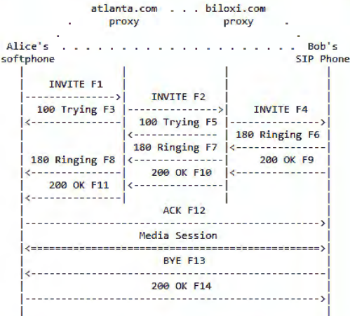
Figure 1: SIP session setup example with SIP trapezoid
