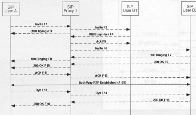
FIGURE B CALL FORWARD ON BUSY
