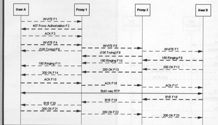
FIGURE A BASIC CALL FLOW
