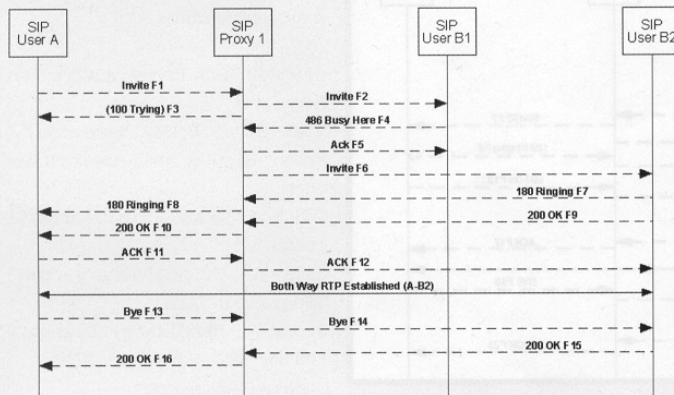
FIGURE B CALL FORWARD ON BUSY
