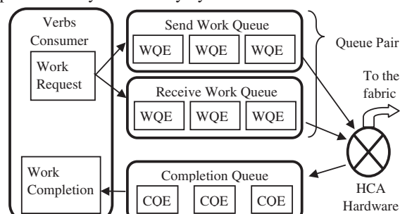
Fig. 1: Infiniband queuing model
