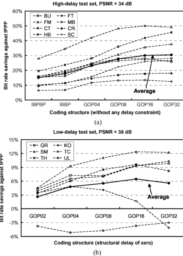
Fig. 3. Bit-rate savings for various hierarchical prediction structures relative to IPPP coding. (a) Simulations without any delay constraint for the high-delay test set (see Table I). (b) Simulations with a structural delay of zero for the low-delay test set (see Table II).
