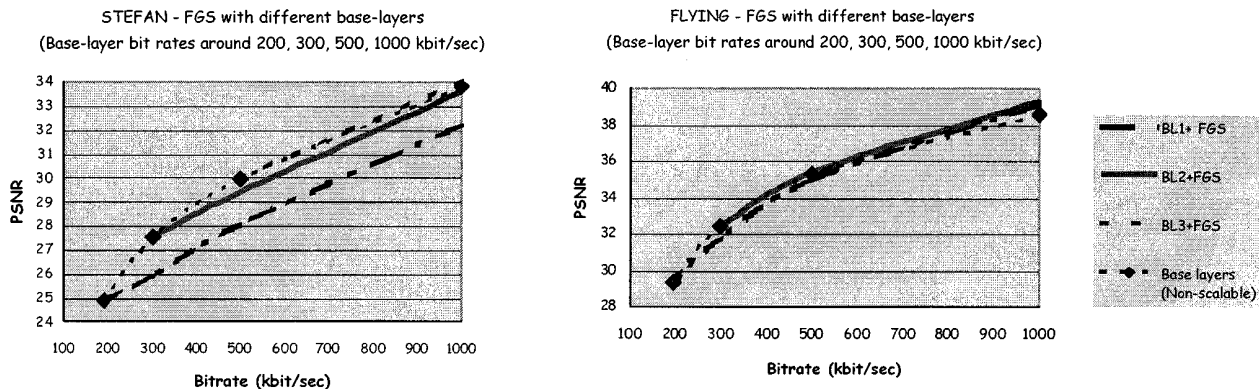
Fig. 8. FGS performance in comparison with multiple nonscalable streams’ (ideal) case. The left figure shows the results for a sequence that exhibits a high-degree of temporal correlation among successive frames. For this type of sequences, FGS pay penalty in performance due to the absence of motion compensation within the enhancement-layer. The right figure shows the performance for a sequence with very-high motion and a large number of scene cuts. For this type of sequences, FGS performance is either similar to or even slightly better than the ideal nonscalable case.
