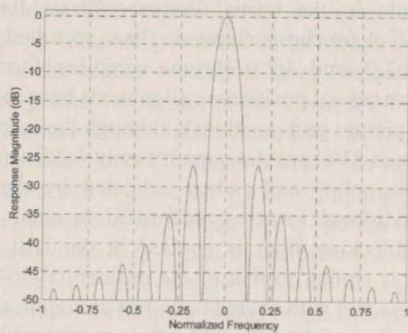
Fig. 3. Frequency response of the poly-phase filter for chroma up-sampling. The filter is used for up-sampling reconstructed chroma values from a reference layer to an enhancement layer for an I BL macroblock.
