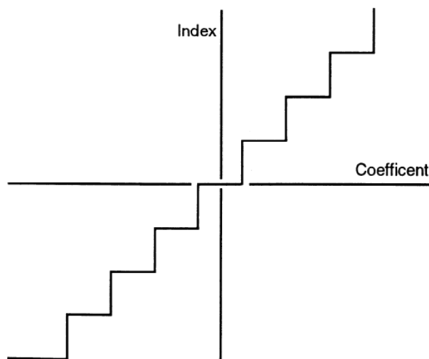
Figure D.29. -- Uniform quantizer characteristics
