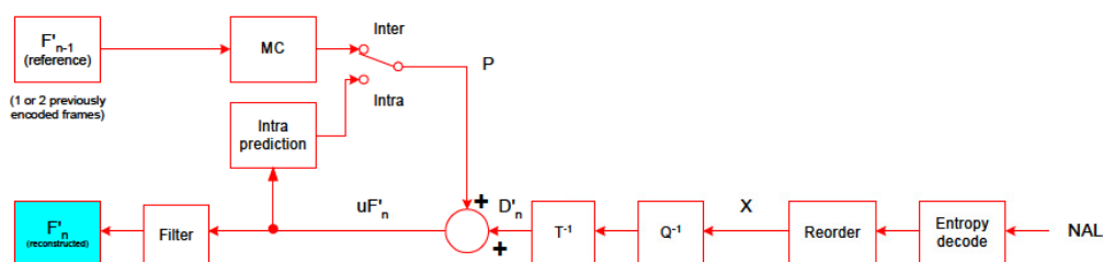
Figure 2-2 AVC Decoder
