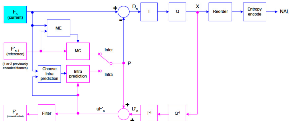
Figure 2-1 AVC Encoder
