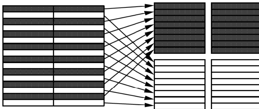
Figure 6-12 — Luminance macroblock structure in field DCT coding
