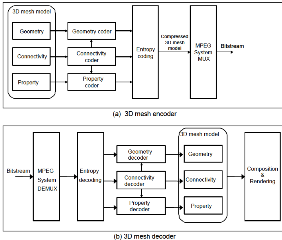
Figure 0-4 — General block diagram of the 3D mesh compressor
