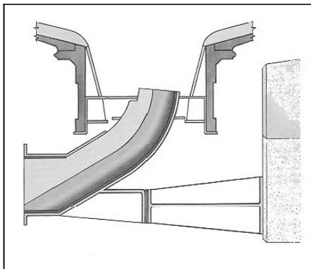
Chute or Spout Feeder
